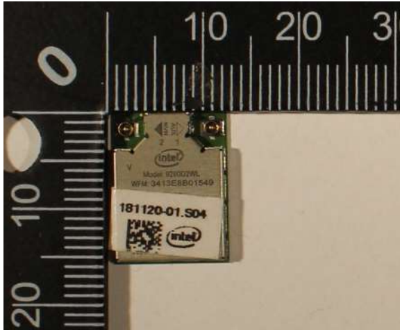
Adapter Front
