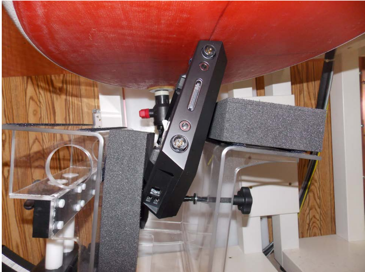
Test Position Side 1,3 Side View 0 mm Gap
