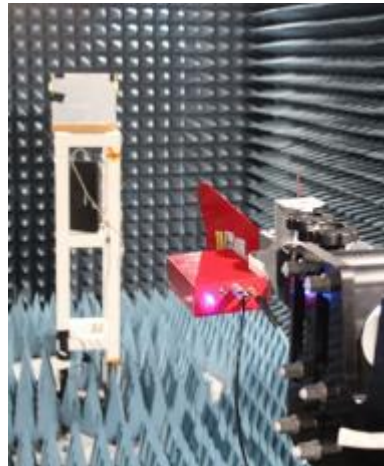
Radiated Setup-2 1 GHz – 18 GHz
