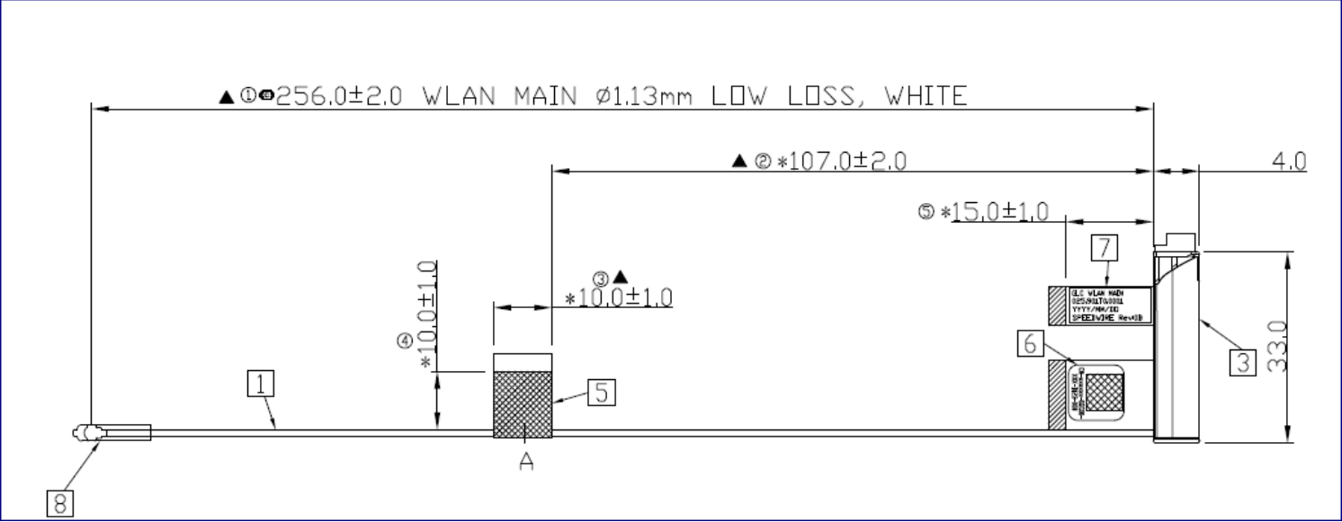
Main Antenna Dimensioned Drawing:
