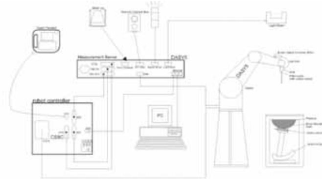
Fig 1. The microwave circuit arrangement used for SAR system verification
