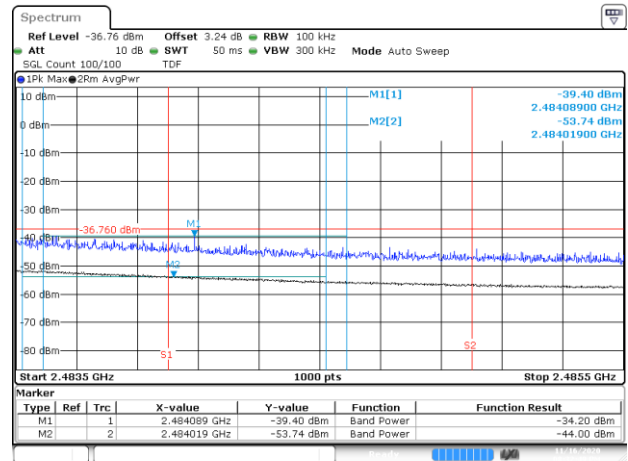
BE-R-HIGH-2MHz, DIV-1, 802.11ax20-HE0, Ch12
