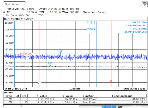
BE-R-HIGH-2MHz, DIV-1, 802.11ax20-HE0, Ch13
