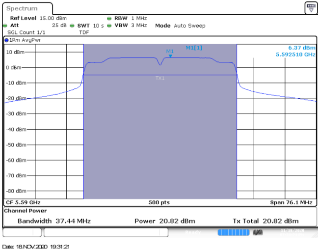
Channel 118
