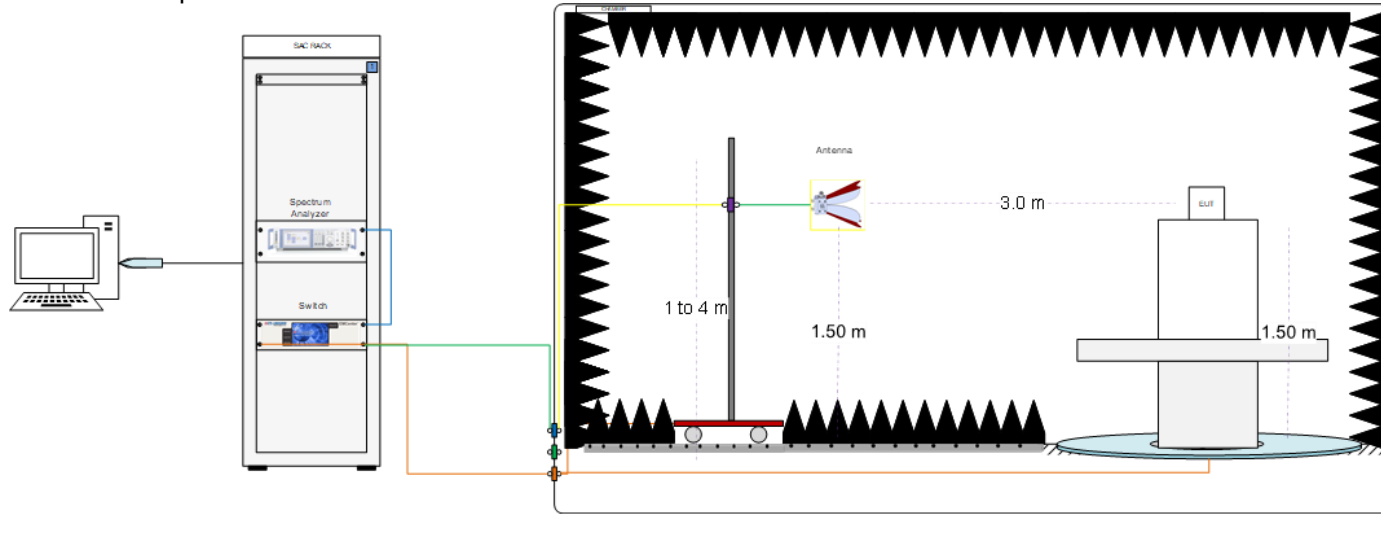
Radiated Setup 1 GHz – 6.4 GHz
