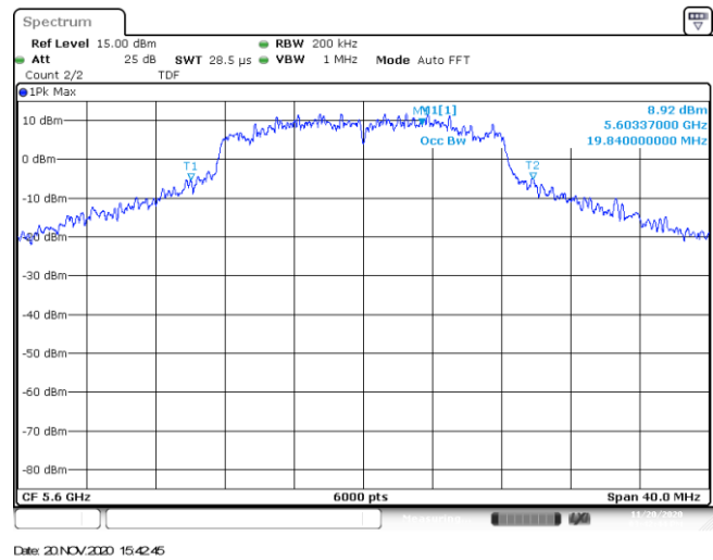
Channel 120
