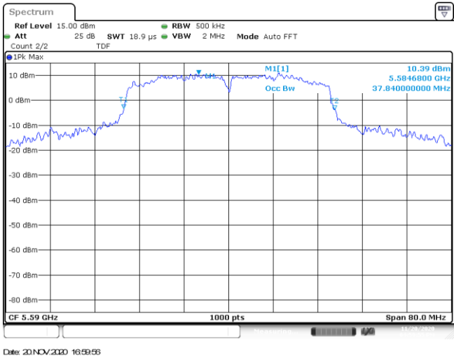
Channel 118
