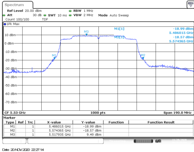
Channel 106
