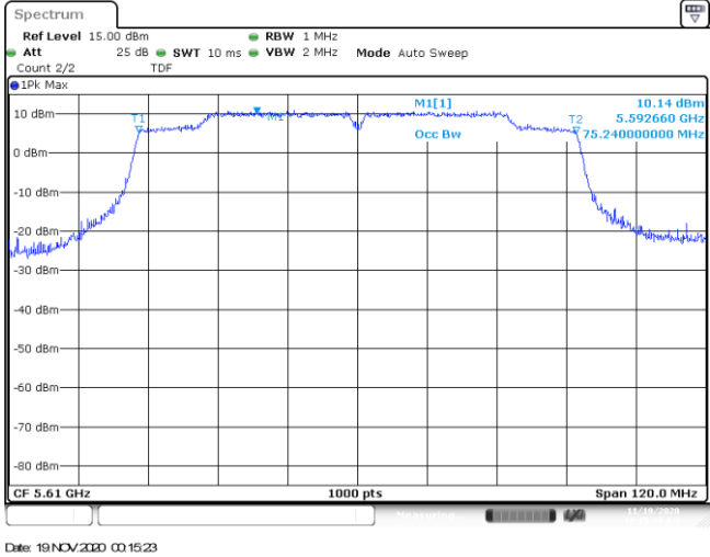
Channel 122
