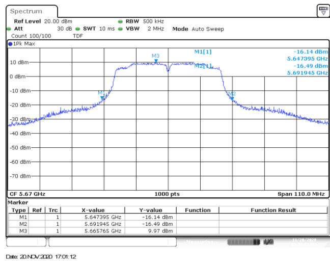
Channel 134
