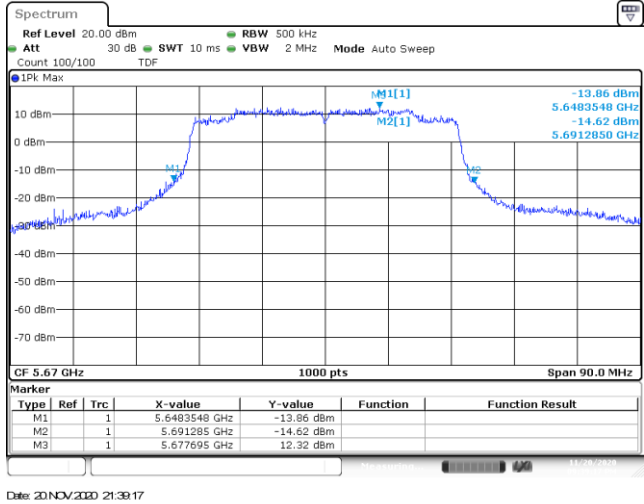
Channel 134
