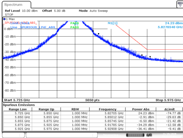
BE-NR-HIGH, DIV-1, 802.11n20-HT0, Ch165
