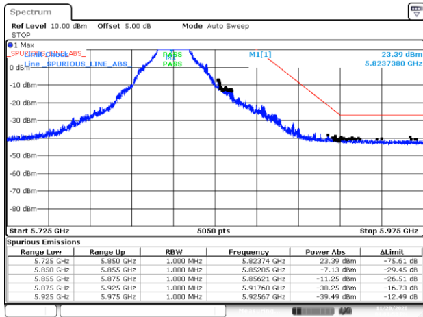
BE-NR-HIGH, DIV-2, 802.11a-6Mbps, Ch165
