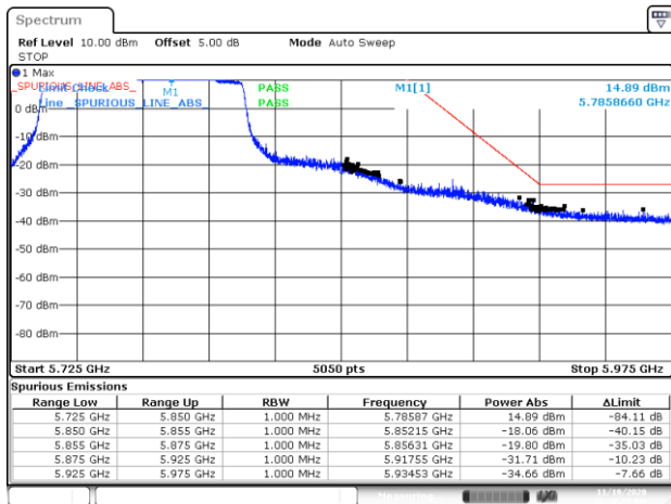
BE-NR-HIGH, DIV-1, 802.11ac80-VHT0, Ch155
