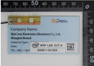
Aux Antenna
