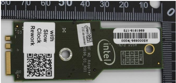
Aux Antenna
