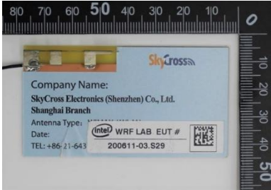
Aux Antenna
