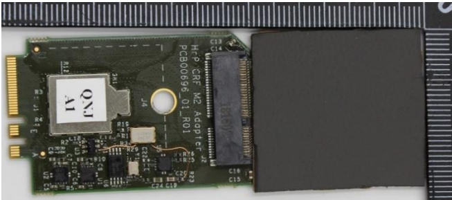
Main Antenna
