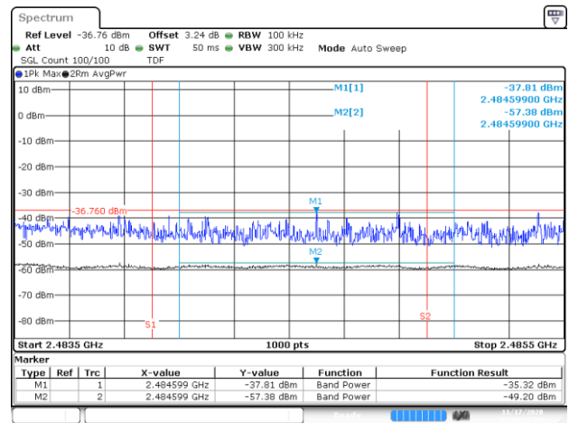
BE-R-HIGH-2MHz, DIV-1, 802.11n20-HT0, Ch13
