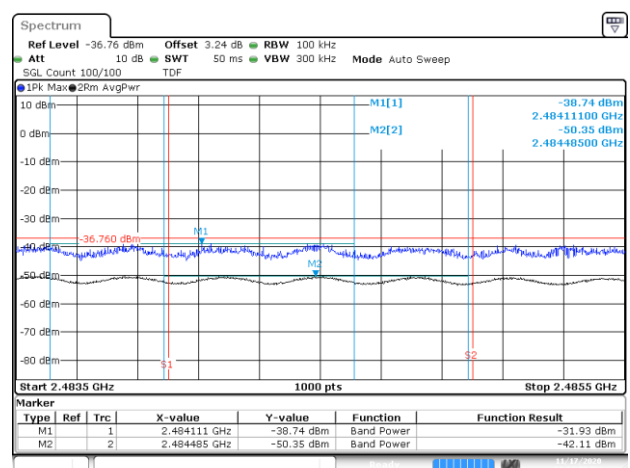
BE-R-HIGH-2MHz, DIV-1, 802.11n40-HT0, Ch9
