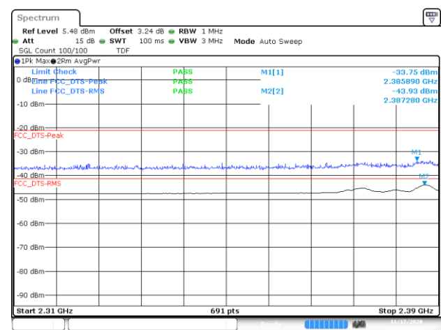
BE-R-LOW, DIV-1, 802.11b-1Mbps, Ch1
