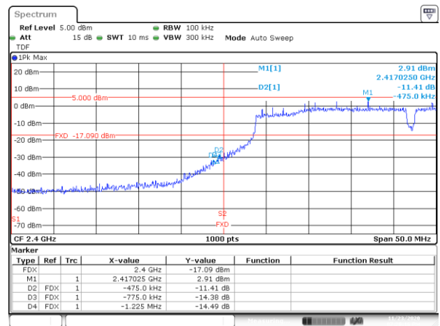
BE-NR, DIV-1, 802.11n40-HT0, Ch3
