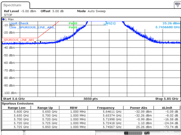
BE-NR-LOW, DIV 2, 802.11ax20-HE0, Ch149
