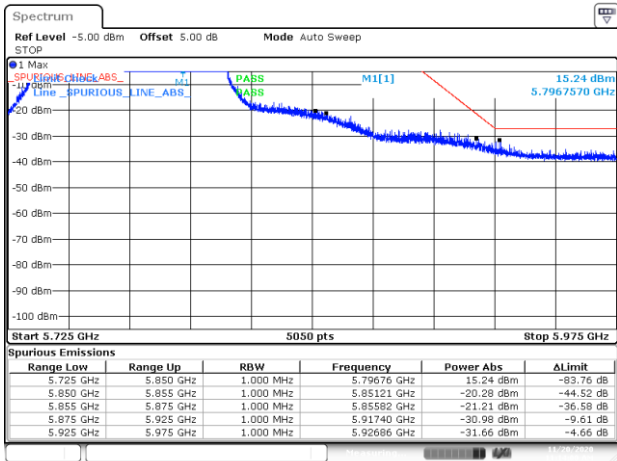
BE-NR-HIGH, DIV 2, 802.11ac80-VHT0, Ch155
