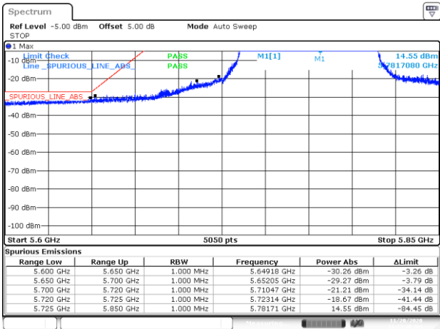
BE-NR-LOW, DIV 2, 802.11ac80-VHT0, Ch155
