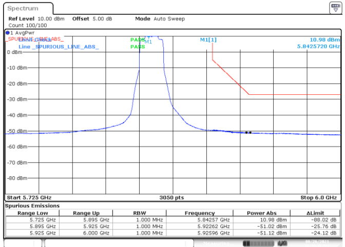
BE-NR-HIGH, SISO-B, 802.11ax20-HE0, Ch169
