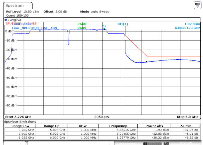
BE-NR-HIGH, SISO-B, 802.11ax160-HE0, Ch163
