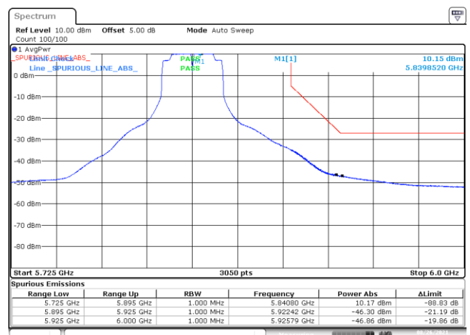
BE-NR-HIGH, MIMO-A, 802.11n40-HT8, Ch167
