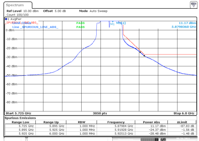
BE-NR-HIGH, SISO-B, 802.11n40-HT0, Ch175
