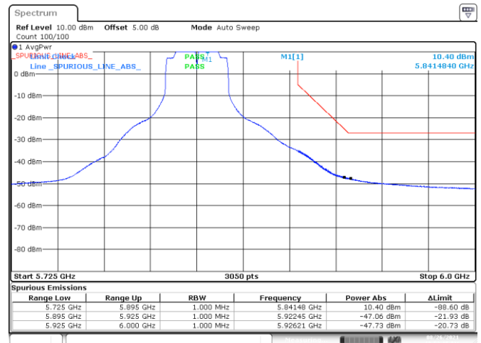
BE-NR-HIGH, MIMO-B, 802.11n40-HT8, Ch167
