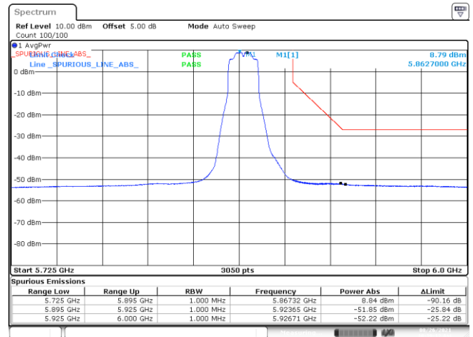
BE-NR-HIGH, MIMO-A, 802.11n20-HT8, Ch173
