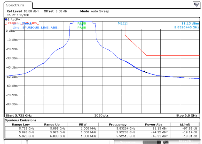
BE-NR-HIGH, SISO-B, 802.11n40-HT0, Ch167
