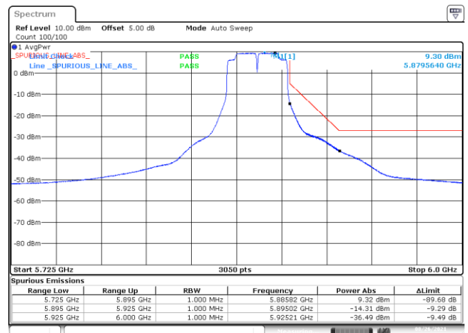
BE-NR-HIGH, MIMO-B, 802.11n40-HT8, Ch175
