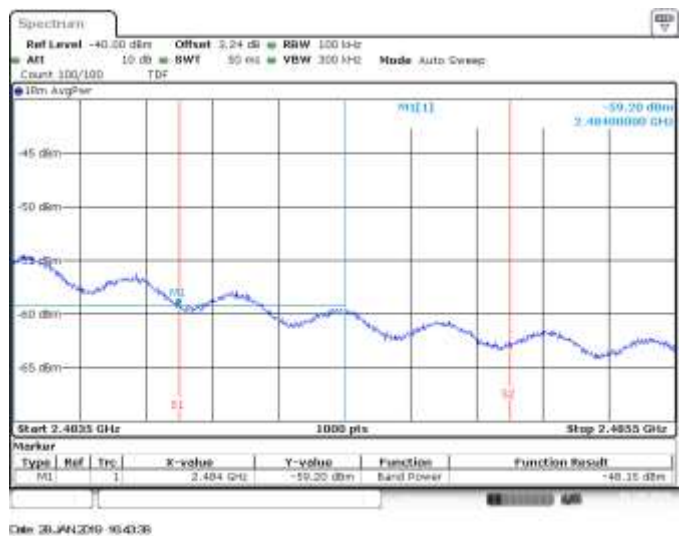
SISO B, CH12, 802.11g, 6Mbps, BE High RMS within 2MHz (Restricted)
