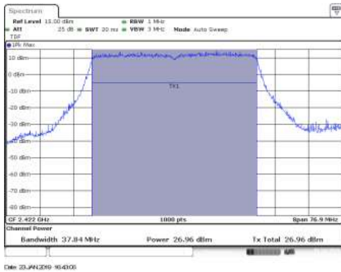
MIMO A, CH3, 802.11ax40, HE0, Power
