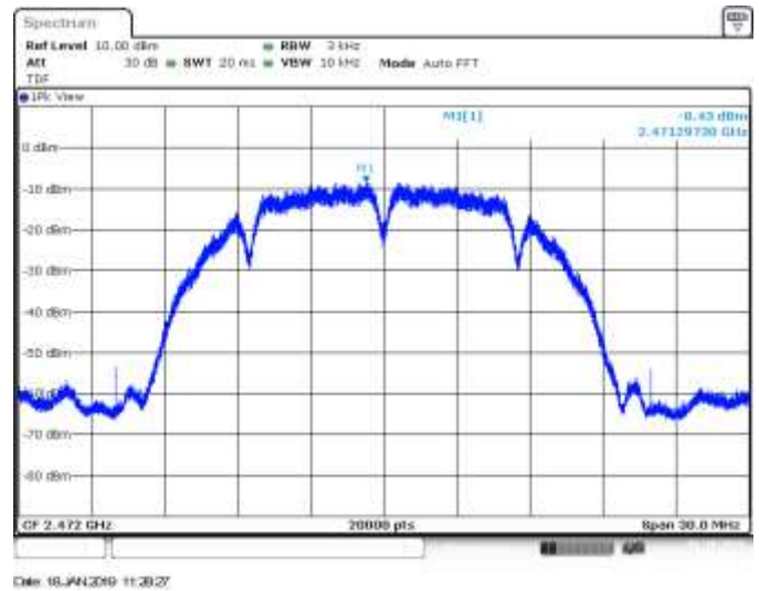
SISO A, CH13, 802.11b, 1Mbps, PSD
