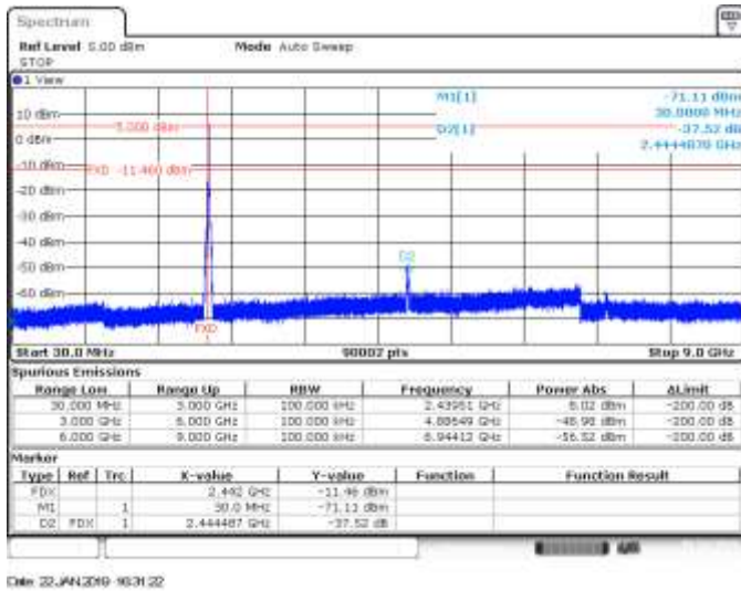
CH7, 802.11ax20, HE0, SISO A, Range 30MHz to 9GHz - Delta Marker Measurement
