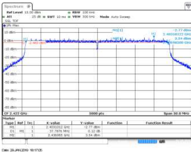
SISO B, CH3, 802.11ax40, HE0, 6dB Occupied Bandwidth
