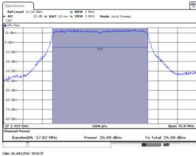
MIMO B, CH3, 802.11ax40, HE0, Power
