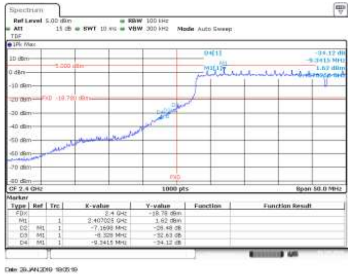
MIMO B, CH3, 802.11ax40, HE0, BE Low (Non Restricted)
