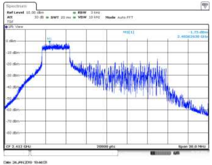
MIMO B, CH1, 802.11ax20_R52_37, HE0, PSD
