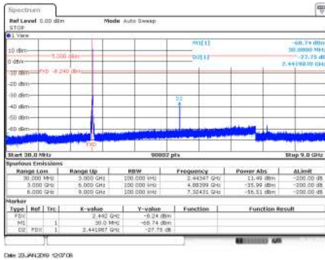
CH7, 802.11b, 1Mbps, SISO A, Range 30MHz to 9GHz - Delta Marker Measurement
