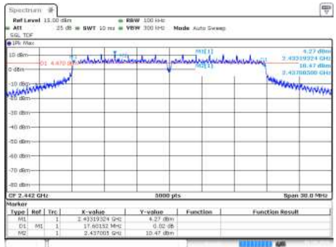
SISO A, CH7, 802.11g, 6Mbps, 99% Occupied Bandwidth
