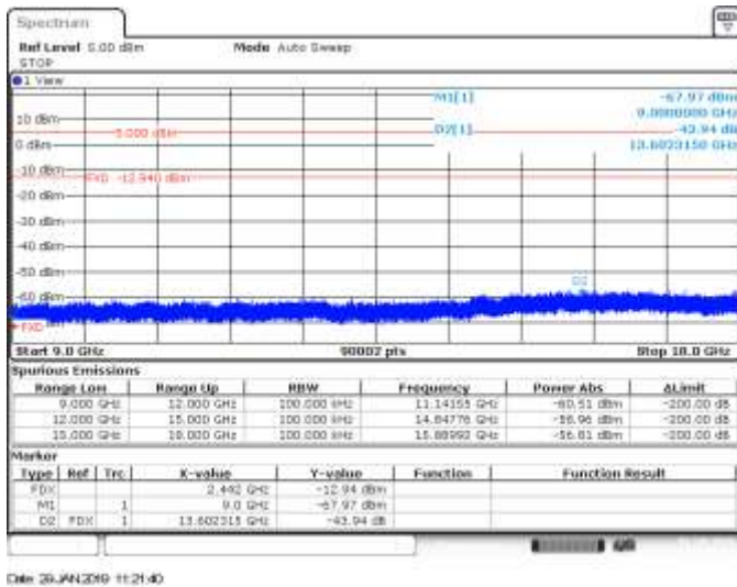
CH7, 802.11n20, HT8, MIMO B, Range 9GHz to 18GHz - Delta Marker Measurement
