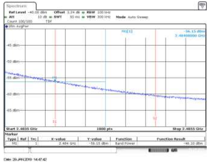
SISO B, CH12, 802.11ax20, HE0, BE High RMS within 2MHz (Restricted)
