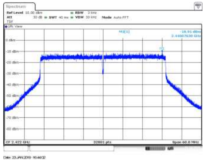
MIMO A, CH3, 802.11ax40, HE0, PSD
