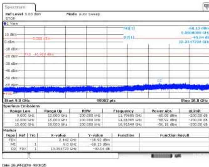
CH7, 802.11n40, HT0, SISO B, Range 9GHz to 18GHz - Delta Marker Measurement
