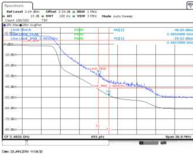
MIMO A, CH10, 802.11n40, HT8, BE High (Restricted)
