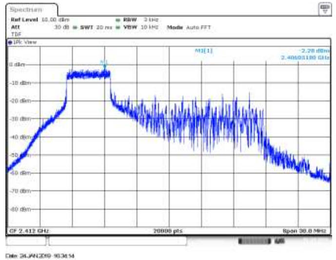
MIMO A, CH1, 802.11ax20_R52_37, HE0, PSD
