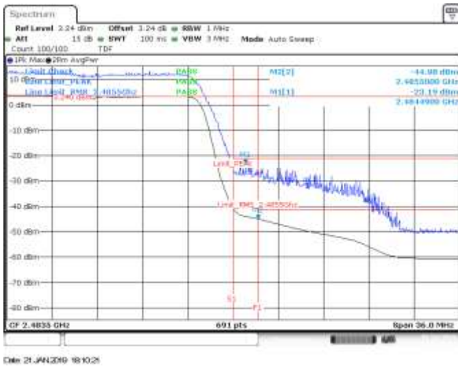
SISO A, CH13, 802.11n20, HT0, BE High (Restricted)
