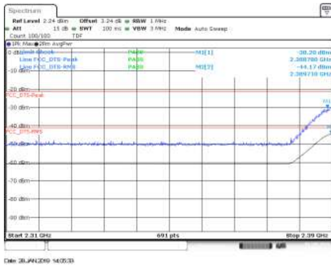
SISO B, CH1, 802.11g, 6Mbps, BE Low
