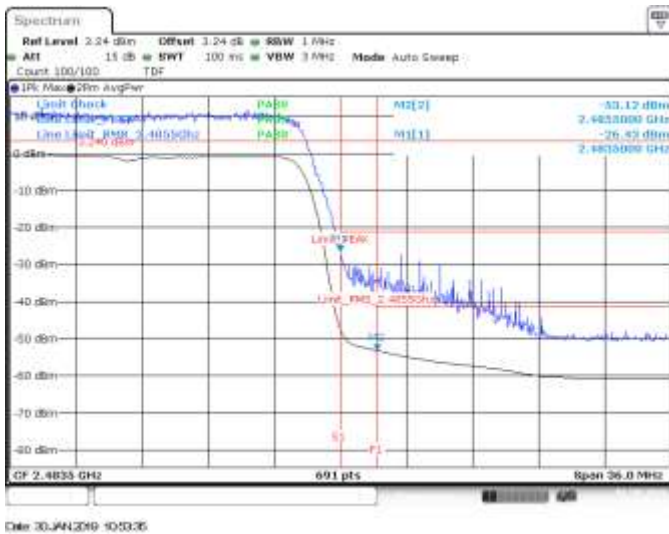
MIMO A, CH13, 802.11ax20, HE0, BE High (Restricted)
