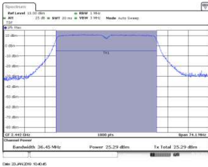
MIMO A, CH7, 802.11n40, HT8, Power
