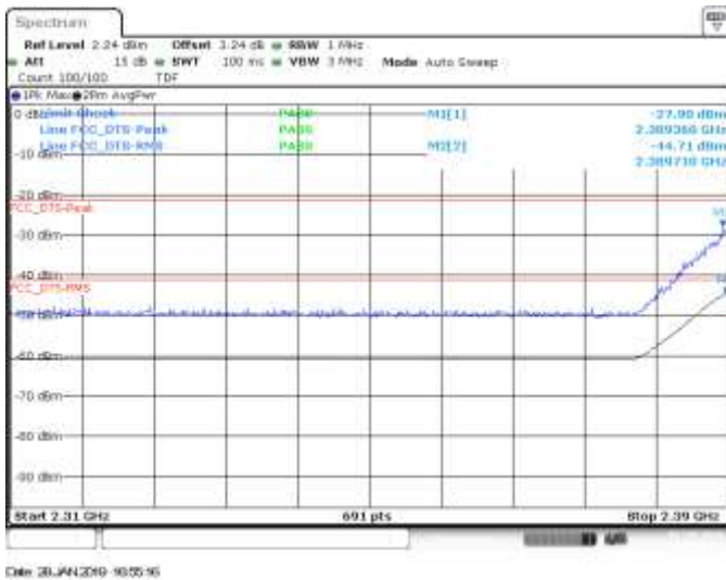
SISO B, CH1, 802.11n20, HT0, BE Low
