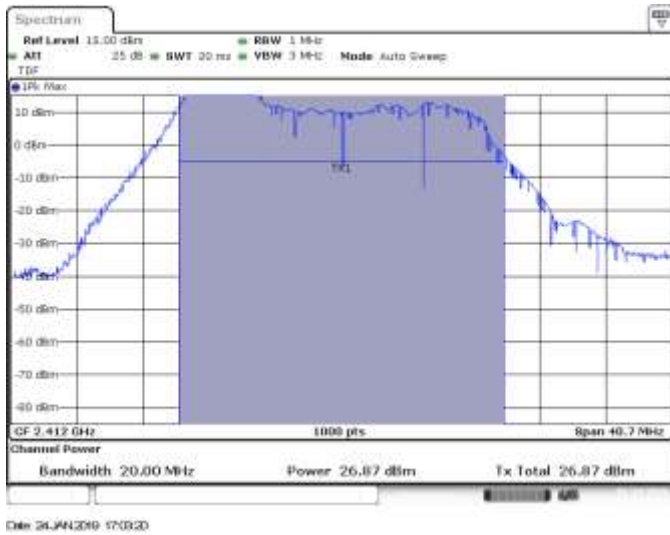
MIMO A, CH1, 802.11ax20_R52_37, HE0, Power
