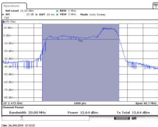
SISO A, CH13, 802.11ax20_R52_40, HE0, Power
