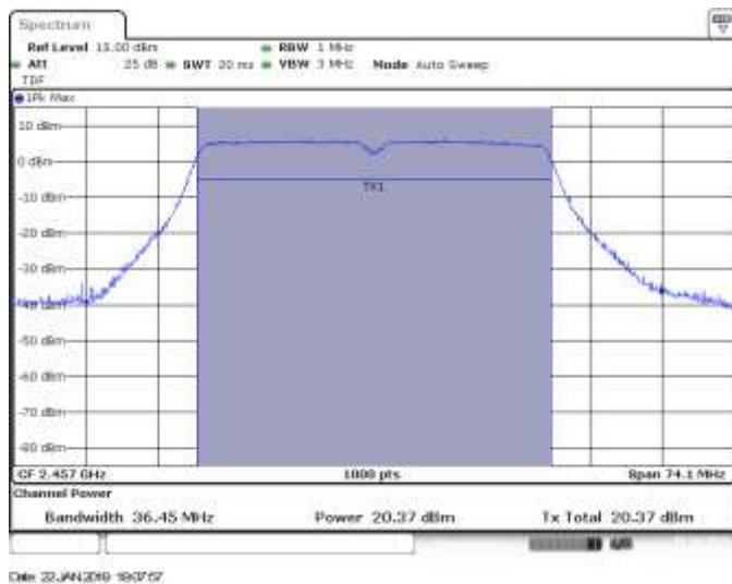
SISO A, CH10, 802.11n40, HT0, Power
