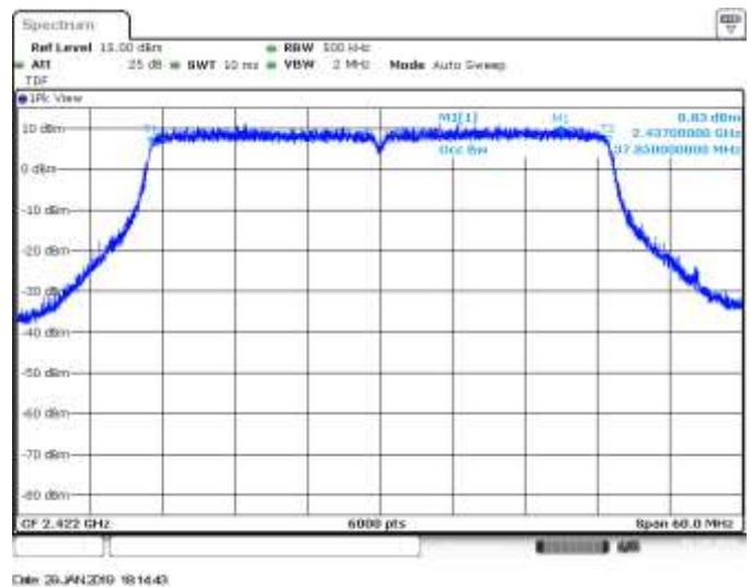
SISO B, CH3, 802.11ax40, HE0, 99% Occupied Bandwidth
