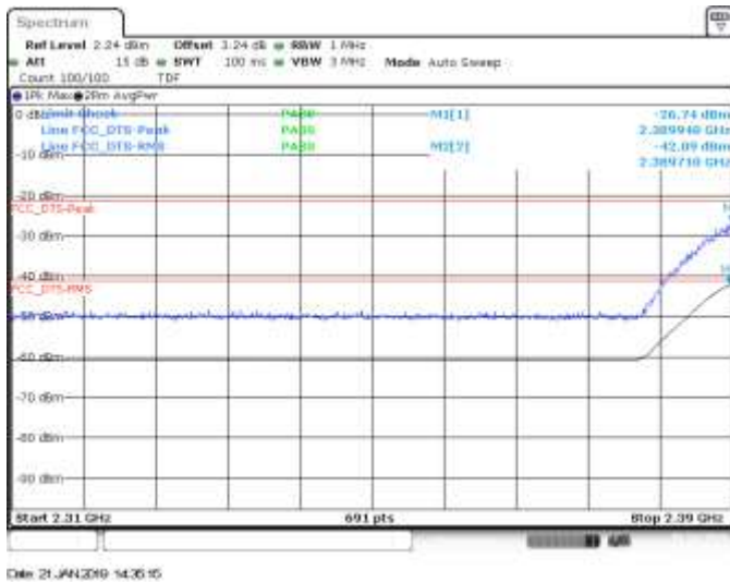
SISO A, CH1, 802.11g, 6Mbps, BE Low
