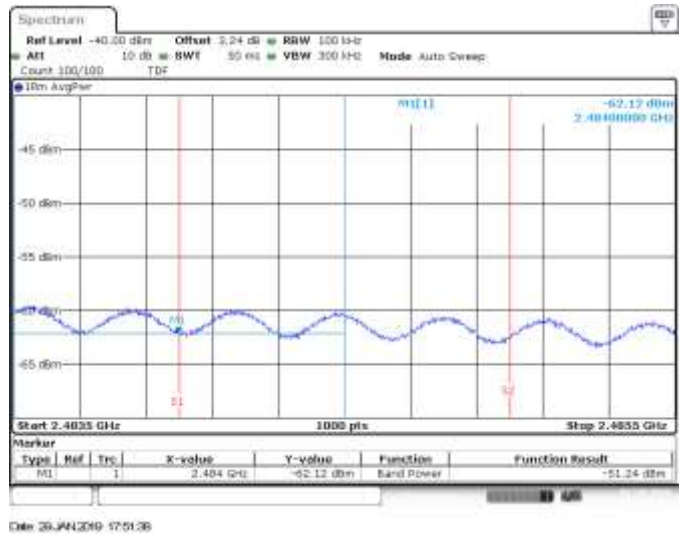
MIMO B, CH9, 802.11n40, HT8, BE High RMS within 2MHz (Restricted)
