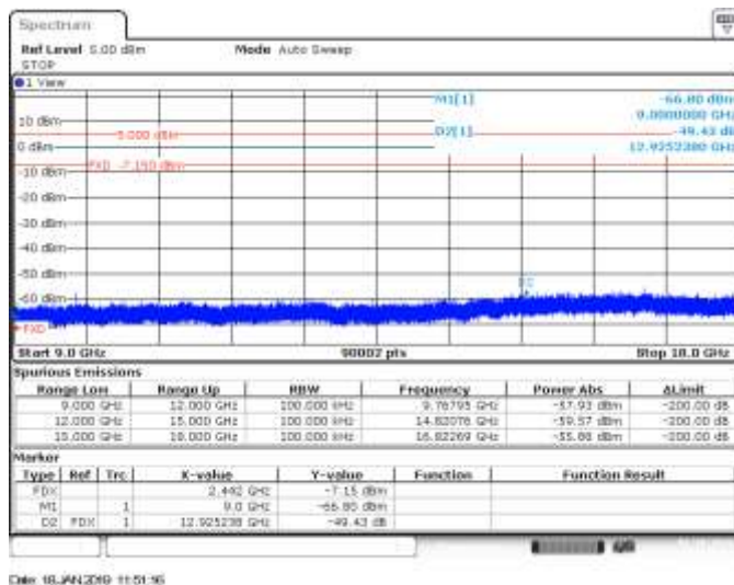
CH7, 802.11b, 1Mbps, SISO B, Range 9GHz to 18GHz - Delta Marker Measurement
