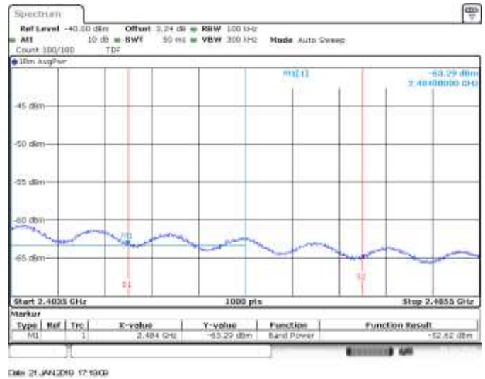
SISO A, CH11, 802.11g, 6Mbps, BE High RMS within 2MHz (Restricted)
