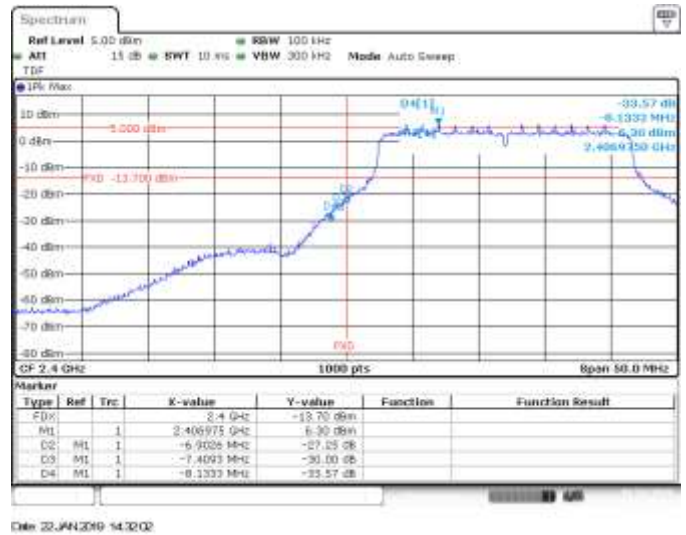
SISO A, CH1, 802.11ax20, HE0, BE Low (Non Restricted)
