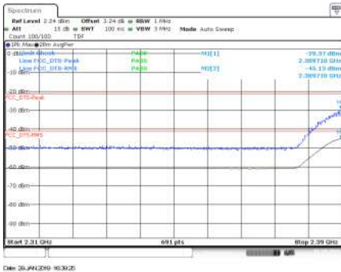
MIMO B, CH3, 802.11n40, HT8, BE Low
