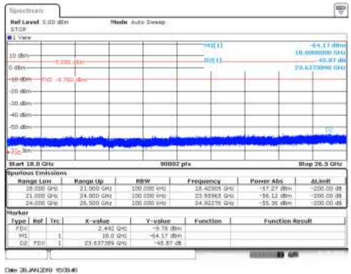
CH7, 802.11g, 6Mbps, SISO B, Range 18GHz to 26.5GHz - Delta Marker Measurement
