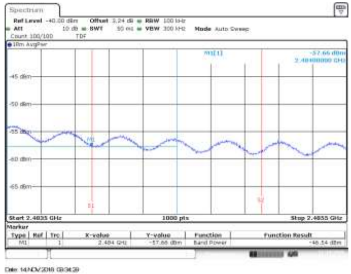
MIMO B, CH12, 802.11n20, HT8, BE High RMS within 2MHz (Restricted)
