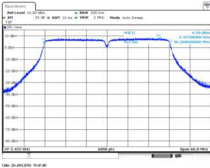
SISO B, CH3, 802.11n40, HT0, 99% Occupied Bandwidth
