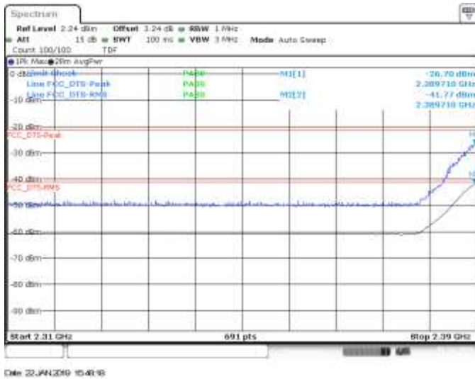
SISO A, CH1, 802.11ax20, HE0, BE Low
