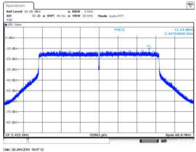
MIMO B, CH3, 802.11ax40, HE0, PSD
