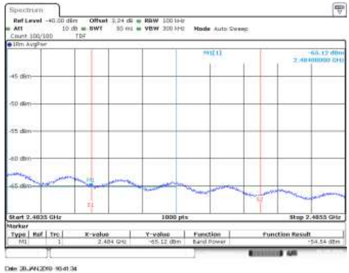
SISO B, CH11, 802.11g, 6Mbps, BE High RMS within 2MHz (Restricted)
