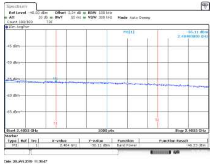
SISO B, CH13, 802.11ax20, HE0, BE High RMS within 2MHz (Restricted)
