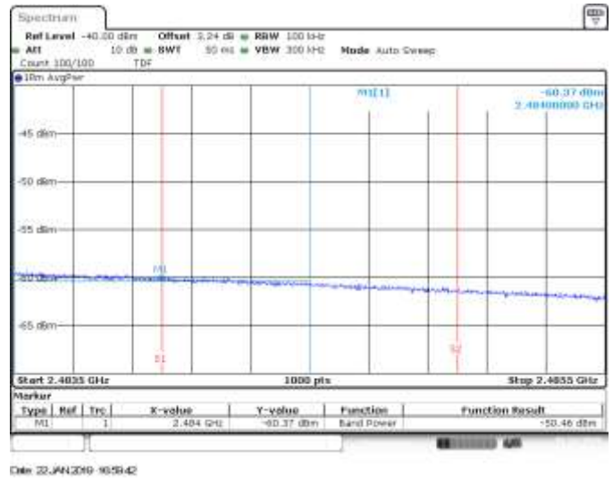
SISO A, CH11, 802.11ax20, HE0, BE High RMS within 2MHz (Restricted)
