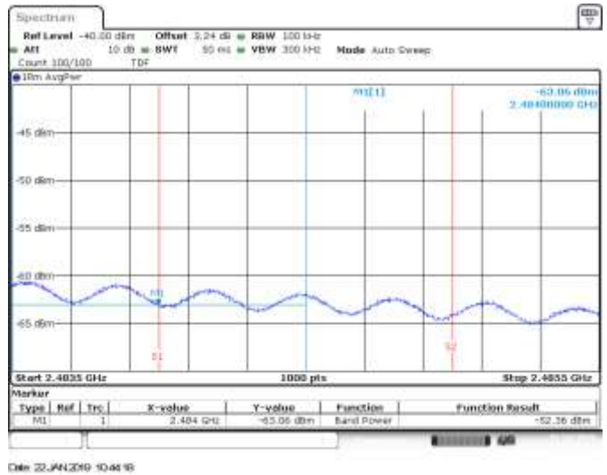
MIMO A, CH11, 802.11n20, HT8, BE High RMS within 2MHz (Restricted)
