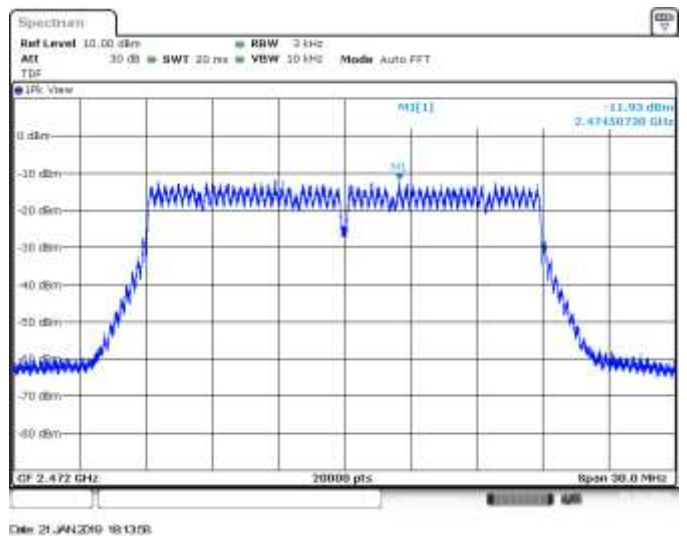
SISO A, CH13, 802.11n20, HT0, PSD
