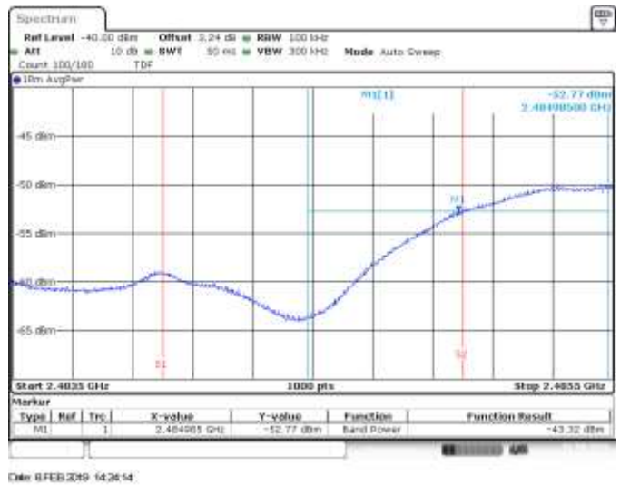
SISO B, CH13, 802.11b, 1Mbps, BE High RMS within 2MHz (Restricted)
