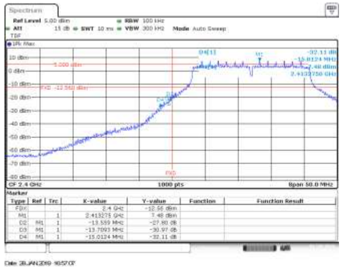
SISO B, CH1, 802.11n20, HT0, BE Low (Non Restricted)
