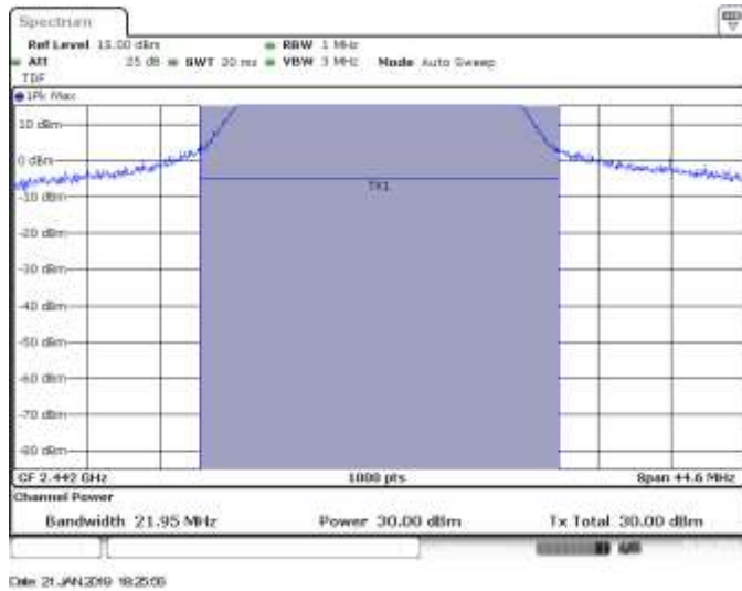
SISO A, CH7, 802.11n20, HT0, Power
