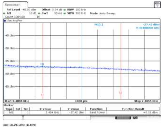
MIMO B, CH13, 802.11ax20, HE0, BE High RMS within 2MHz (Restricted)
