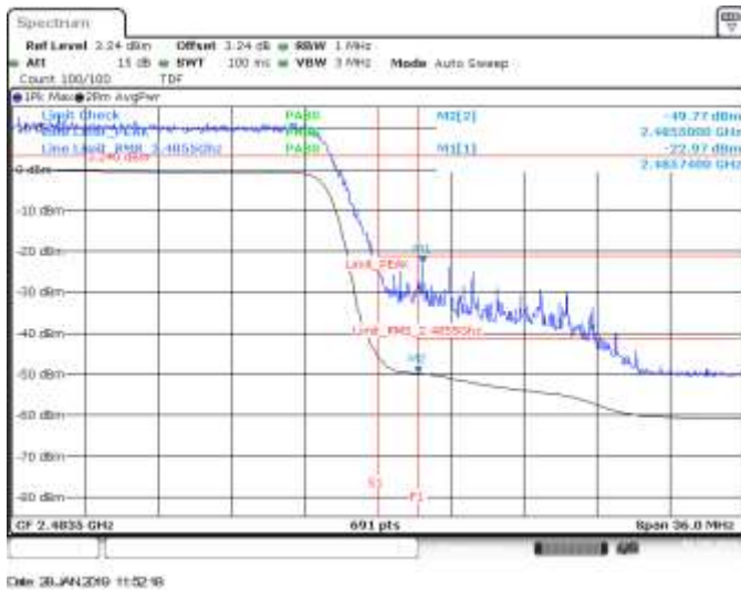
SISO B, CH11, 802.11ax40, HE0, BE High (Restricted)
