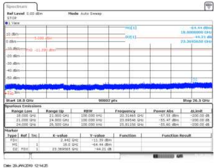
CH7, 802.11ax20, HE0, SISO B, Range 18GHz to 26.5GHz - Delta Marker Measurement
