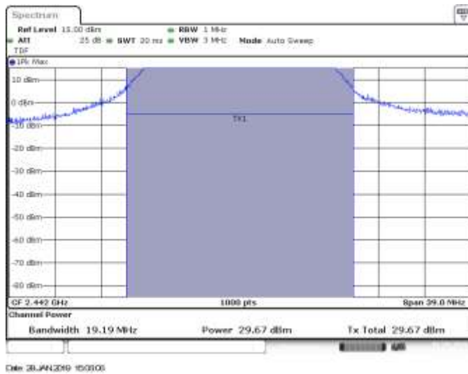
SISO B, CH7, 802.11g, 6Mbps, Power
