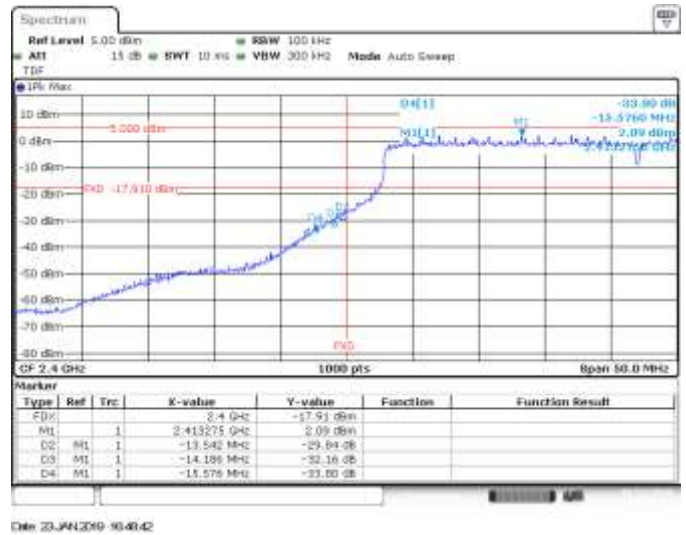
MIMO A, CH3, 802.11ax40, HE0, BE Low (Non Restricted)
