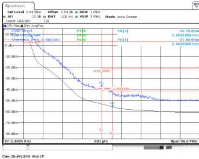
SISO B, CH11, 802.11g, 6Mbps, BE High (Restricted)
