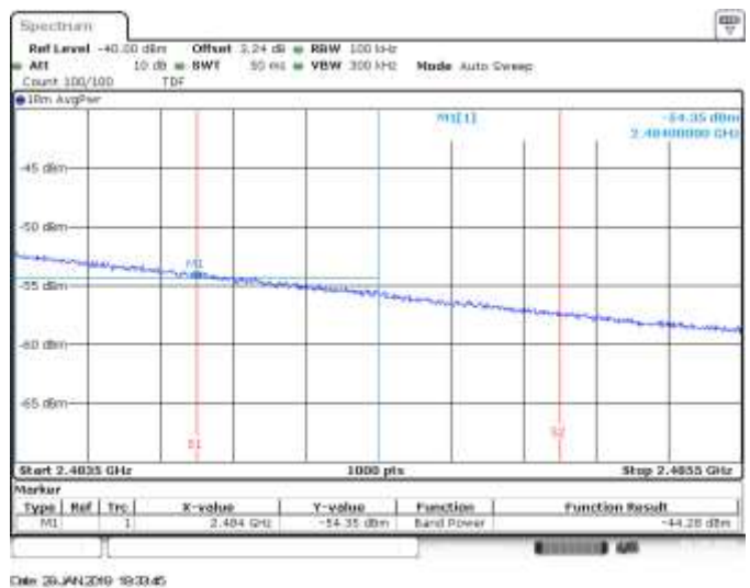
MIMO B, CH10, 802.11ax40, HE0, BE High RMS within 2MHz (Restricted)
