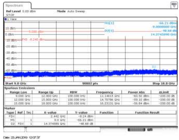
CH7, 802.11b, 1Mbps, SISO A, Range 9GHz to 18GHz - Delta Marker Measurement
