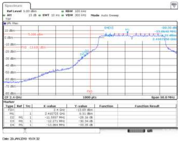
MIMO B, CH1, 802.11ax20, HE0, BE Low (Non Restricted)
