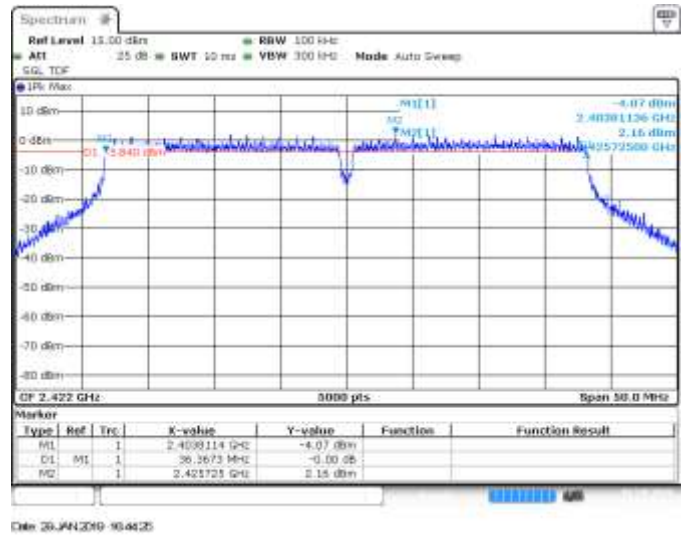
MIMO B, CH3, 802.11n40, HT8, 6dB Occupied Bandwidth
