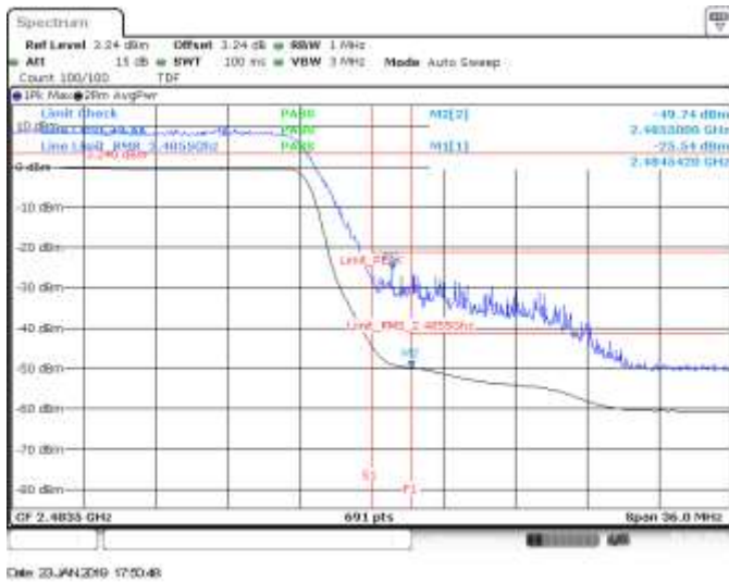
MIMO A, CH11, 802.11n40, HT8, BE High (Restricted)
