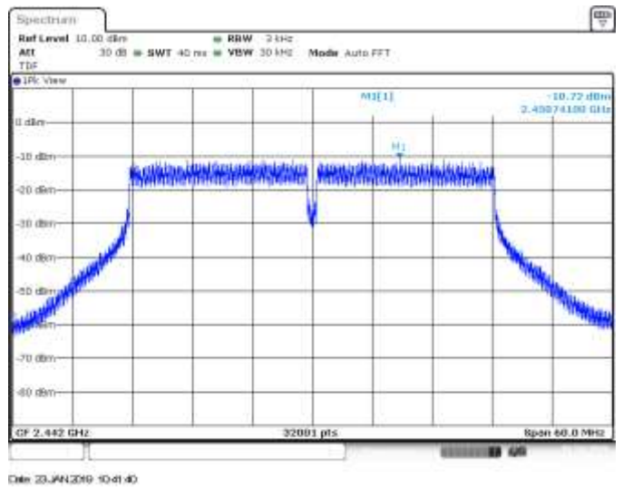
MIMO A, CH7, 802.11n40, HT8, PSD
