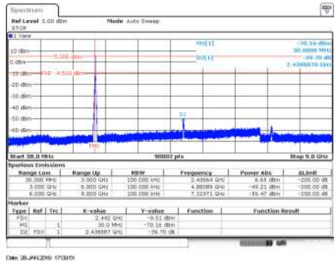
CH7, 802.11n20, HT0, SISO B, Range 30MHz to 9GHz - Delta Marker Measurement
