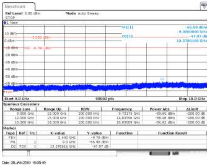
CH7, 802.11g, 6Mbps, SISO B, Range 9GHz to 18GHz - Delta Marker Measurement
