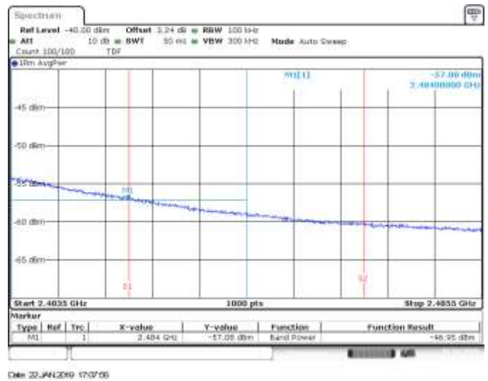
SISO A, CH12, 802.11ax20, HE0, BE High RMS within 2MHz (Restricted)
