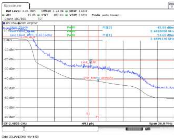
SISO A, CH9, 802.11ax40, HE0, BE High (Restricted)
