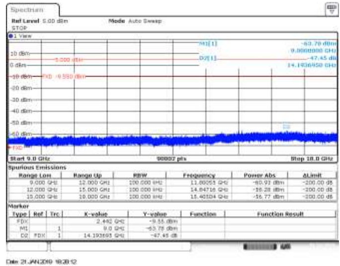
CH7, 802.11n20, HT0, SISO A, Range 9GHz to 18GHz - Delta Marker Measurement
