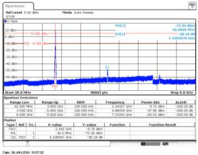
CH7, 802.11g, 6Mbps, SISO B, Range 30MHz to 9GHz - Delta Marker Measurement
