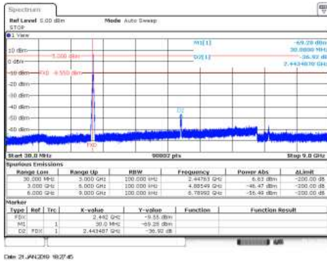
CH7, 802.11n20, HT0, SISO A, Range 30MHz to 9GHz - Delta Marker Measurement
