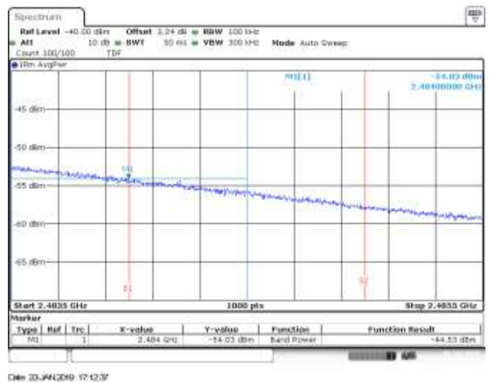
MIMO A, CH10, 802.11ax40, HE0, BE High RMS within 2MHz (Restricted)
