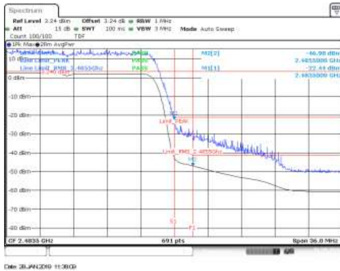
SISO B, CH13, 802.11ax20, HE0, BE High (Restricted)
