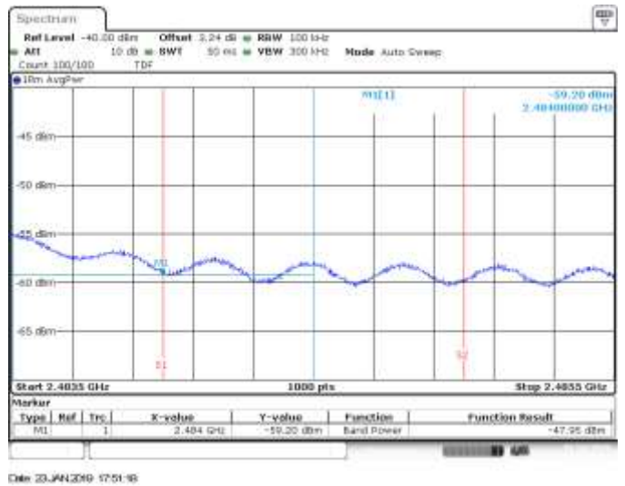
MIMO A, CH11, 802.11n40, HT8, BE High RMS within 2MHz (Restricted)
