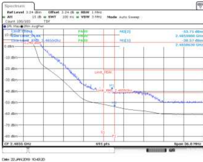
MIMO A, CH11, 802.11n20, HT8, BE High (Restricted)
