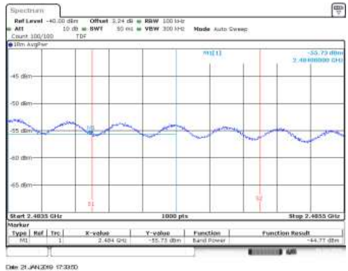
SISO A, CH13, 802.11g, 6Mbps, BE High RMS within 2MHz (Restricted)
