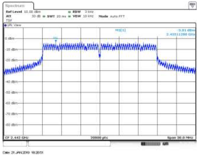
SISO A, CH7, 802.11n20, HT0, PSD
