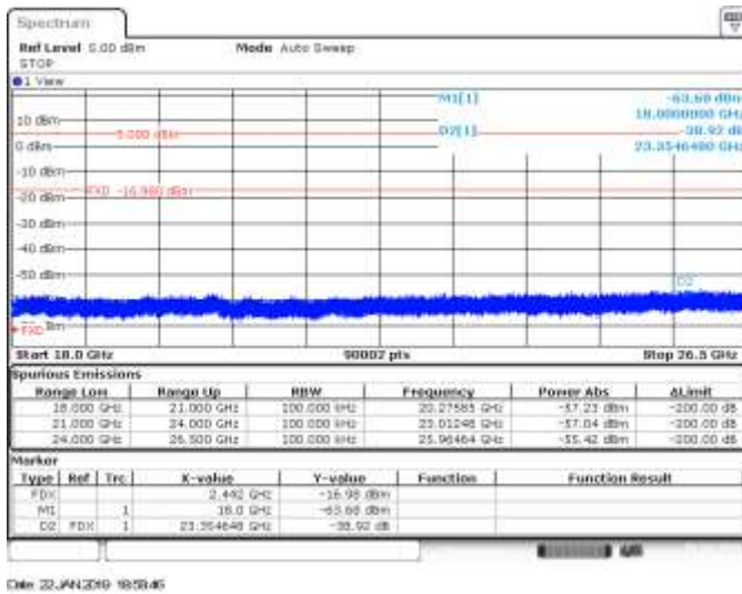
CH7, 802.11n40, HT0, SISO A, Range 18GHz to 26.5GHz - Delta Marker Measurement
