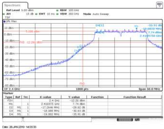
SISO B, CH1, 802.11g, 6Mbps, BE Low (Non Restricted)
