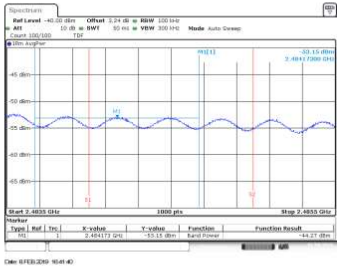
SISO A, CH13, 802.11n20, HT0, BE High RMS within 2MHz (Restricted)
