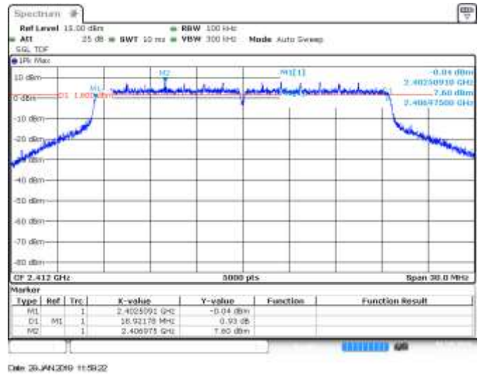
SISO B, CH1, 802.11ax20, HE0, 6dB Occupied Bandwidth
