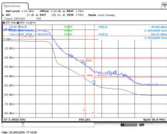
MIMO A, CH10, 802.11ax40, HE0, BE High (Restricted)
