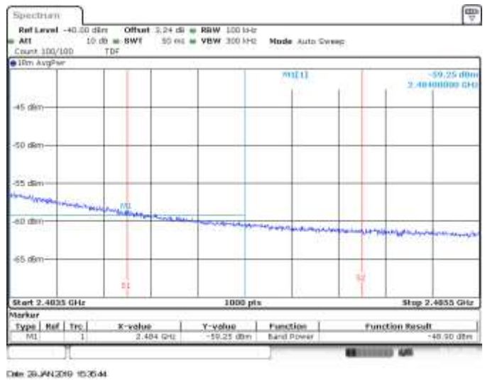
MIMO B, CH12, 802.11ax20, HE0, BE High RMS within 2MHz (Restricted)
