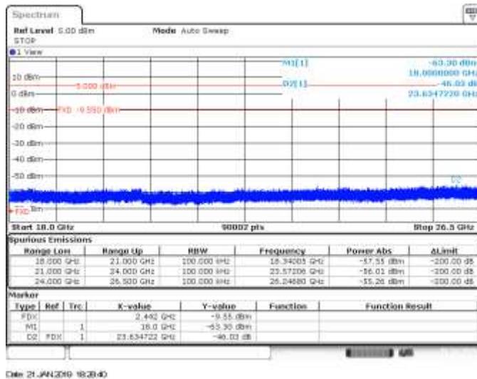
CH7, 802.11n20, HT0, SISO A, Range 18GHz to 26.5GHz - Delta Marker Measurement
