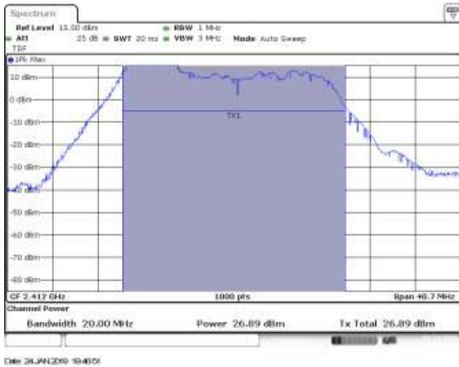
MIMO B, CH1, 802.11ax20_R52_37, HE0, Power
