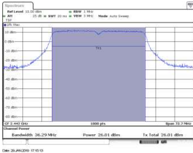
MIMO B, CH7, 802.11n40, HT8, Power
