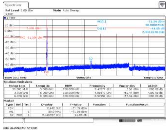
CH7, 802.11ax20, HE0, SISO B, Range 30MHz to 9GHz - Delta Marker Measurement
