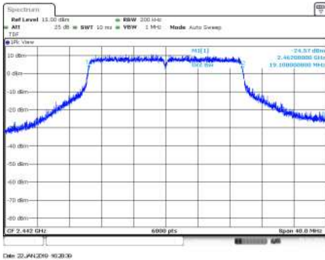
SISO A, CH7, 802.11ax20, HE0, 99% Occupied Bandwidth
