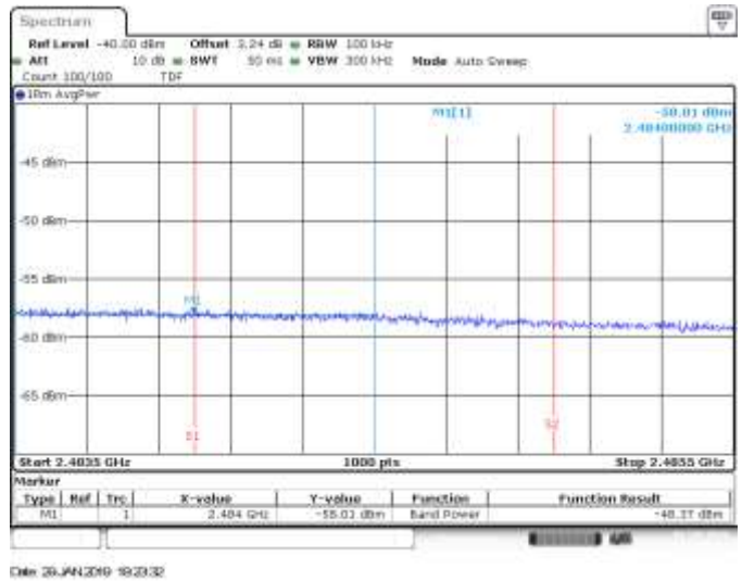
MIMO B, CH9, 802.11ax40, HE0, BE High RMS within 2MHz (Restricted)
