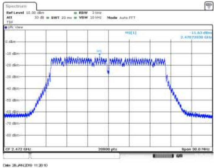
SISO B, CH13, 802.11g, 6Mbps, PSD
