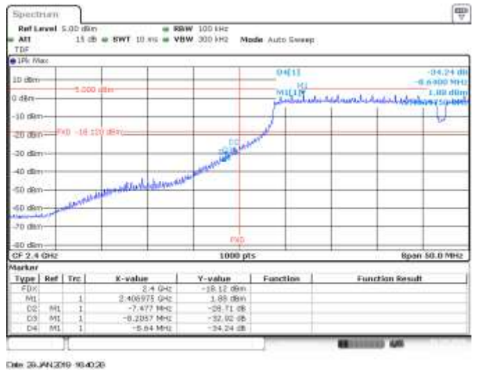
MIMO B, CH3, 802.11n40, HT8, BE Low (Non Restricted)
