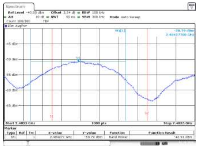
SISO A, CH11, 802.11b, 1Mbps, BE High RMS within 2MHz (Restricted)
