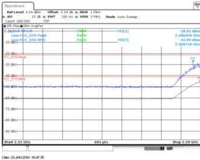
MIMO A, CH3, 802.11ax40, HE0, BE Low
