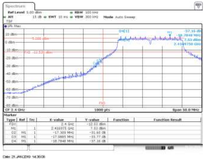
SISO A, CH1, 802.11g, 6Mbps, BE Low (Non Restricted)
