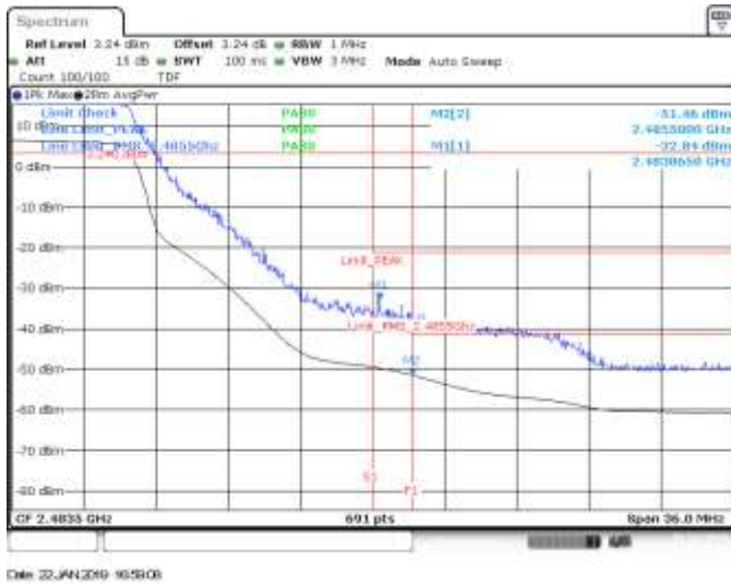
SISO A, CH11, 802.11ax20, HE0, BE High (Restricted)
