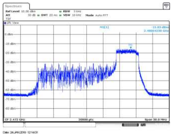
SISO A, CH13, 802.11ax20_R52_40, HE0, PSD
