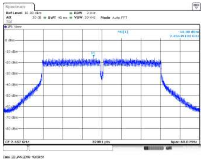
SISO A, CH10, 802.11n40, HT0, PSD
