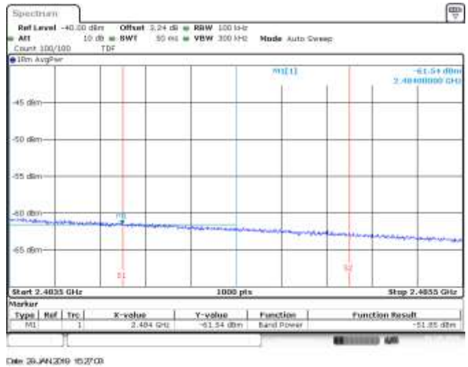
MIMO B, CH11, 802.11ax20, HE0, BE High RMS within 2MHz (Restricted)
