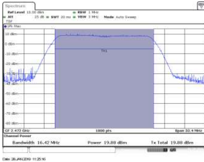
SISO B, CH13, 802.11g, 6Mbps, Power
