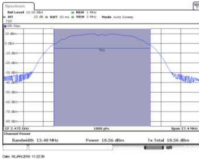
SISO A, CH13, 802.11b, 1Mbps, Power
