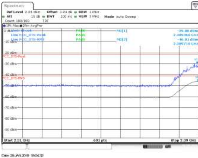
MIMO B, CH3, 802.11ax40, HE0, BE Low
