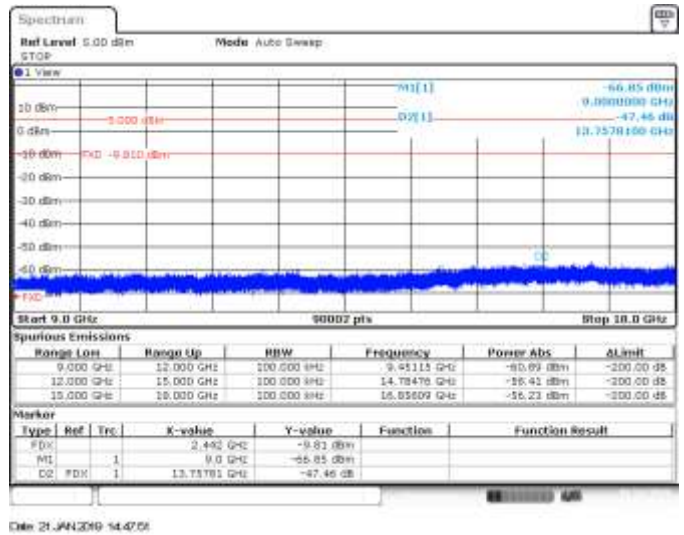
CH7, 802.11g, 6Mbps, SISO A, Range 9GHz to 18GHz - Delta Marker Measurement
