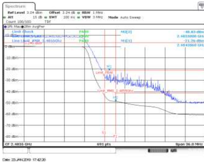
SISO A, CH11, 802.11n40, HT0, BE High (Restricted)
