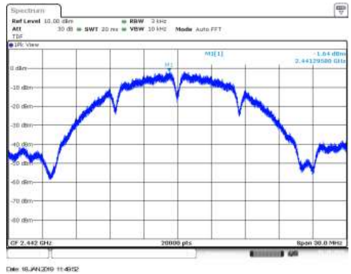
SISO B, CH7, 802.11b, 1Mbps, PSD
