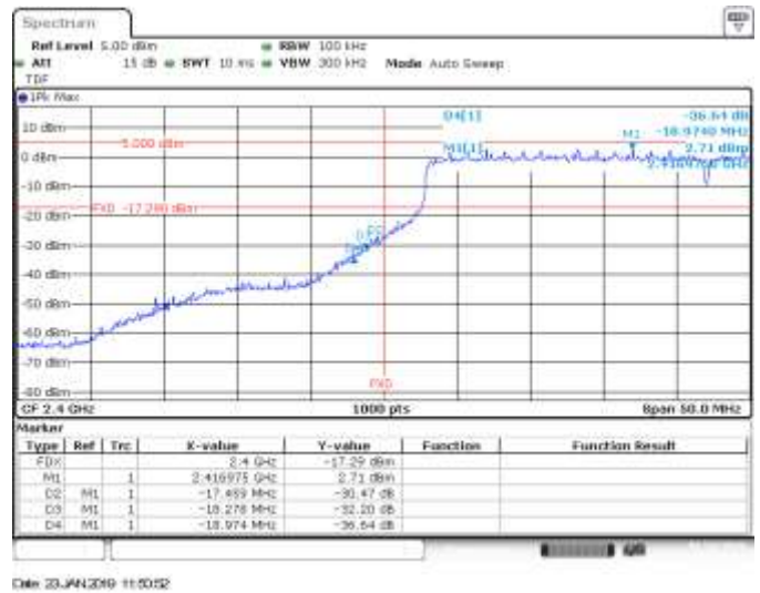
SISO A, CH3, 802.11ax40, HE0, BE Low (Non Restricted)
