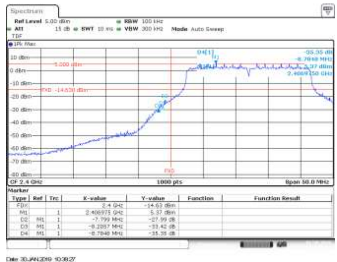
MIMO A, CH1, 802.11ax20, HE0, BE Low (Non Restricted)
