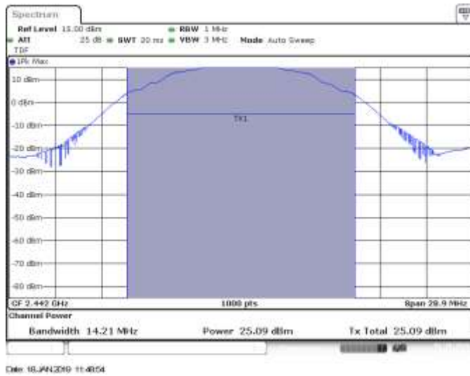
SISO B, CH7, 802.11b, 1Mbps, Power
