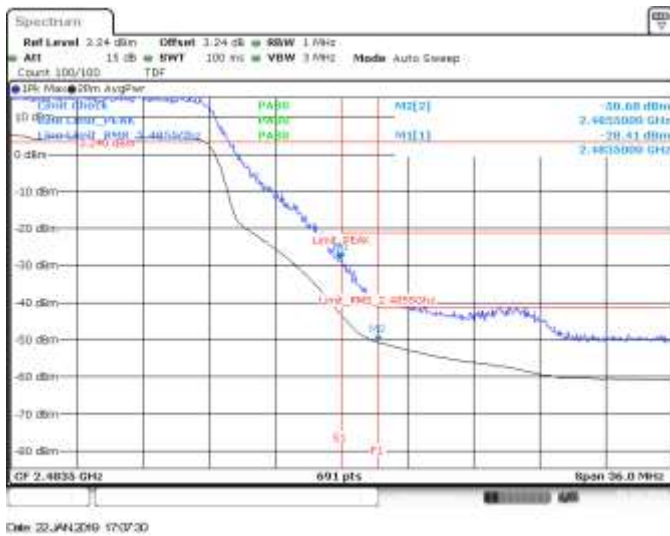
SISO A, CH12, 802.11ax20, HE0, BE High (Restricted)
