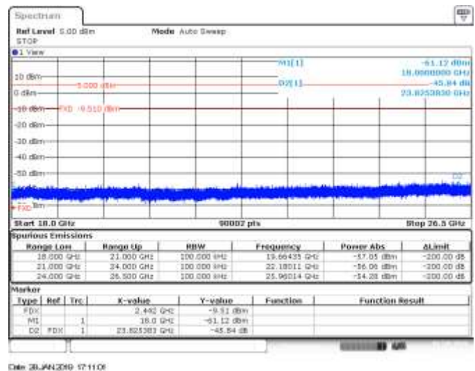
CH7, 802.11n20, HT0, SISO B, Range 18GHz to 26.5GHz - Delta Marker Measurement
