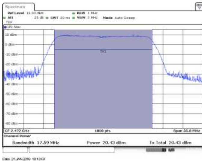
SISO A, CH13, 802.11n20, HT0, Power
