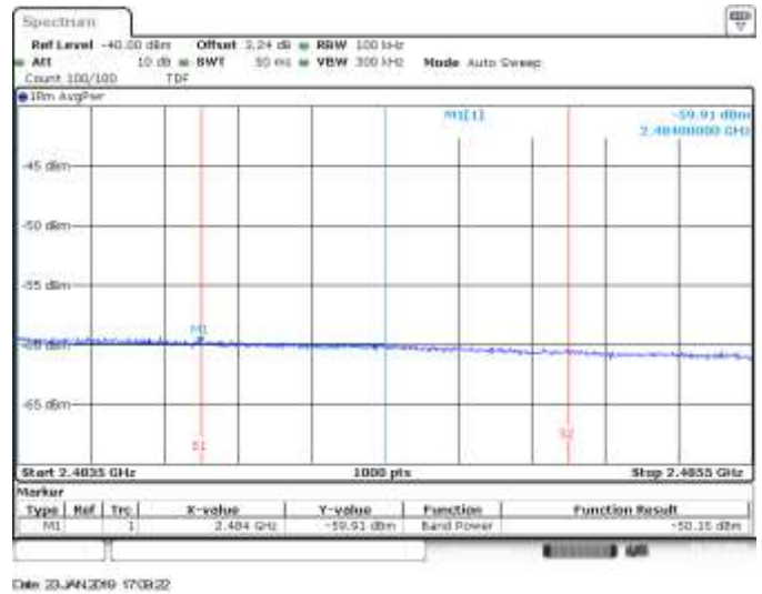
MIMO A, CH9, 802.11ax40, HE0, BE High RMS within 2MHz (Restricted)
