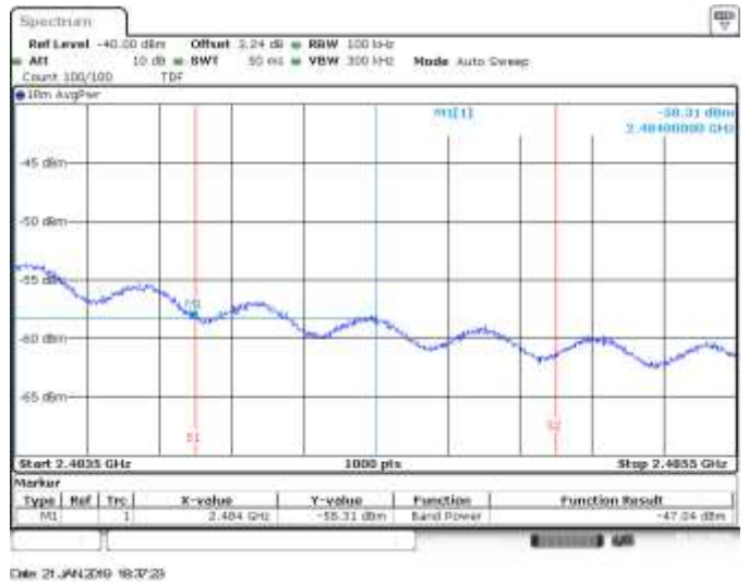
SISO A, CH12, 802.11n20, HT0, BE High RMS within 2MHz (Restricted)
