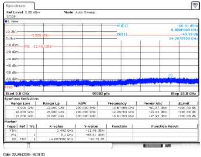
CH7, 802.11ax20, HE0, SISO A, Range 9GHz to 18GHz - Delta Marker Measurement
