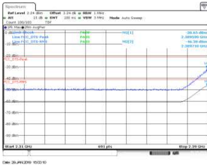
MIMO B, CH1, 802.11ax20, HE0, BE Low
