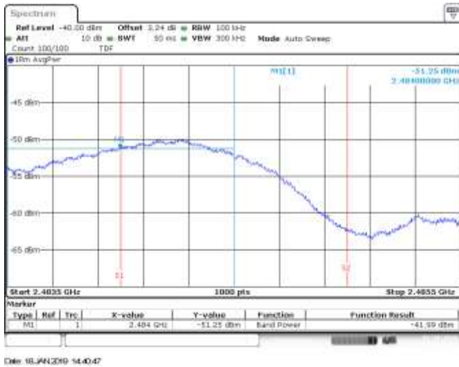
SISO B, CH12, 802.11b, 1Mbps, BE High (Restricted)
