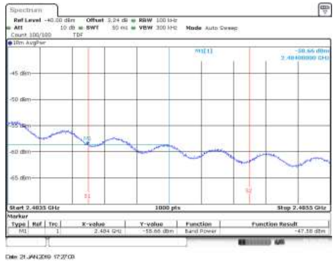
SISO A, CH12, 802.11g, 6Mbps, BE High RMS within 2MHz (Restricted)
