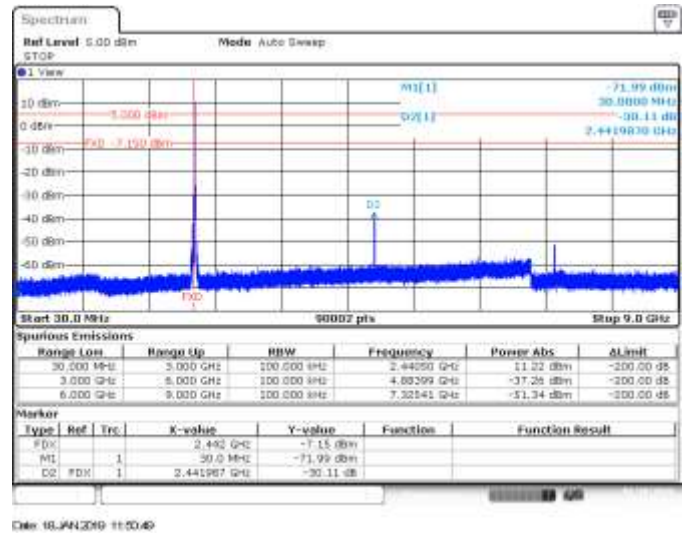
CH7, 802.11b, 1Mbps, SISO B, Range 30MHz to 9GHz - Delta Marker Measurement
