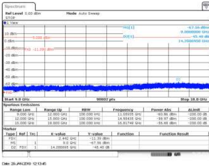
CH7, 802.11ax20, HE0, SISO B, Range 9GHz to 18GHz - Delta Marker Measurement
