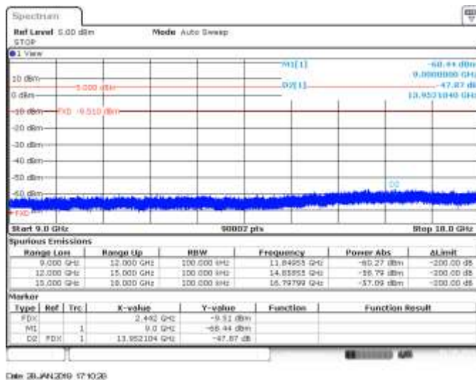
CH7, 802.11n20, HT0, SISO B, Range 9GHz to 18GHz - Delta Marker Measurement
