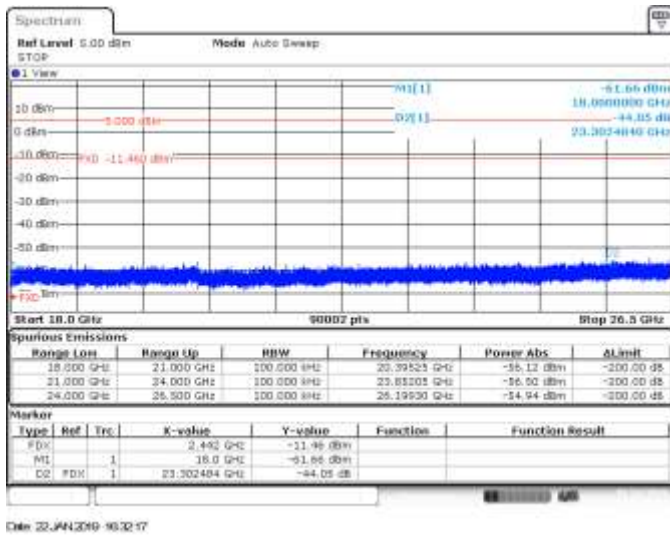
CH7, 802.11ax20, HE0, SISO A, Range 18GHz to 26.5GHz - Delta Marker Measurement
