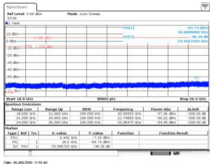
CH7, 802.11b, 1Mbps, SISO B, Range 18GHz to 26.5GHz - Delta Marker Measurement
