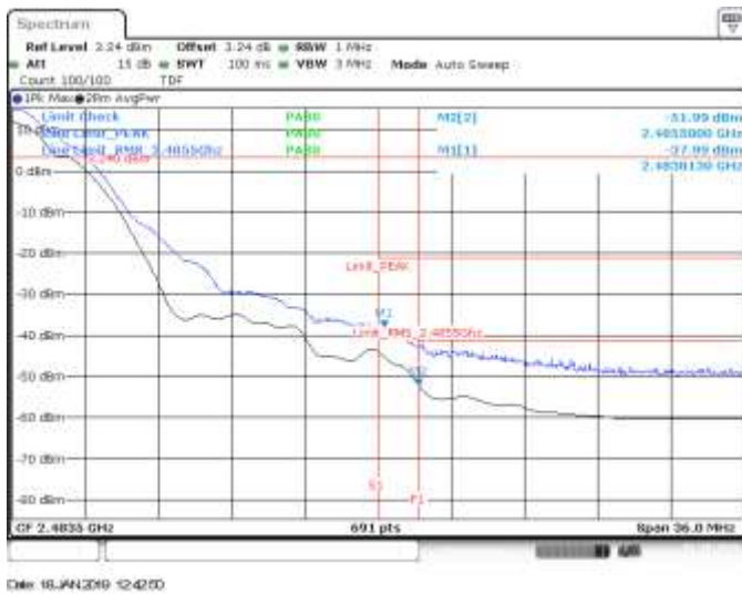
SISO B, CH11, 802.11b, 1Mbps, BE High (Restricted)
