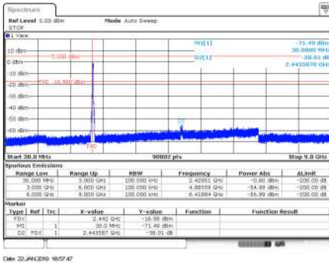
CH7, 802.11n40, HT0, SISO A, Range 30MHz to 9GHz - Delta Marker Measurement
