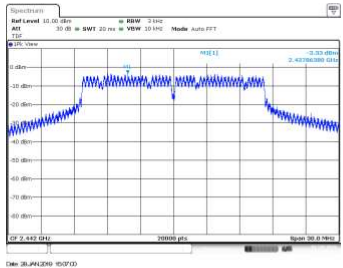
SISO B, CH7, 802.11g, 6Mbps, PSD
