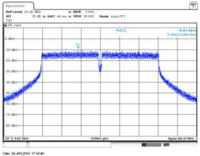
MIMO B, CH7, 802.11n40, HT8, PSD
