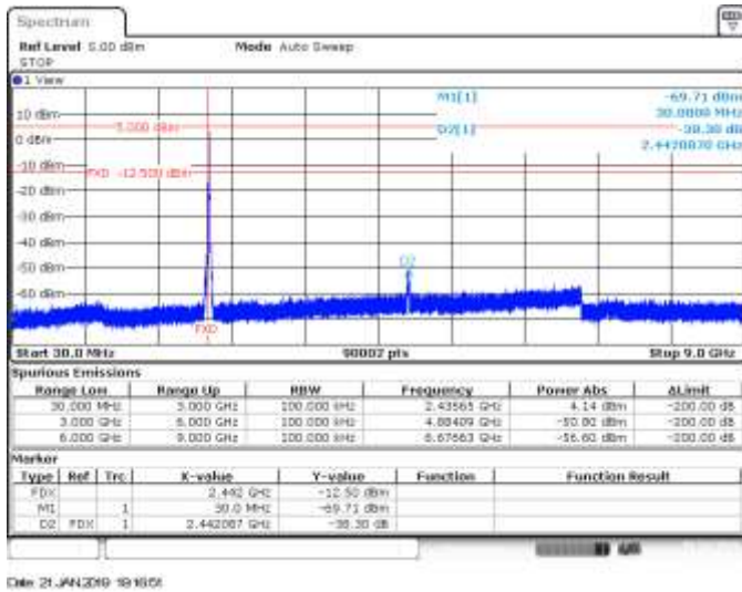
CH7, 802.11n20, HT8, MIMO A, Range 30MHz to 9GHz - Delta Marker Measurement
