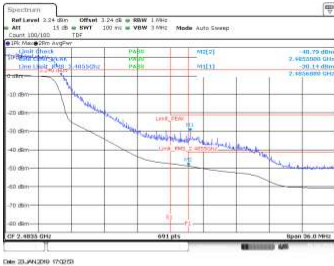
MIMO A, CH9, 802.11ax40, HE0, BE High (Restricted)
