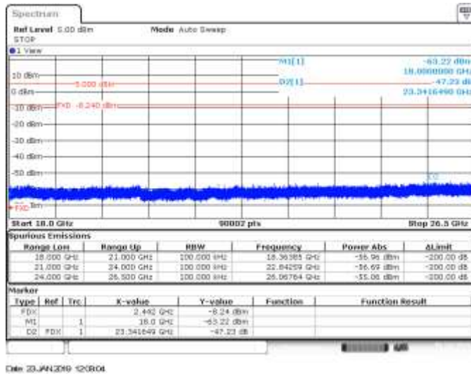
CH7, 802.11b, 1Mbps, SISO A, Range 18GHz to 26.5GHz - Delta Marker Measurement
