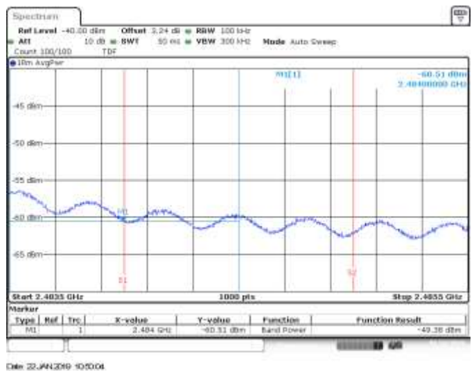
MIMO A, CH12, 802.11n20, HT8, BE High RMS within 2MHz (Restricted)
