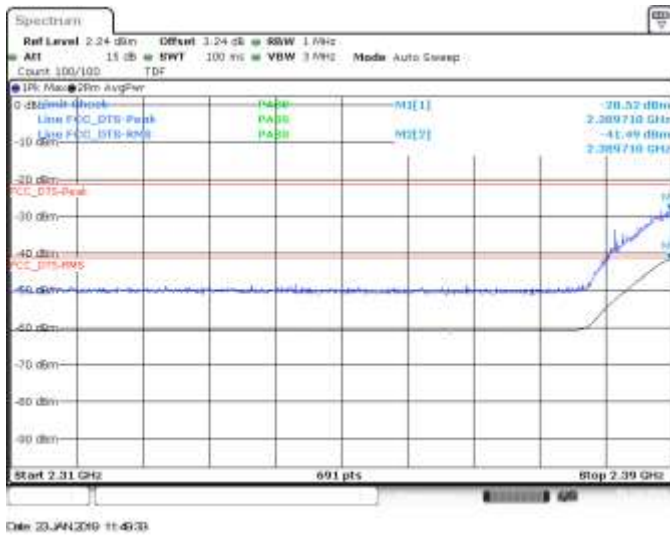
SISO A, CH3, 802.11ax40, HE0, BE Low
