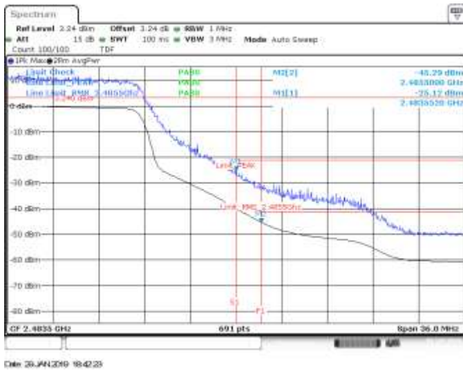
SISO B, CH10, 802.11ax40, HE0, BE High (Restricted)
