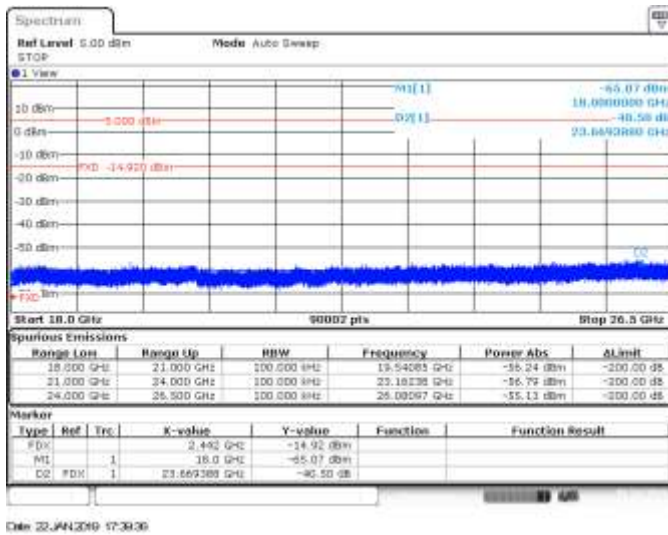
CH7, 802.11ax20, HE0, MIMO A, Range 18GHz to 26.5GHz - Delta Marker Measurement
