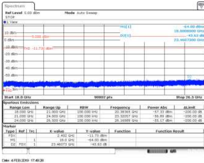
CH 37, Conducted Spurious Range 18GHz to 26.5GHz - Delta Marker Measurement
