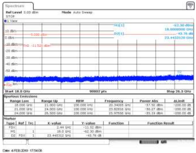
CH 17, Conducted Spurious Range 18GHz to 26.5GHz - Delta Marker Measurement
