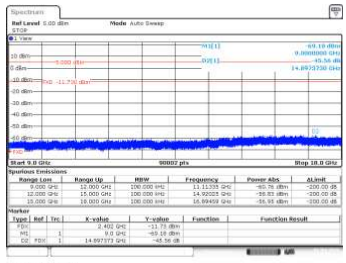
CH 37, Conducted Spurious Range 9GHz to 18GHz - Delta Marker Measurement
