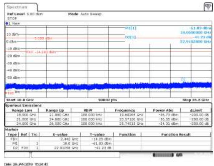
CH7, 802.11ax20, HE0, MIMO B, Range 18GHz to 26.5GHz - Delta Marker Measurement
