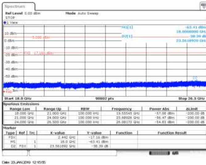
CH7, 802.11ax40, HE0, SISO A, Range 18GHz to 26.5GHz - Delta Marker Measurement
