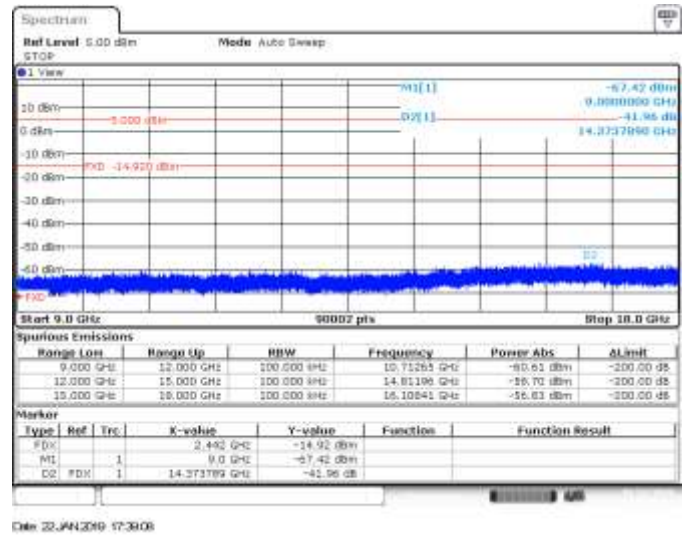
CH7, 802.11ax20, HE0, MIMO A, Range 9GHz to 18GHz - Delta Marker Measurement
