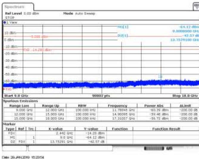
CH7, 802.11ax20, HE0, MIMO B, Range 9GHz to 18GHz - Delta Marker Measurement
