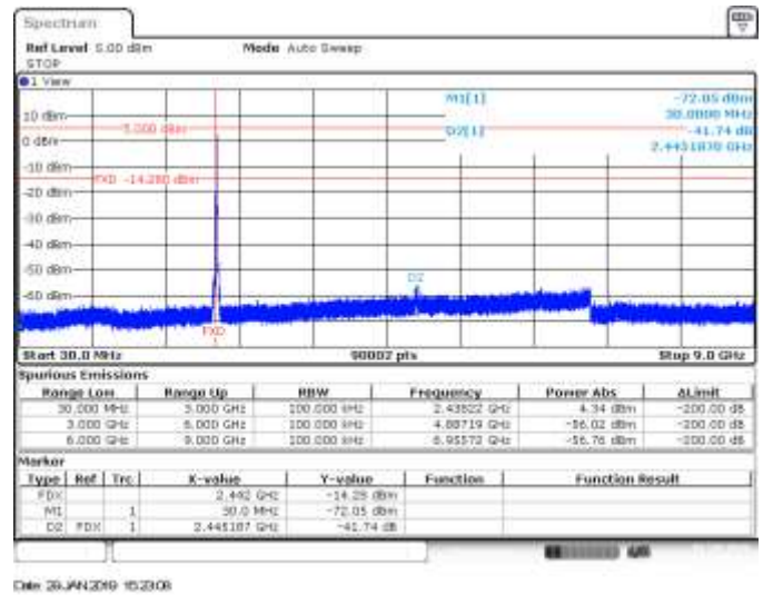
CH7, 802.11ax20, HE0, MIMO B, Range 30MHz to 9GHz - Delta Marker Measurement
