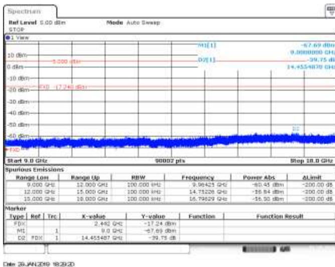
CH7, 802.11ax40, HE0, SISO B, Range 9GHz to 18GHz - Delta Marker Measurement
