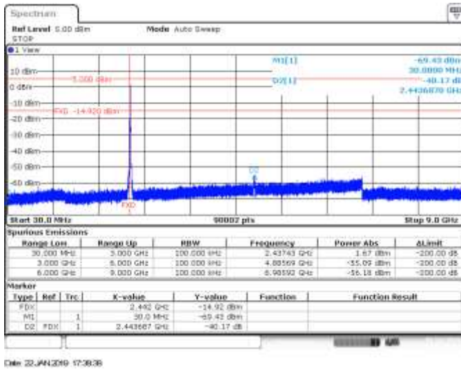
CH7, 802.11ax20, HE0, MIMO A, Range 30MHz to 9GHz - Delta Marker Measurement
