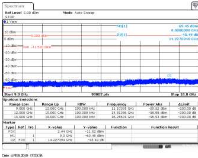
CH 17, Conducted Spurious Range 9GHz to 18GHz - Delta Marker Measurement
