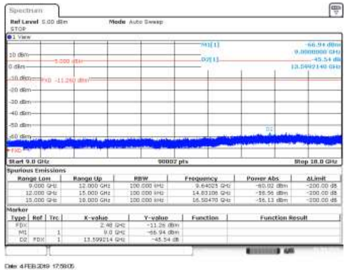
CH 39, Conducted Spurious Range 9GHz to 18GHz - Delta Marker Measurement
