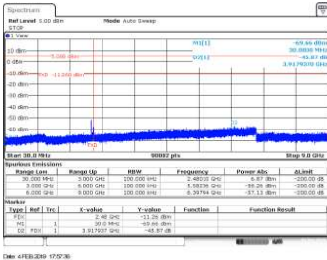
CH 39, Conducted Spurious Range 30MHz to 9GHz - Delta Marker Measurement
