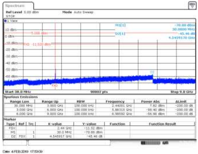
CH 17, Conducted Spurious Range 30MHz to 9GHz - Delta Marker Measurement
