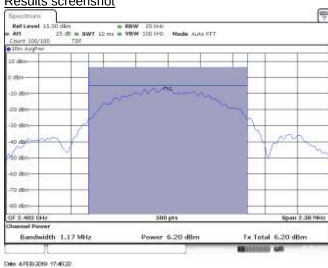
CH 37, Max Power RMS
