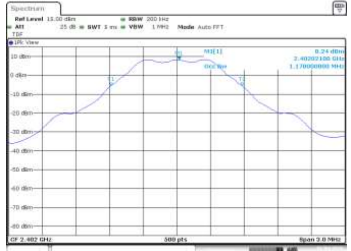
CH 37, 99% Occupied Bandwidth
