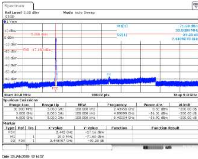
CH7, 802.11ax40, HE0, SISO A, Range 30MHz to 9GHz - Delta Marker Measurement
