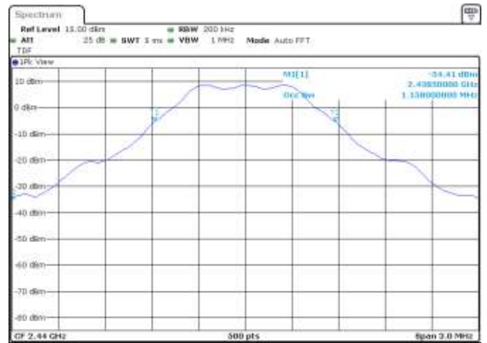
CH 37, 99% Occupied Bandwidth
