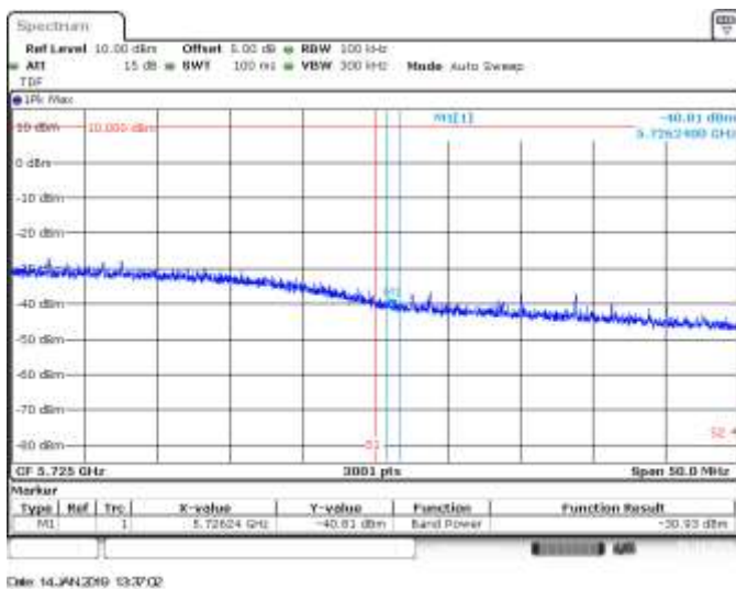
MIMO A, 802.11ax40, HE0, CH134, BE High Peak
