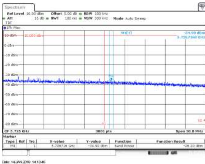
SISO A, 802.11ax80, HE0, CH122, BE High Peak
