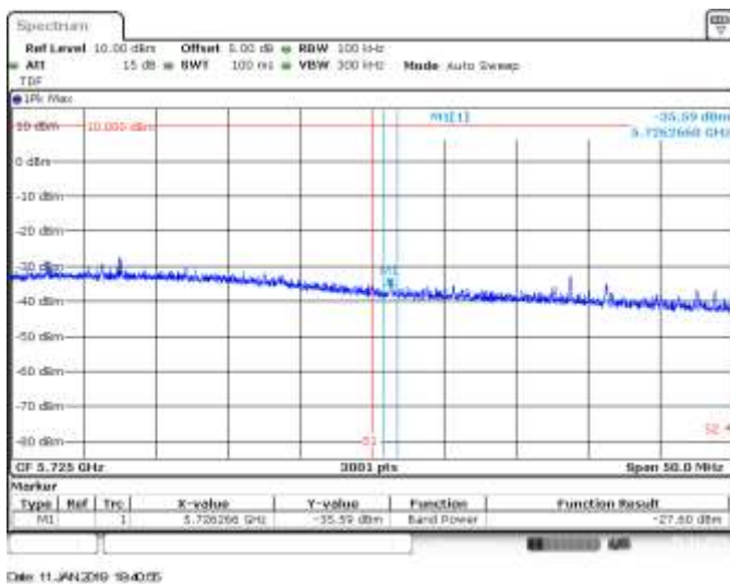
SISO A, 802.11ax40, HE0, CH134, BE High Peak
