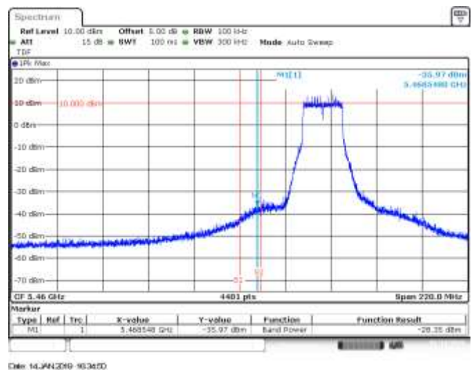
SISO B, 802.11ax20, HE0, CH100, BE Low Peak (Non Restricted)
