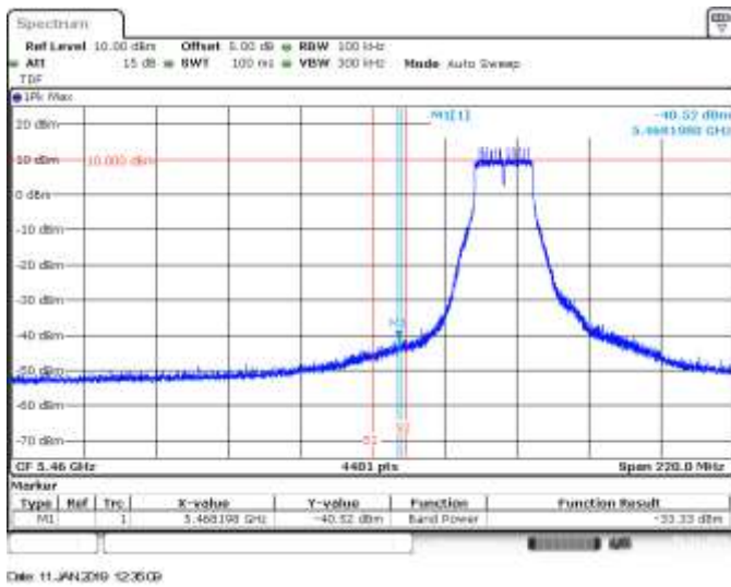
MIMO A, 802.11n20, HT8, CH100, BE Low Peak (Non Restricted)
