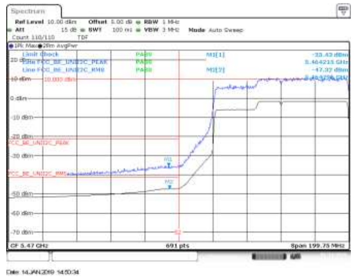
MIMO A, 802.11ax160, HE0, CH114, BE Low RMS, Peak
