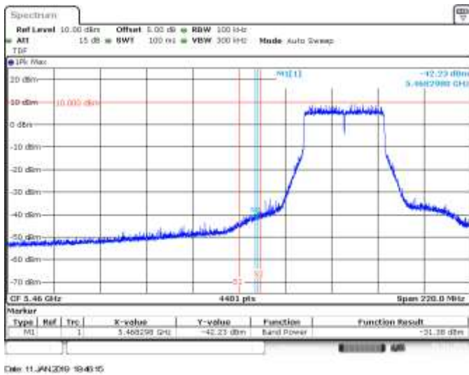
MIMO A, 802.11ax40, HE0, CH102, BE Low Peak (Non Restricted)
