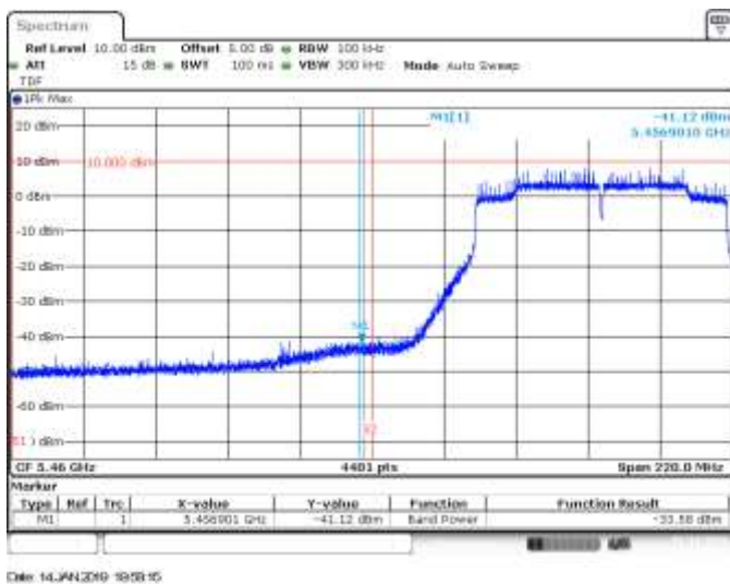
SISO B, 802.11ac80, VHT0, CH106, BE Low Peak (Restricted)
