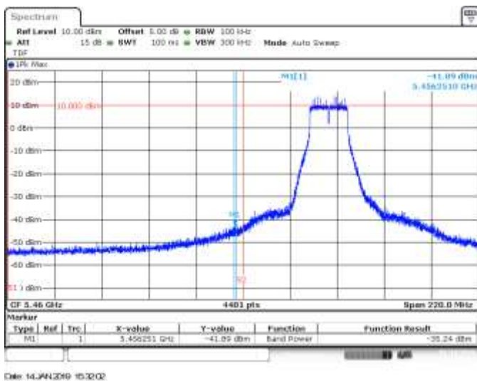
SISO B, 802.11n20, HT0, CH100, BE Low Peak (Restricted)
