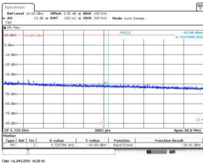
MIMO A, 802.11ax80, HE0, CH122, BE High Peak
