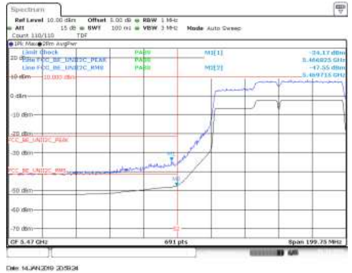
MIMO B, 802.11ac160, VHT0, CH114, BE Low RMS, Peak
