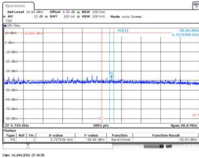
MIMO B, 802.11ax160, HE0, CH114, BE High Peak
