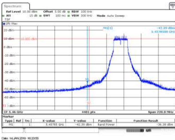
MIMO B, 802.11n20, HT8, CH100, BE Low Peak (Restricted)
