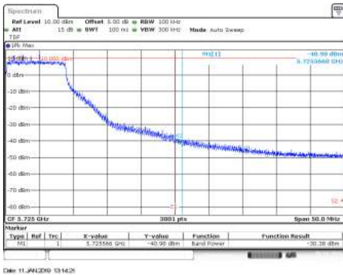
MIMO A, 802.11n20, HT8, CH140, BE High Peak
