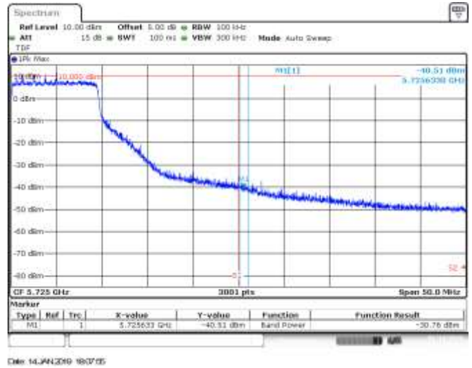
MIMO B, 802.11ax20, HE0, CH140, BE High Peak
