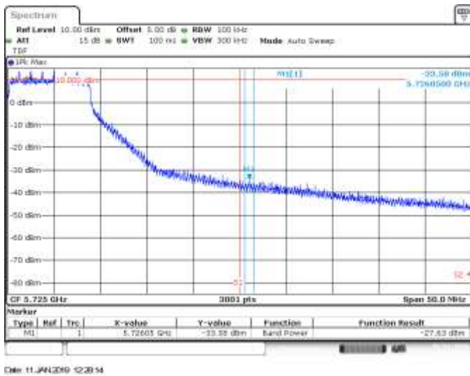
SISO A, 802.11n20, HT0, CH140, BE High Peak
