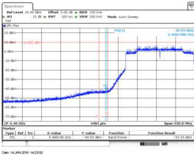
MIMO A, 802.11ax80, HE0, CH106, BE Low Peak (Non Restricted)
