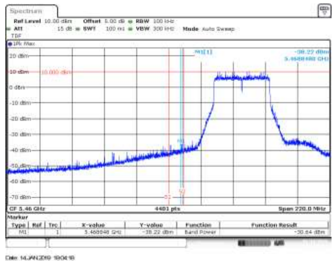
SISO B, 802.11ax40, HE0, CH102, BE Low Peak (Non Restricted)
