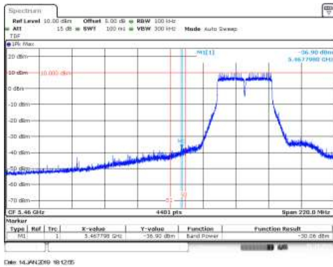
SISO B, 802.11n40, HT0, CH102, BE Low Peak (Non Restricted)
