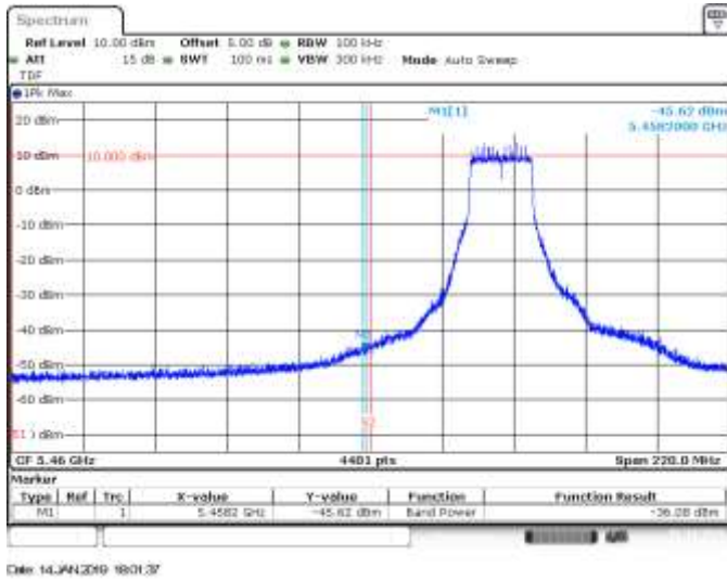
MIMO B, 802.11ax20, HE0, CH100, BE Low Peak (Restricted)
