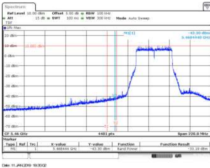
SISO A, 802.11ax40, HE0, CH102, BE Low Peak (Non Restricted)
