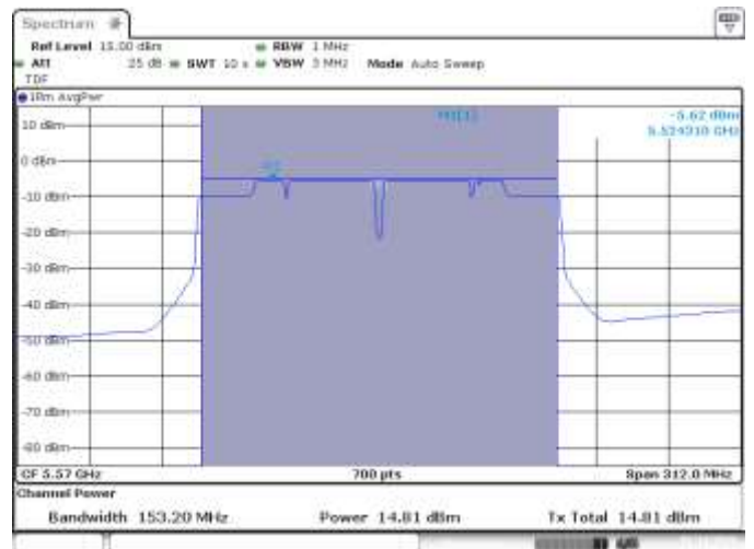
SISO B, CH114, 802.11ac160, VHT0
