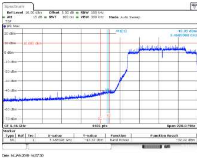
SISO A, 802.11ax80, HE0, CH106, BE Low Peak (Non Restricted)
