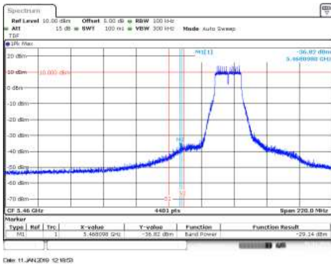
SISO A, 802.11n20, HT0, CH100, BE Low Peak (Non Restricted)
