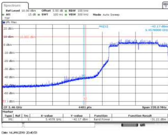
MIMO B, 802.11ax80, HE0, CH106, BE Low Peak (Restricted)
