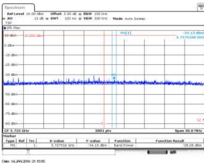
SISO B, 802.11ax160, HE0, CH114, BE High Peak
