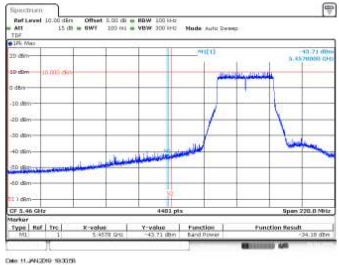
SISO A, 802.11ax40, HE0, CH102, BE Low Peak (Restricted)
