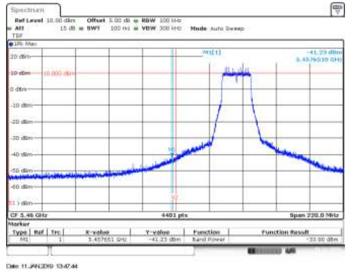
SISO A, 802.11ax20, HE0, CH100, BE Low Peak (Restricted)
