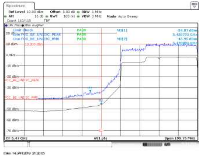
MIMO B, 802.11ax160, HE0, CH114, BE Low RMS, Peak
