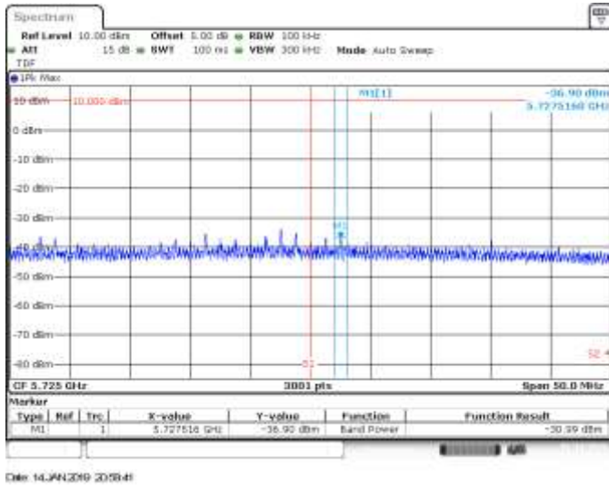
MIMO B, 802.11ac160, VHT0, CH114, BE High Peak
