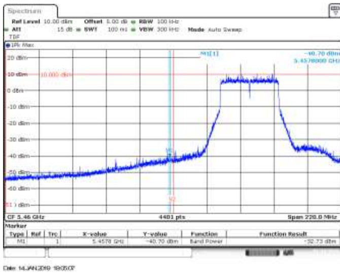
SISO B, 802.11ax40, HE0, CH102, BE Low Peak (Restricted)
