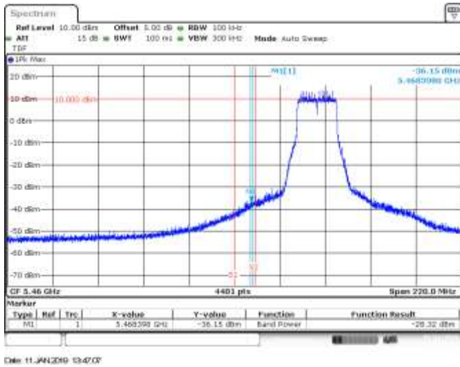
SISO A, 802.11ax20, HE0, CH100, BE Low Peak (Non Restricted)
