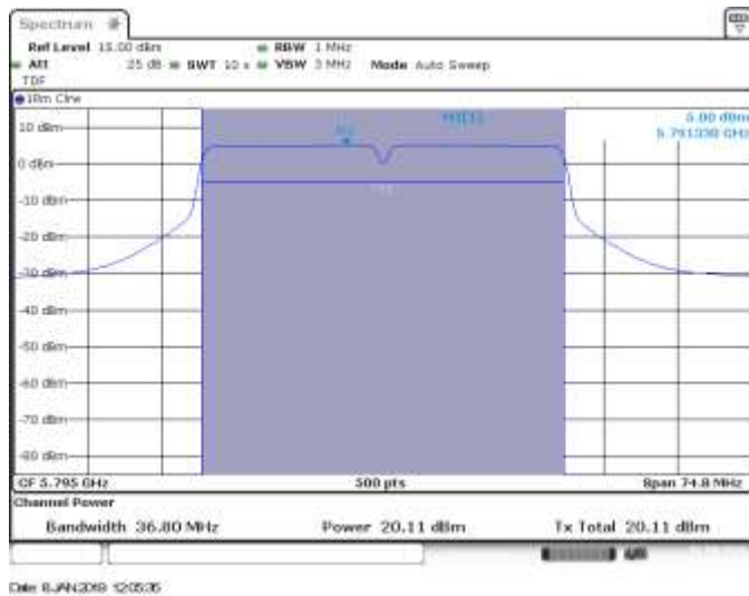
MIMO A, CH159, 802.11n40, HT8
