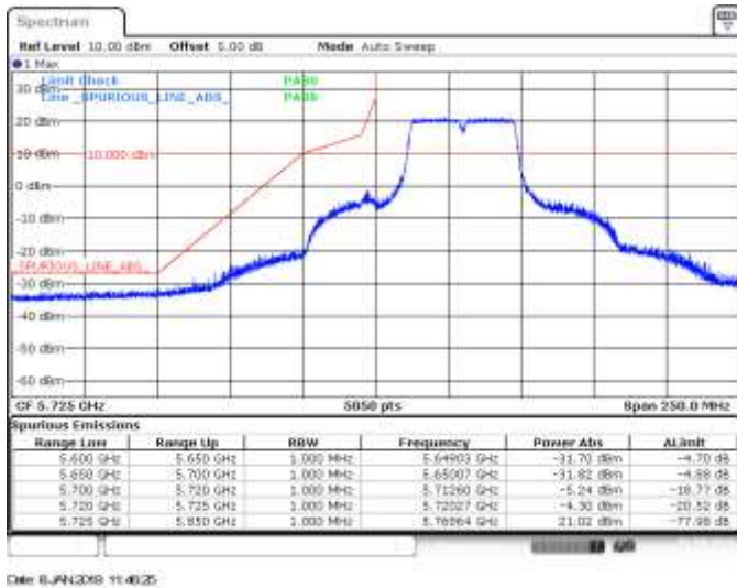
SISO A, 802.11n40, HT0, CH151, BE Low Peak
