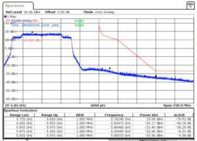
SISO A, 802.11ax80, HE0, CH155, BE High Peak
