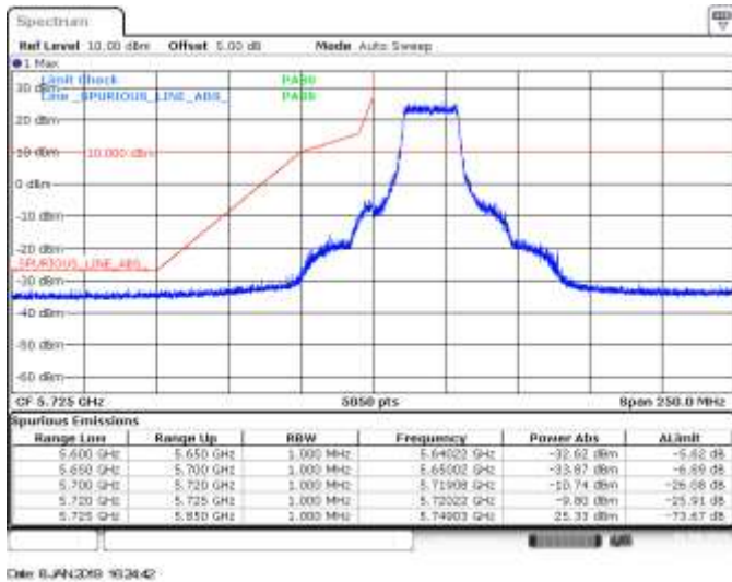
SISO B, 802.11ax20, HE0, CH149, BE Low Peak
