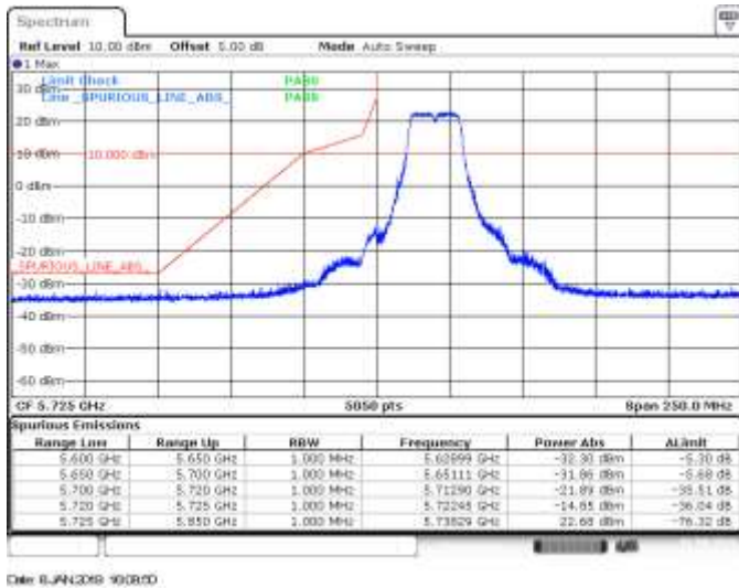
MIMO B, 802.11n20, HT8, CH149, BE Low Peak
