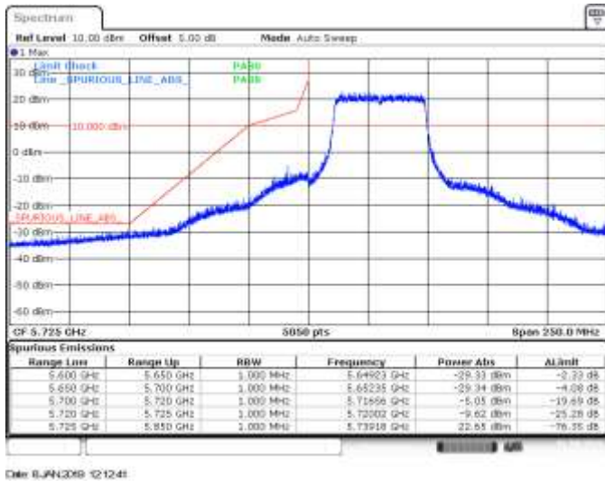
SISO A, 802.11ax40, HE0, CH151, BE Low Peak
