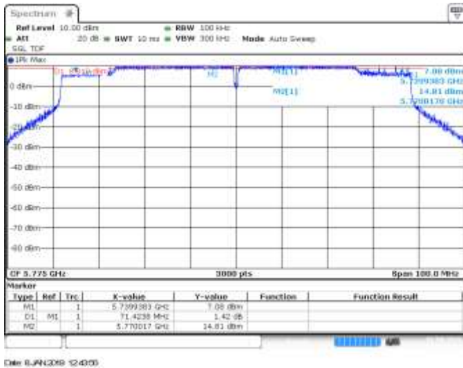
SISO A, CH155, 802.11ac80, VHT0, 6dB BW
