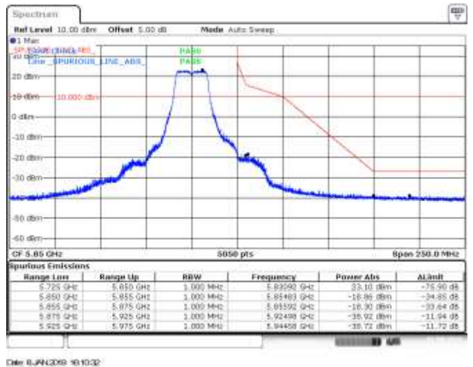
MIMO B, 802.11n20, HT8, CH165, BE High Peak
