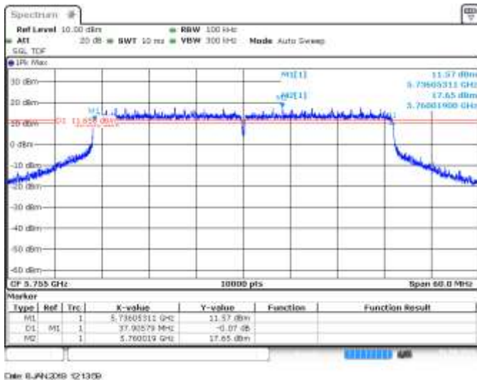
SISO A, CH151, 802.11ax40, HE0, 6dB BW
