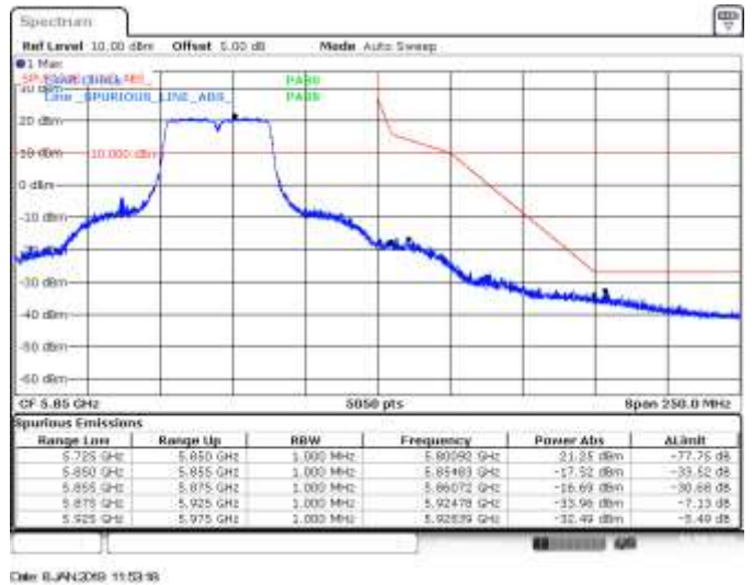
SISO A, 802.11n40, HT0, CH159, BE High Peak
