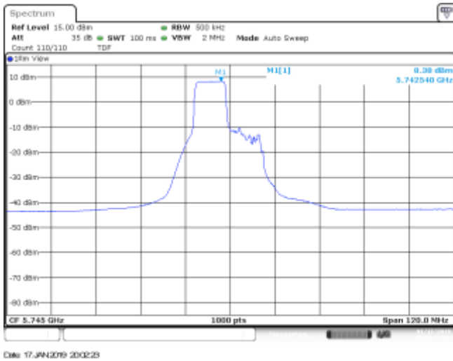
MIMO A, CH149, RU106_53, 802.11ax20, HE0
