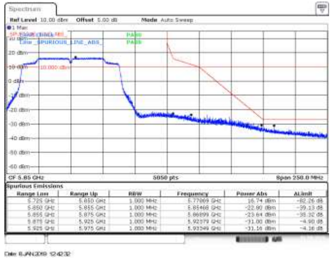
SISO A, 802.11ac80, VHT0, CH155, BE High Peak
