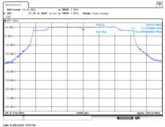
MIMO A, CH155, 802.11ac80, VHT0, 99% BW
