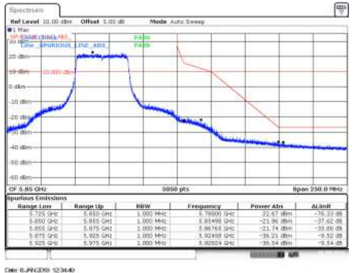
MIMO A, 802.11ax40, HE0, CH159, BE High Peak
