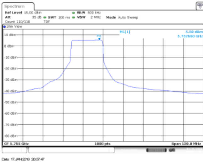
SISO A, CH151, RU242_61, 802.11ax40, HE0
