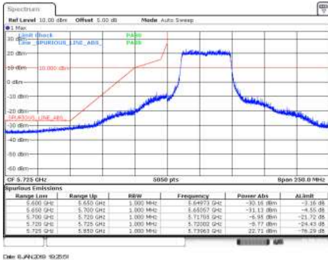
SISO B, 802.11ax40, HE0, CH151, BE Low Peak
