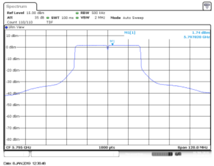
MIMO A, CH159, 802.11ax40, HE0
