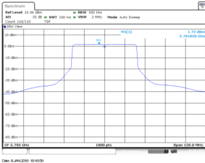
MIMO B, CH159, 802.11ax40, HE0
