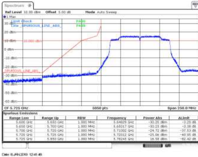
SISO A, 802.11ac80, VHT0, CH155, BE Low Peak
