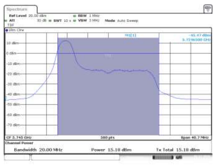
SISO A, CH149, RU26_0, 802.11ax20, HE0
