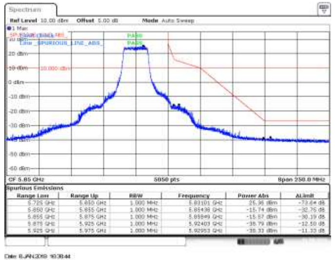
SISO B, 802.11ax20, HE0, CH165, BE High Peak
