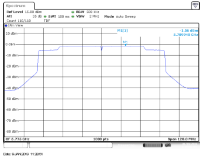
SISO B, CH155, 802.11ax80, HE0
