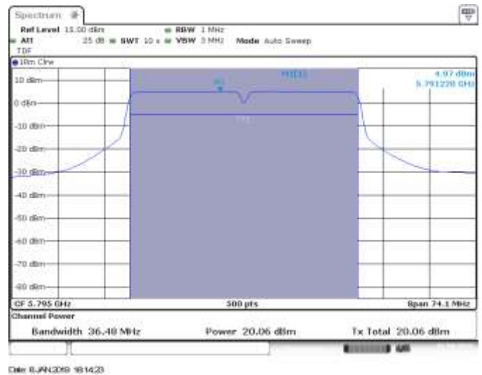
MIMO B, CH159, 802.11n40, HT8
