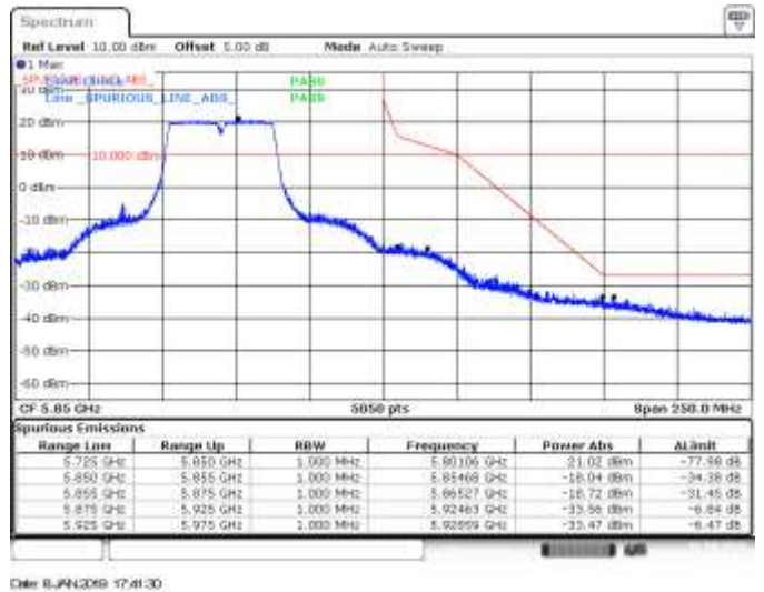
SISO B, 802.11n40, HT0, CH159, BE High Peak
