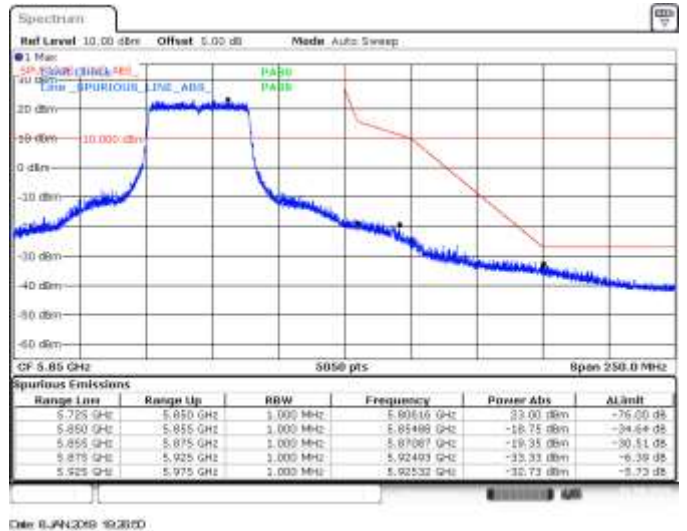
SISO B, 802.11ax40, HE0, CH159, BE High Peak
