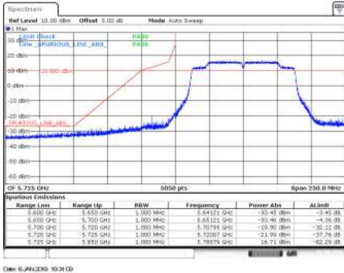
SISO B, 802.11ac80, VHT0, CH155, BE Low Peak
