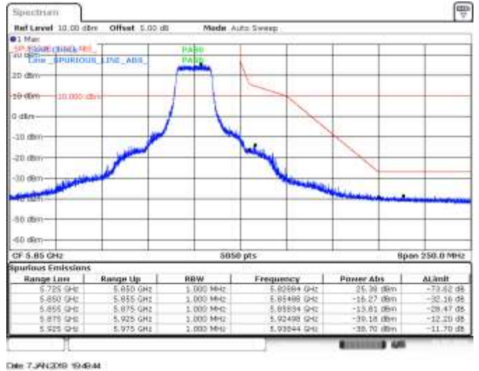
SISO A, 802.11ax20, HE0, CH165, BE High Peak
