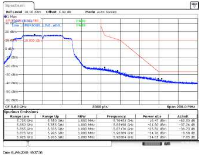
MIMO B, 802.11ac80, VHT0, CH155, BE High Peak
