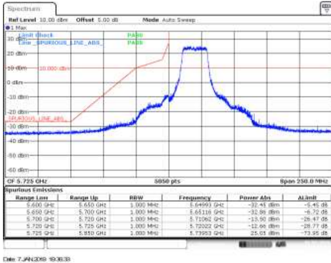
SISO A, 802.11ax20, HE0, CH149, BE Low Peak
