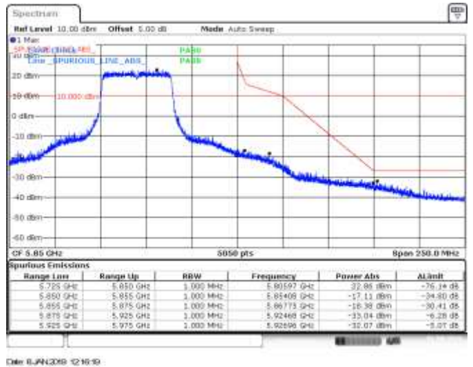
SISO A, 802.11ax40, HE0, CH159, BE High Peak
