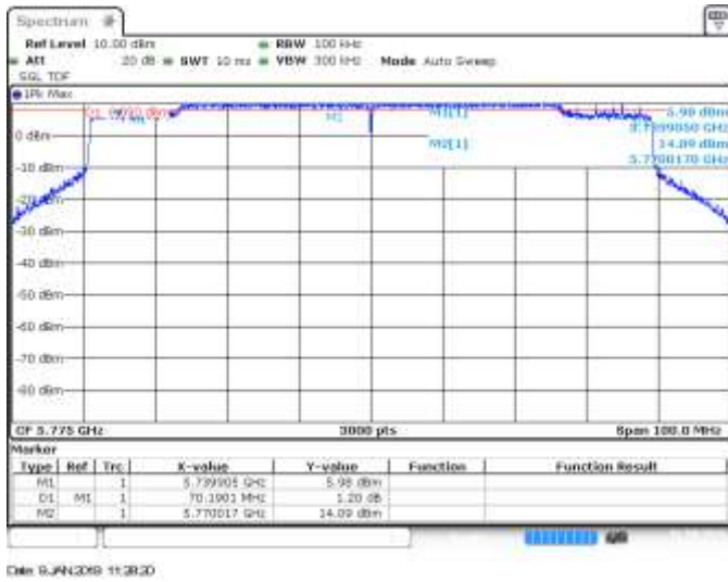
SISO B, CH155, 802.11ax80, HE0, 6dB BW
