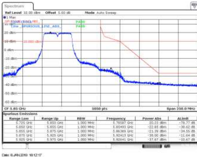
MIMO B, 802.11n20, HT8, CH159, BE High Peak
