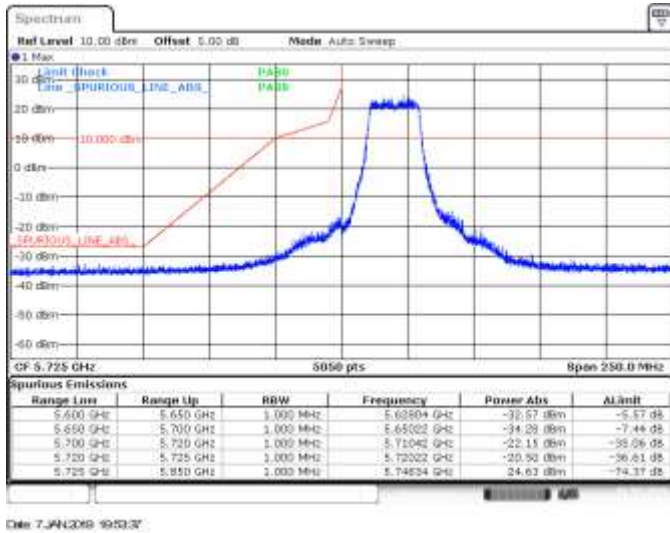
MIMO A, 802.11ax20, HE0, CH149, BE Low Peak
