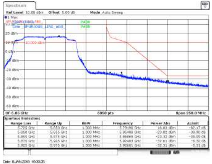
SISO B, 802.11ac80, VHT0, CH155, BE High Peak
