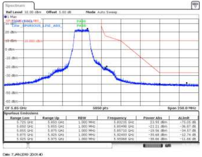
MIMO A, 802.11ax20, HE0, CH165, BE High Peak
