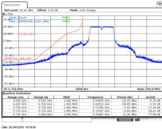
SISO B, 802.11n40, HT0, CH151, BE Low Peak
