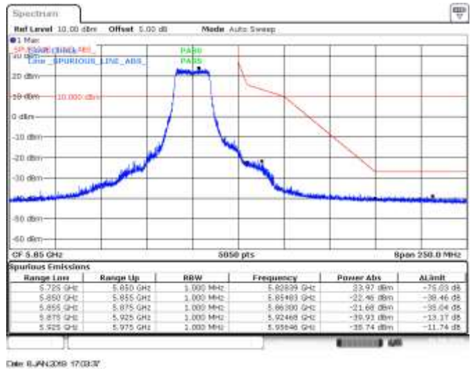
MIMO B, 802.11ax20, HE0, CH165, BE High Peak
