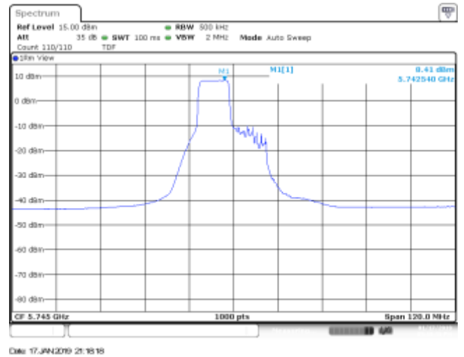
MIMO B, CH149, RU106_53, 802.11ax20, HE0
