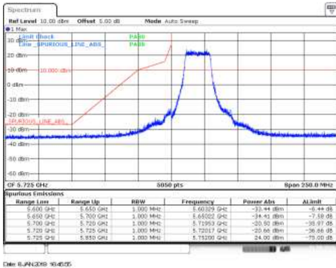
MIMO B, 802.11ax20, HE0, CH149, BE Low Peak
