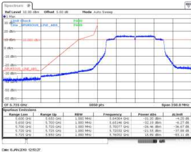
MIMO A, 802.11ac80, VHT0, CH155, BE Low Peak
