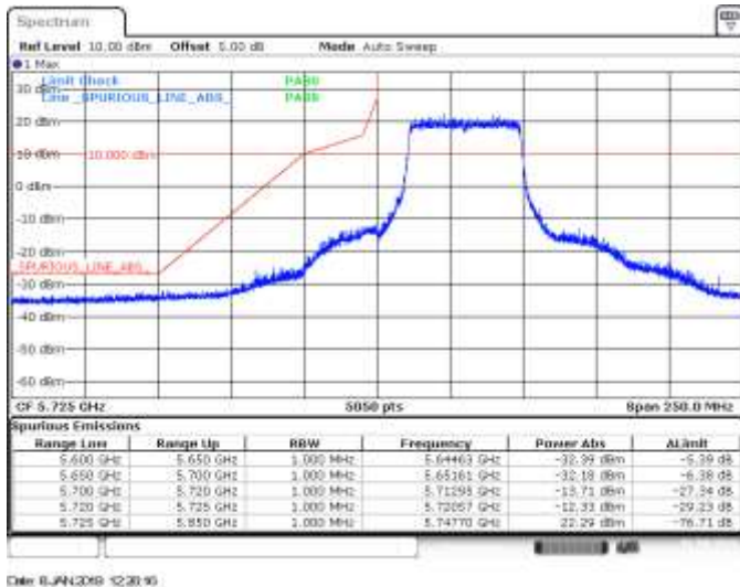
MIMO A, 802.11ax40, HE0, CH151, BE Low Peak
