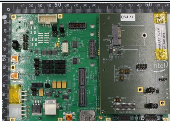
Socket front
