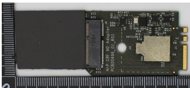
Main Antenna
