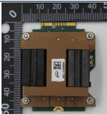
Adaptor front (with absorber)
