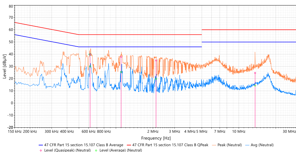
#2-150kHz-30M(Neutral)
