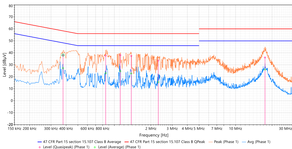
#1-150kHz-30M(Phase 1)
