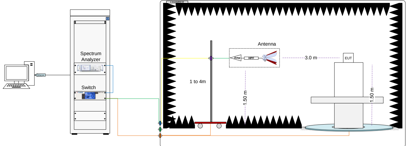
Radiated Setup 9.5 GHz – 18 GHz
