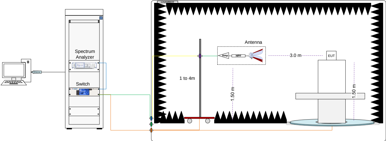
Radiated Setup 9.5 GHz - 18 GHz
