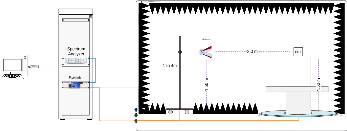
Radiated Setup 1 GHz – 9.5 GHz
