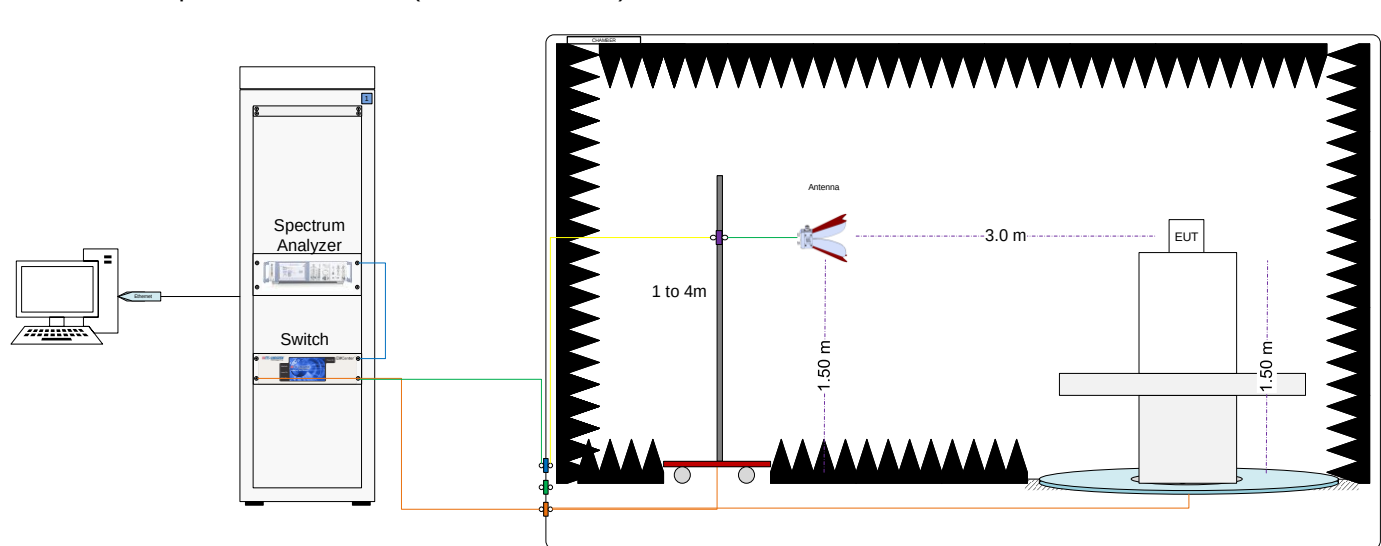
Radiated Setup 1 GHz – 9.5 GHz (Transmitter tests)
