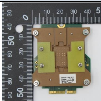
Adaptor front (with absorber)
