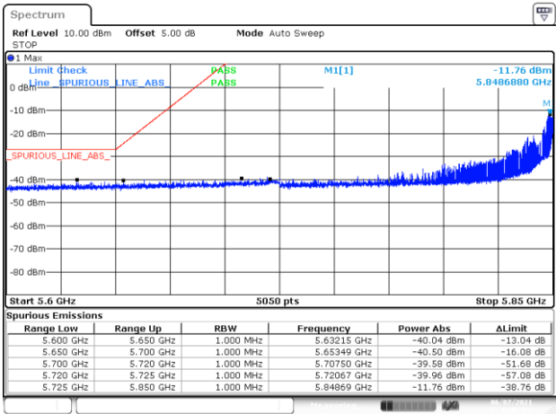
BE-NR-LOW, MIMO-B, 802.11n20-HT8, Ch173
