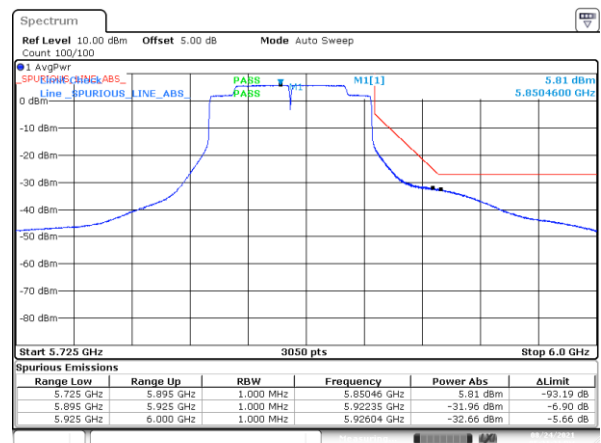
BE-NR-HIGH, MIMO-B, 802.11ac80-VHT0, Ch171
