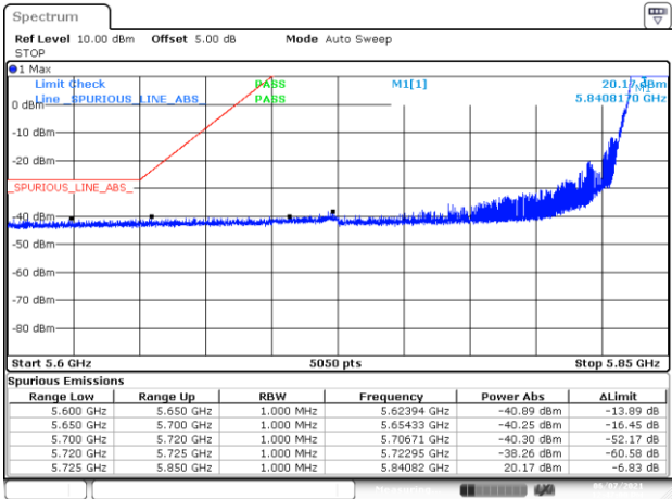
BE-NR-LOW, MIMO-B, 802.11n20-HT8, Ch169
