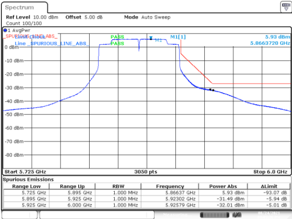
BE-NR-HIGH, MIMO-A, 802.11ac80-VHT0, Ch171
