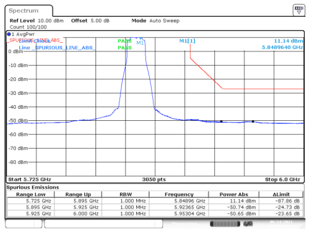
BE-NR-HIGH, SISO-B, 802.11a20-6Mbps, Ch169
