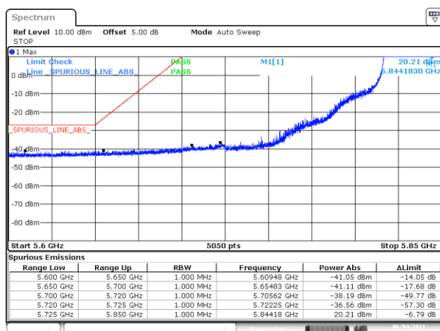
BE-NR-LOW, MIMO-A, 802.11n40-HT8, Ch167
