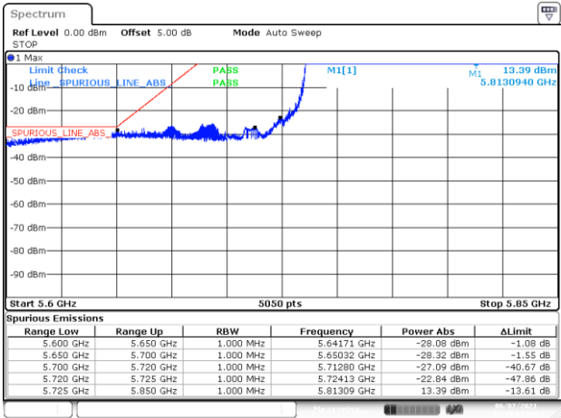
BE-NR-LOW, SISO-B, 802.11ax160-HE0, Ch163
