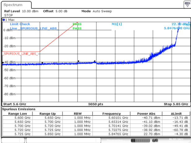
BE-NR-LOW, SISO-B, 802.11n20-HT0, Ch169
