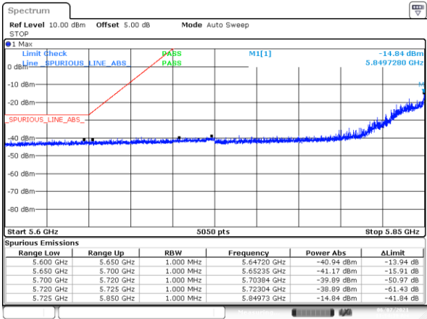
BE-NR-LOW, SISO-B, 802.11n20-HT0, Ch173
