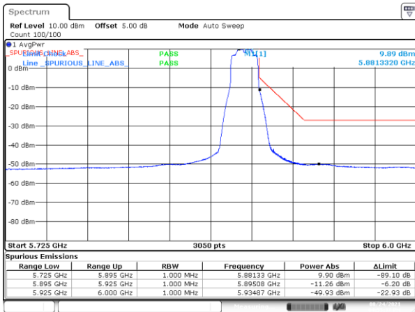
BE-NR-HIGH, MIMO-B, 802.11n20-HT8, Ch177
