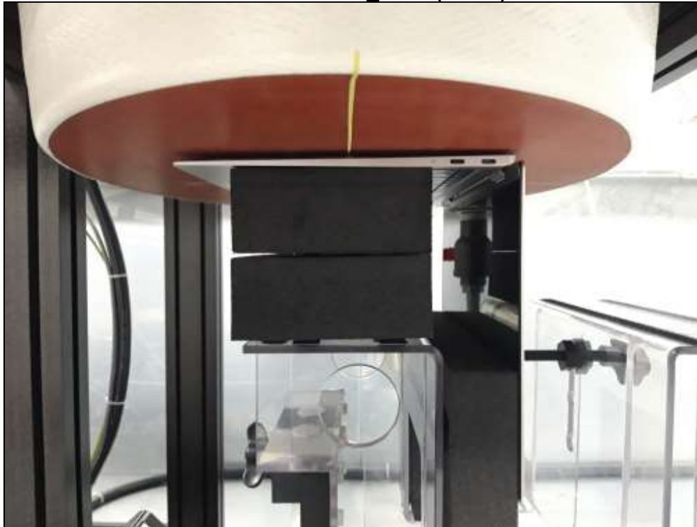
Notebook Mode_Rear (0 mm)
