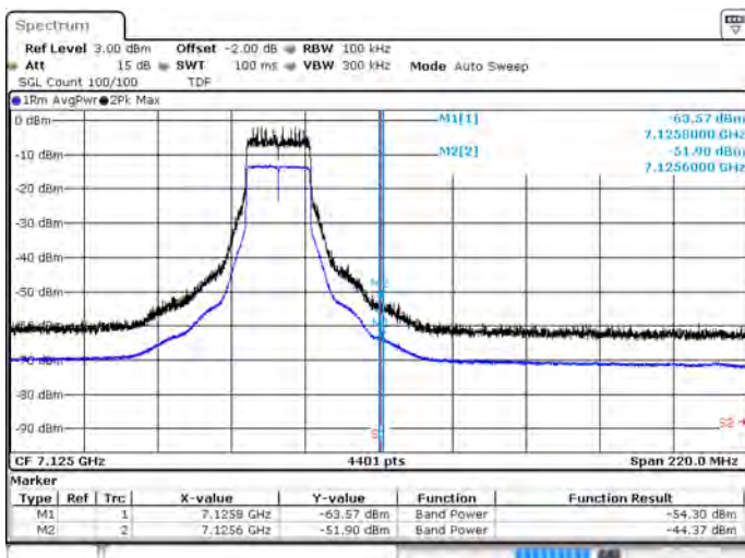
BE-NR-HIGH, SISO-A, 802.11ax20-MCS0, Ch229
