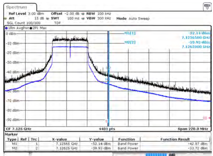
BE-NR-HIGH, SISO-A, 802.11ax40-MCS0, Ch227
