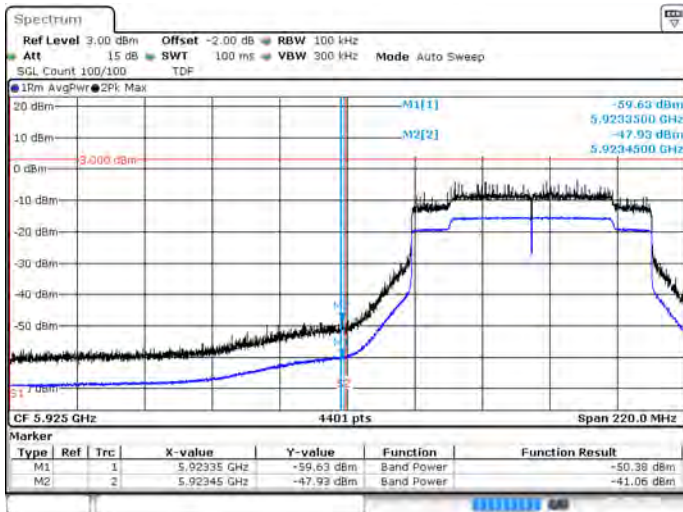
BE-NR-LOW, MIMO-B, 802.11ax80-MCS0, Ch7
