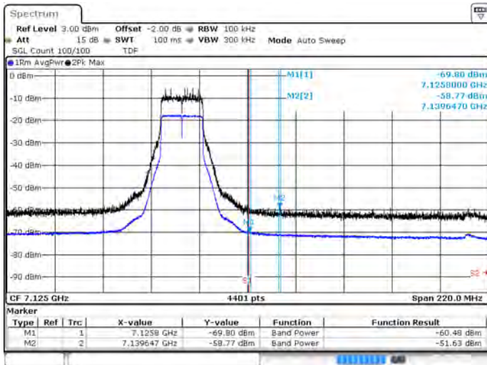
BE-NR-HIGH, MIMO-A, 802.11ax20-MCS0, Ch229
