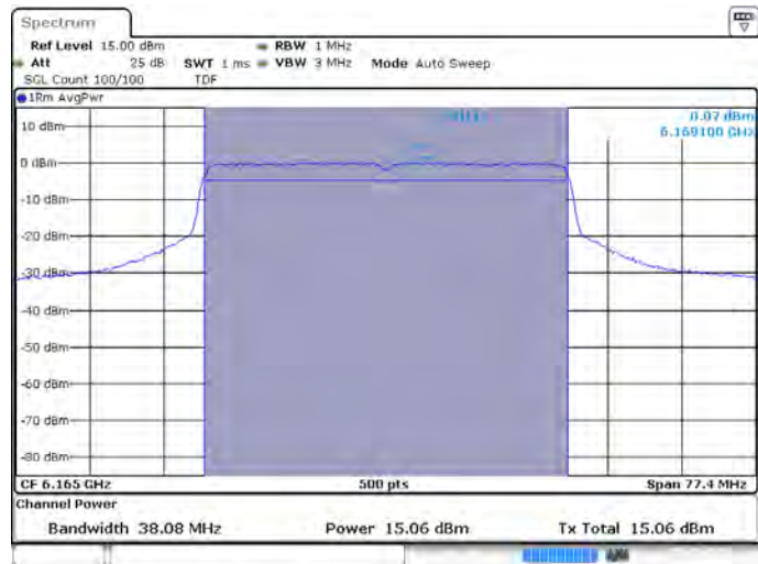
UNII-5 SISO B-802.11ax-40MHz-Ch43-6165MHz-MCS0
