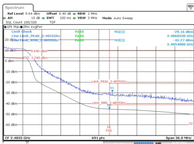
BE-R-HIGH, SISO-B, 802.11n40-HT0, Ch9
