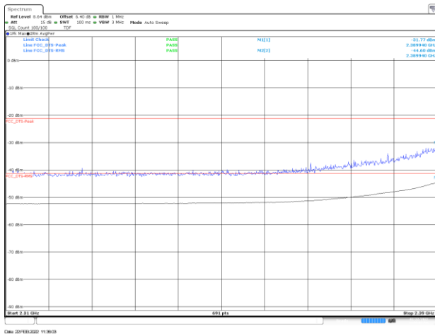
BE-R-LOW, MIMO-A, 802.11n20-HT8, Ch1
