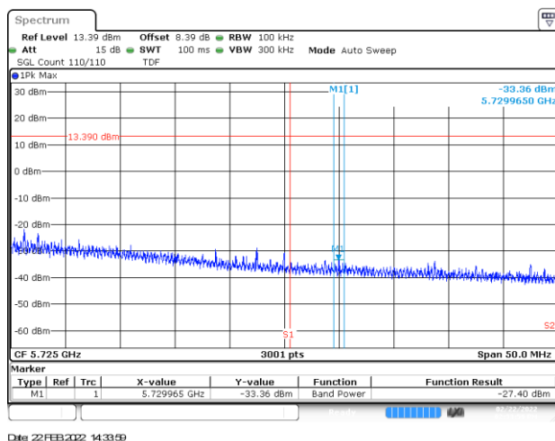
BE-NR-HIGH, SISO-A, 802.11n40-HT0, Ch134
