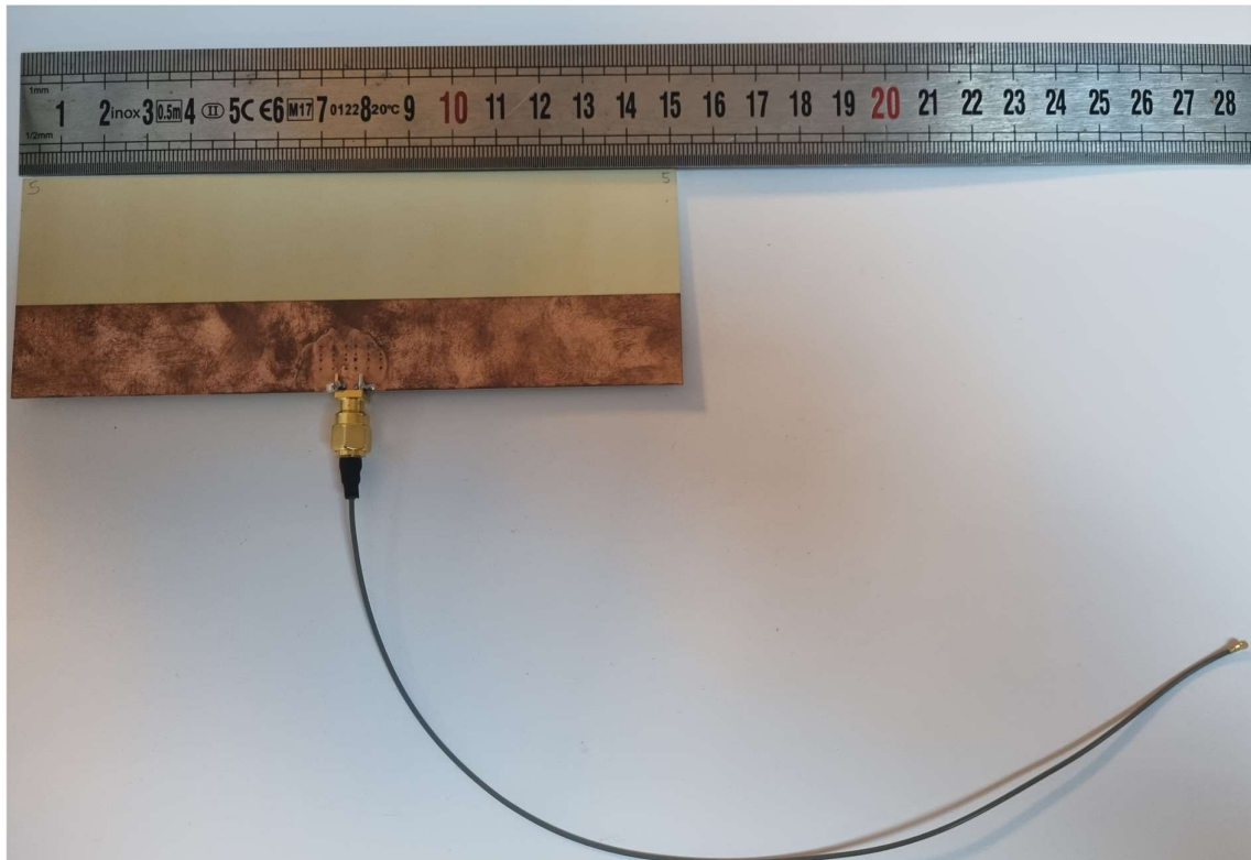
Back view
