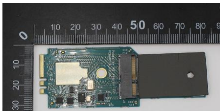
Extender board
