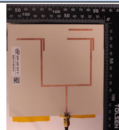
Antenna 2
