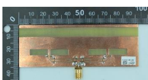
Antenna 1
