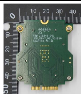
Adaptor back
