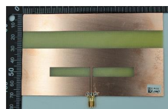
Antenna 2
