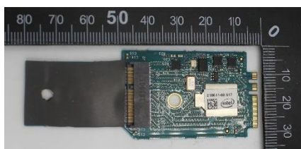
Extender board
