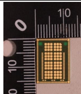
Socket back
