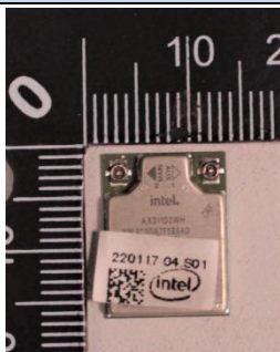
Socket front
