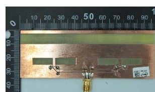
Antenna 2
