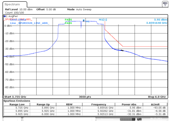
BE-NR-HIGH, SISO-A, 802.11ac80-VHT0, Ch171
