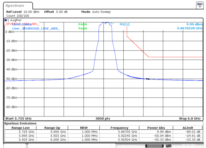
BE-NR-HIGH, SISO-A, 802.11n20-HT0, Ch173
