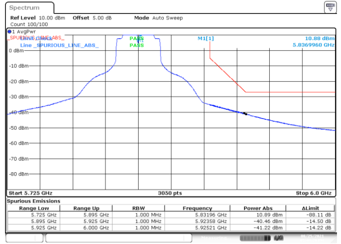
BE-NR-HIGH, SISO-A, 802.11n40-HT0, Ch167
