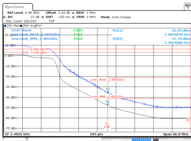
BE-R-HIGH, SISO-A, 802.11n40-HT0, Ch10
