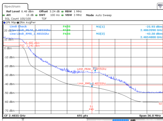
BE-R-HIGH, SISO-A, 802.11n40-HT0, Ch9
