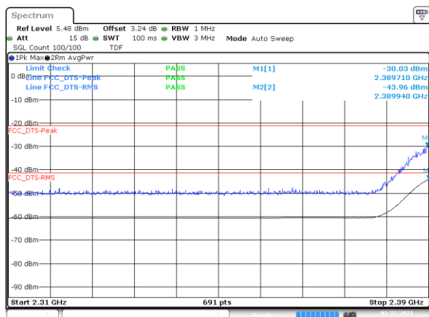
BE-R-LOW, SISO-A, 802.11g-6Mbps, Ch1
