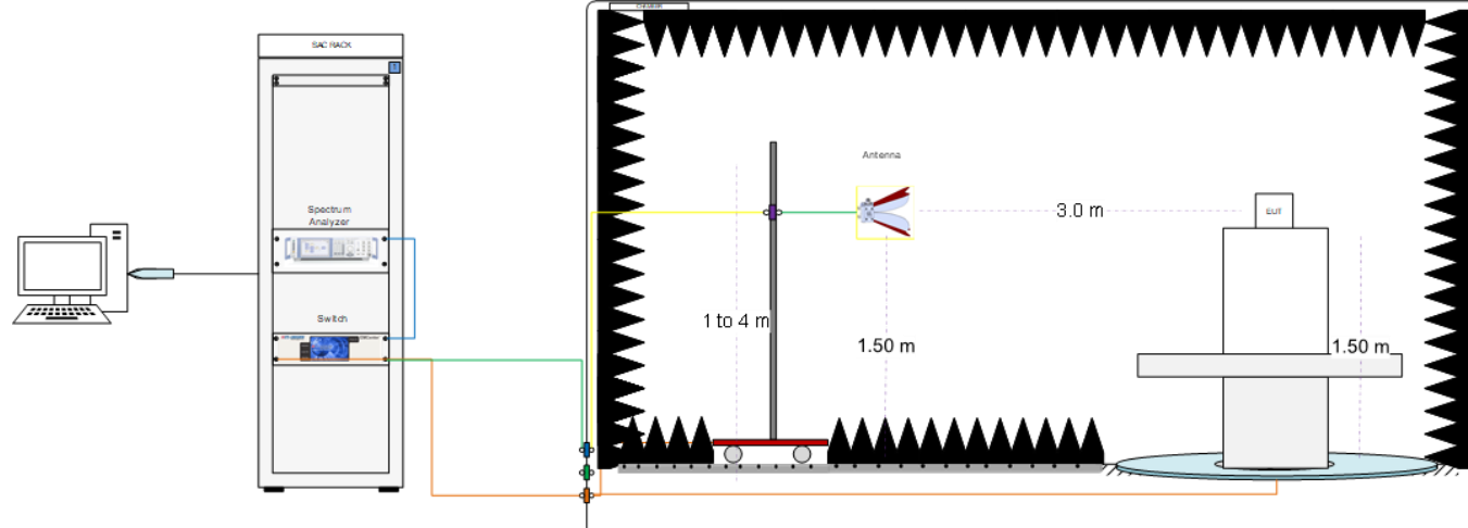
Radiated Setup 1 GHz – 6.4 GHz
