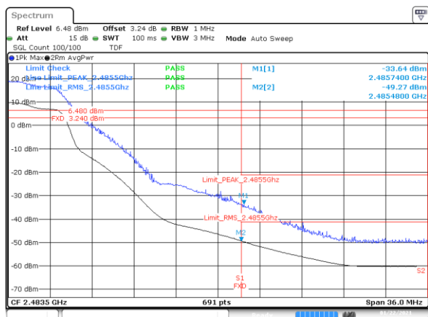
BE-R-HIGH, SISO-A, 802.11g-6Mbps, Ch11
