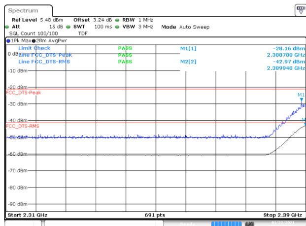
BE-R-LOW, SISO-A, 802.11n40-HT0, Ch3
