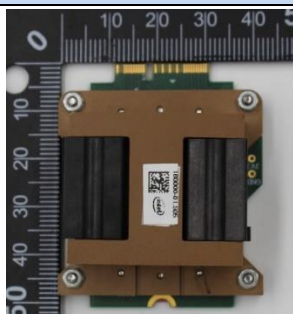
Extender board
