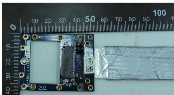
Antenna 1
