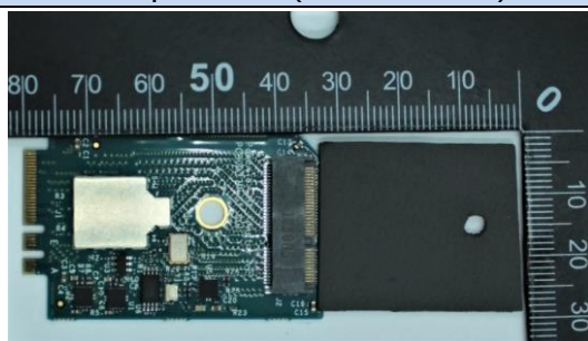
Extender board
