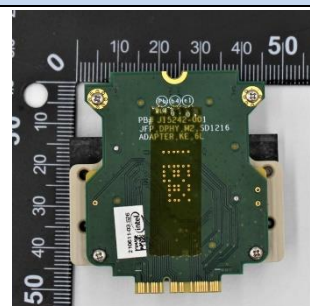
Adaptor back
