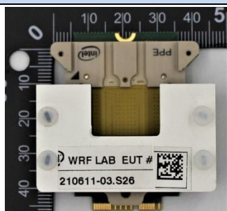
Adaptor front (with absorber)
