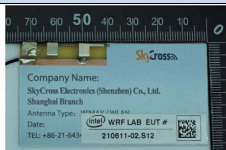
Aux Antenna
