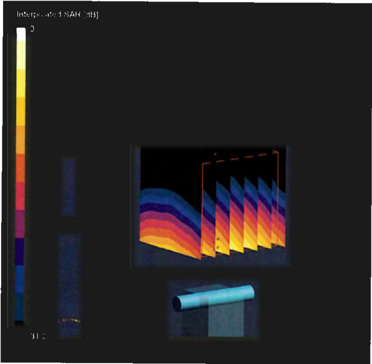
0 dB – 37.3 W/Kg
