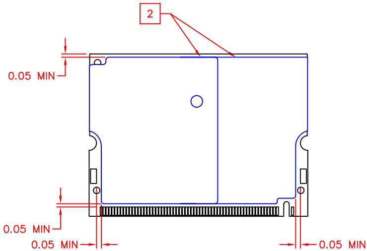
SECONDARY SIDE INSULATION PLACEMENT STEP 3
