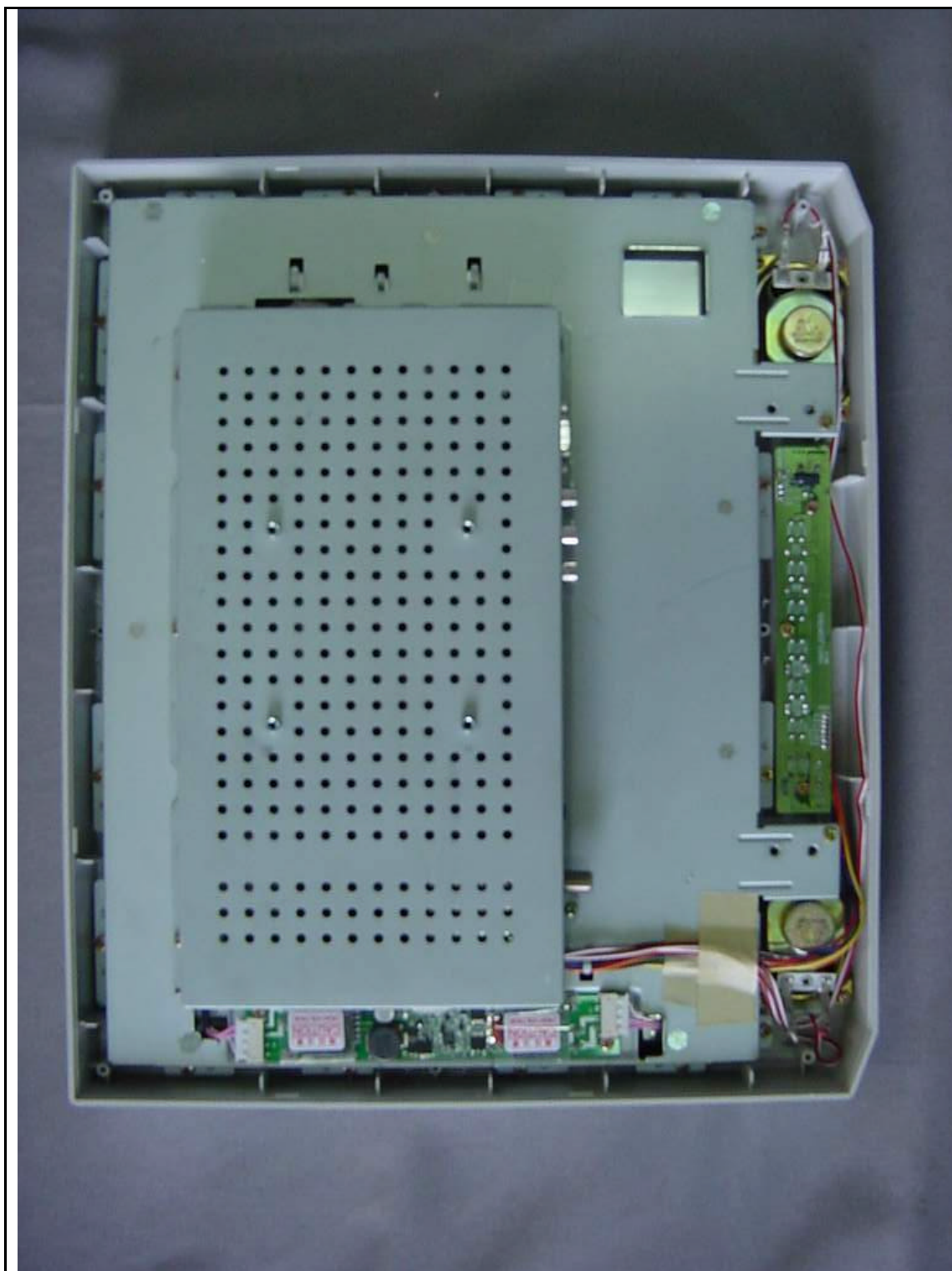
[ Inside View of the LCD Panel ]
