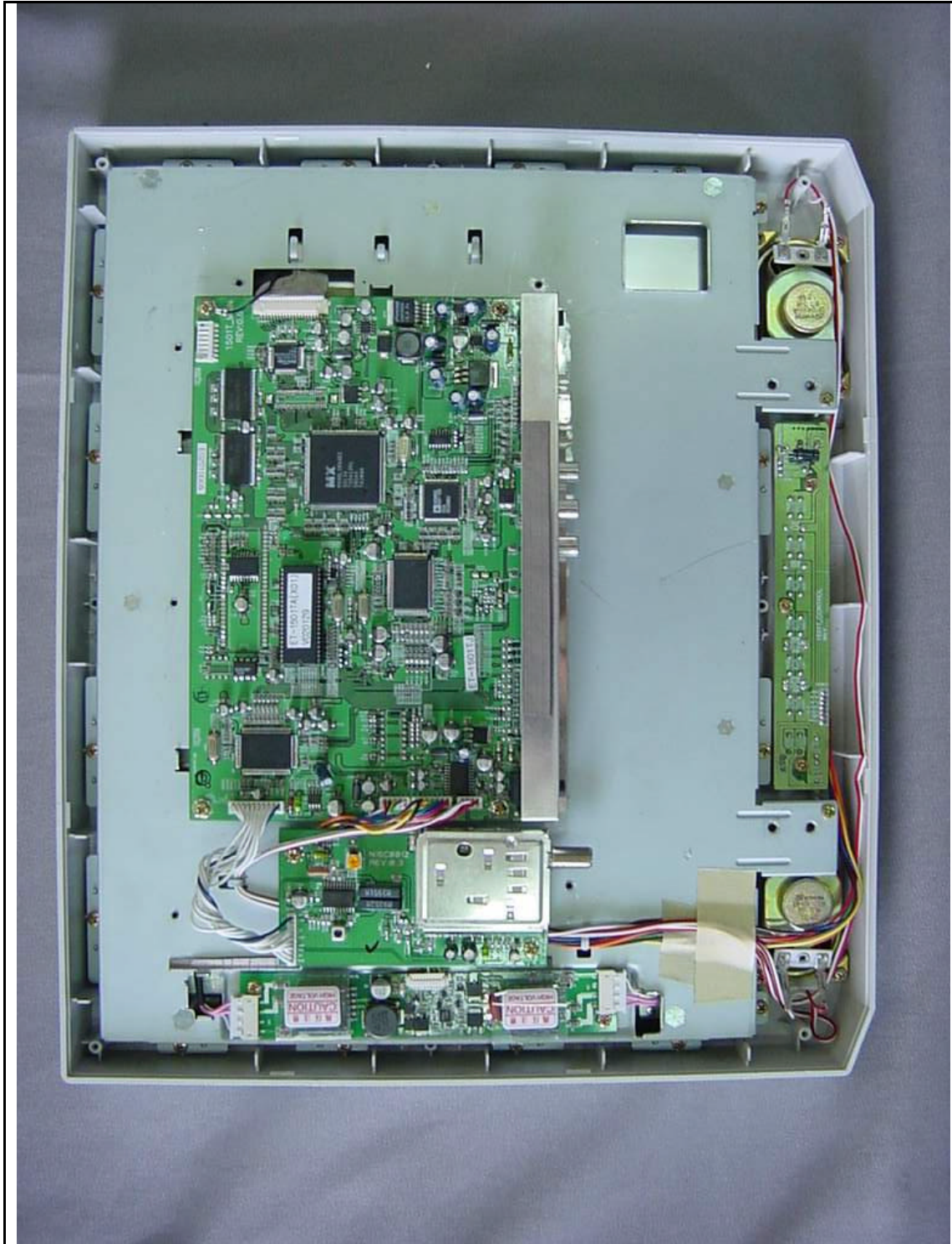
[ Inside View after Open Shield Cover of the LCD Panel]
