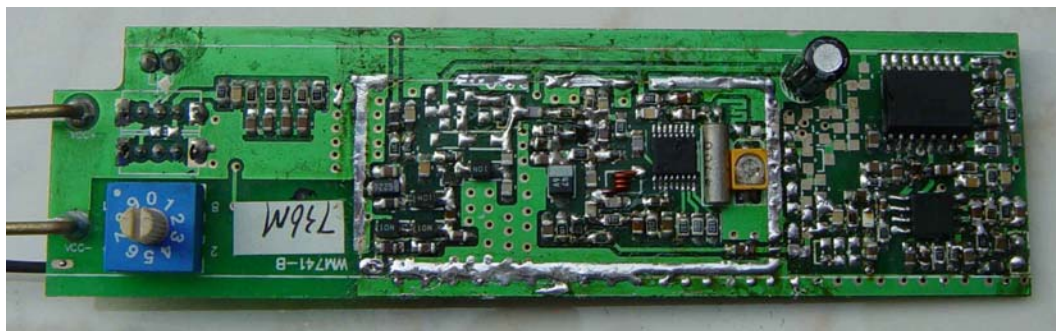
(4) Main board solder side
