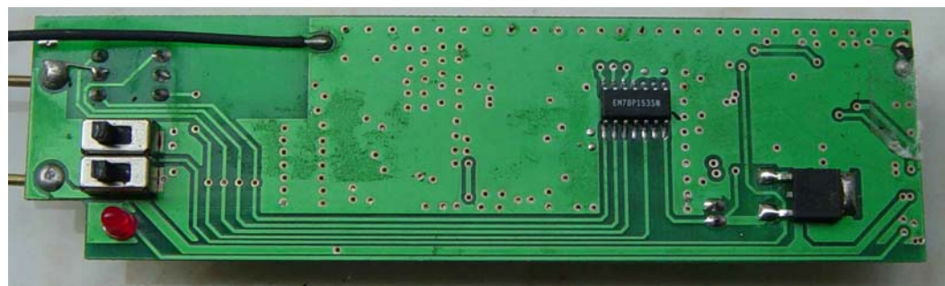
(4) Main board solder side
