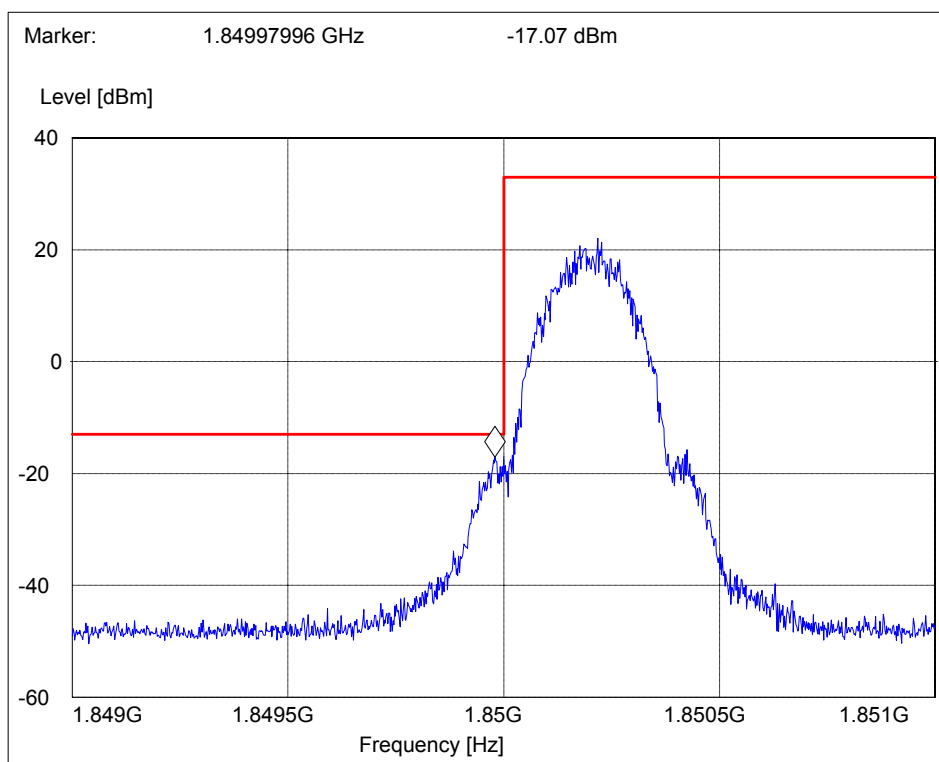
Picture 1 Lower bandedge, channel 512, GSM
