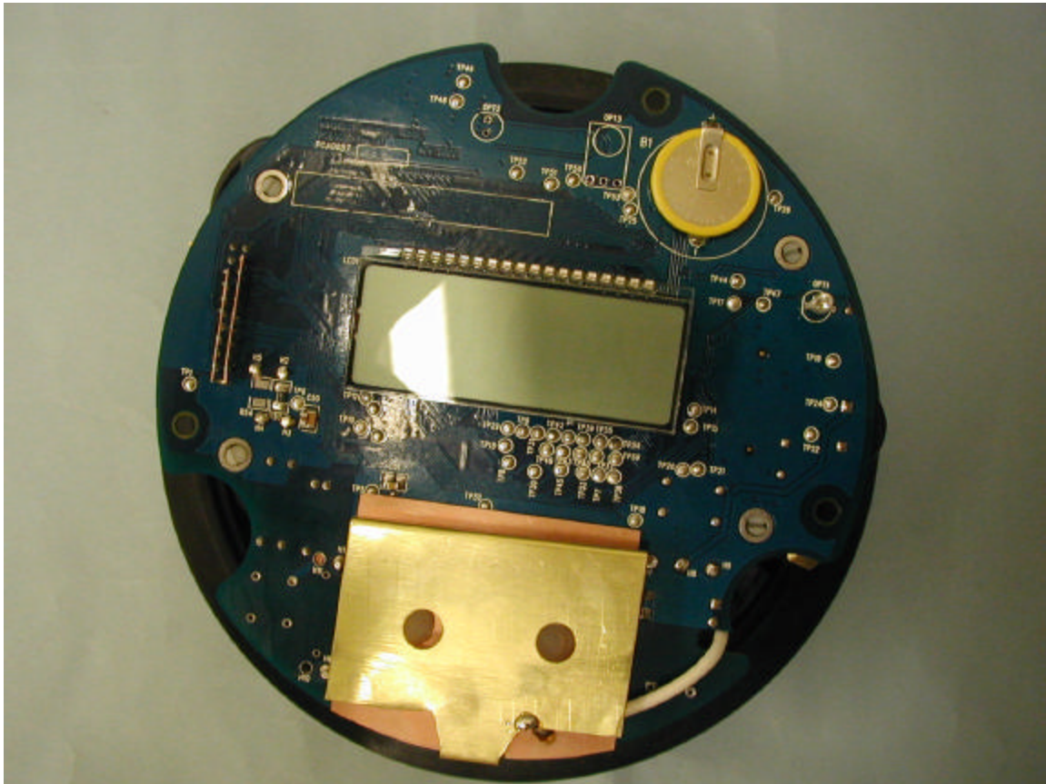
Internal Layout of Meter
