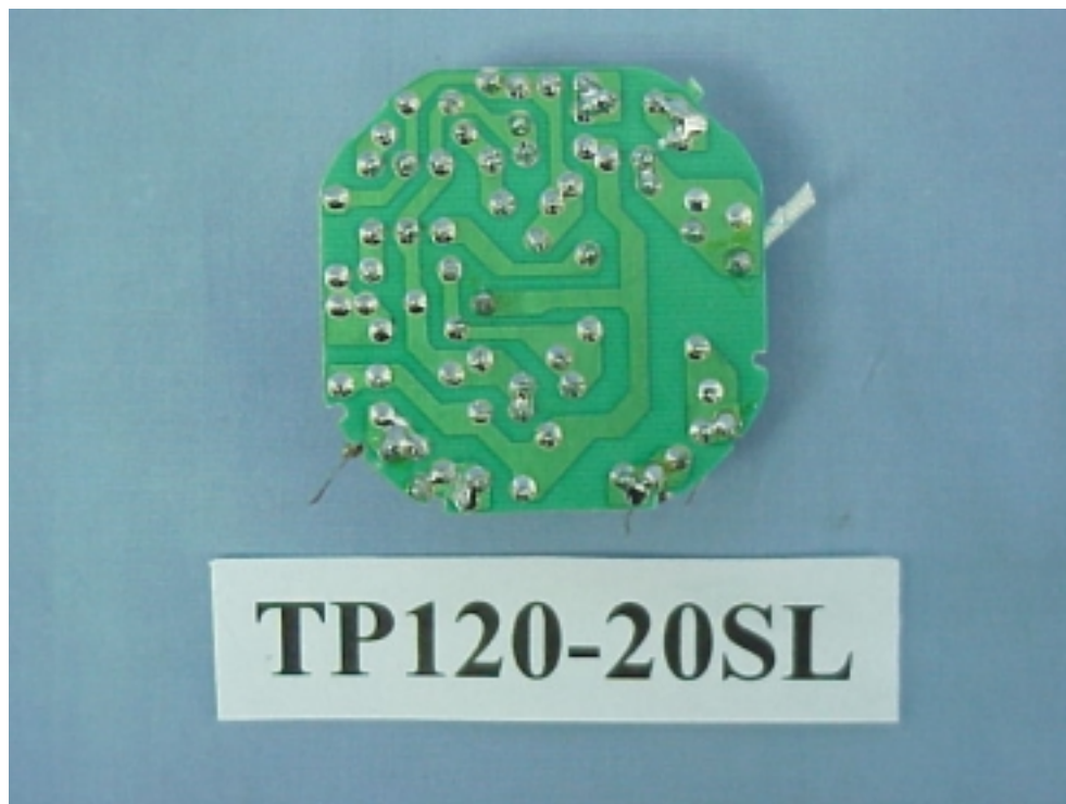
Figure 10 Compact Fluorescent Lamp (M/N: TP120-20SL) Main Board (Soldered Side)
