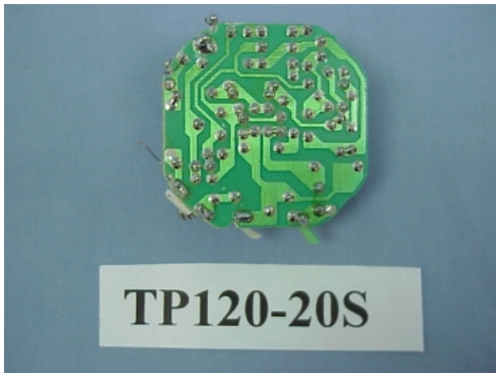
Figure 4 Compact Fluorescent Lamp (M/N: TP120-20S) Main Board (Soldered Side)
