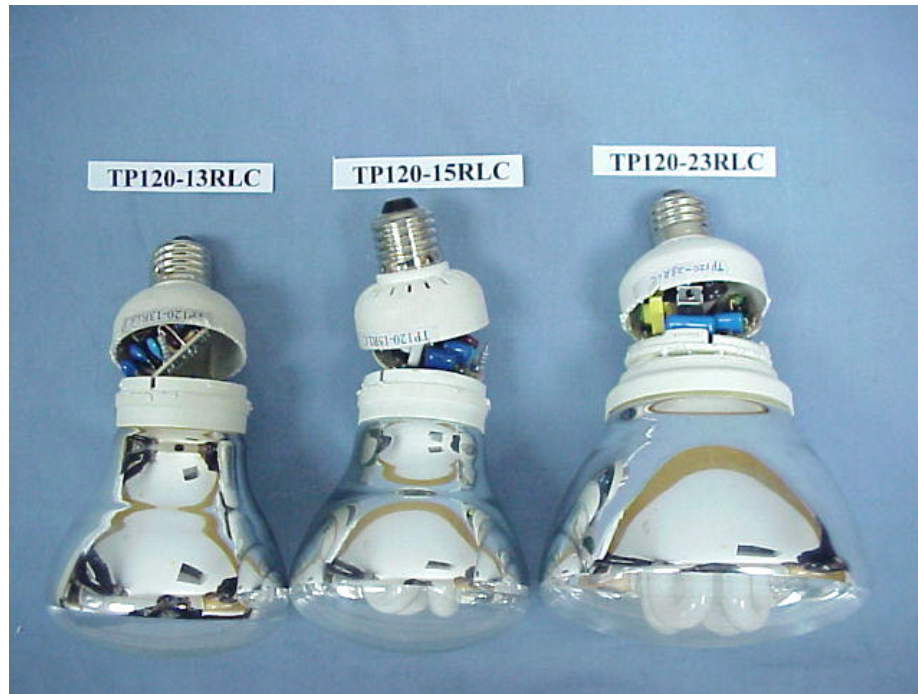
Figure 4. Compact Fluorescent Lamp (M/N: TP120-RLC Series) Cover Removed
