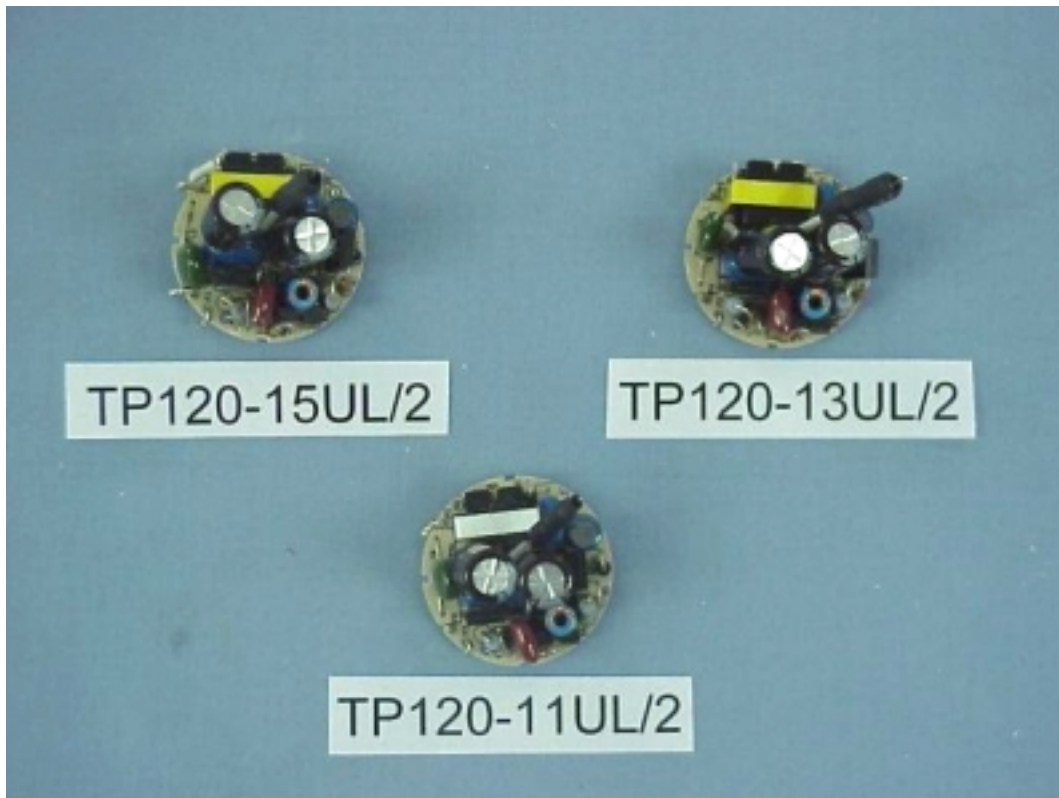
FIGURE 5 ENERGY SAVING LAMP (M/N: TP120-11UL/2, -13UL/2, -15UL/2) MAIN BOARD (COMPONENT SIDE)
