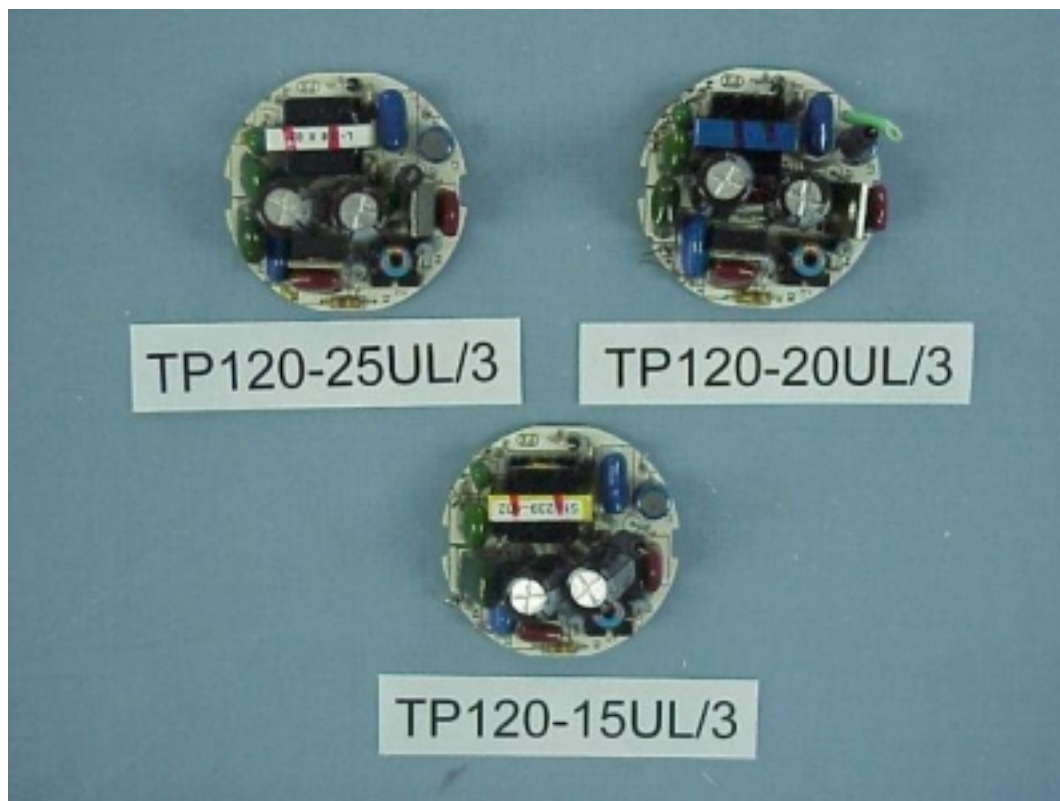
FIGURE 8 ENERGY SAVING LAMP (M/N: TP120-15UL/3, -20UL/3, -25UL/3) MAIN BOARD (COMPONENT SIDE)
