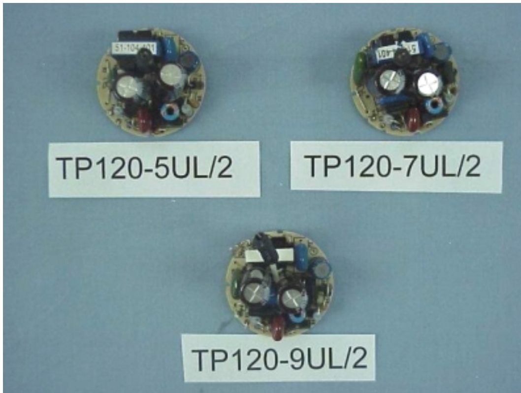
FIGURE 2 ENERGY SAVING LAMP (M/N: TP120-5UL/2, -7UL/2, -9UL/2) MAIN BOARD (COMPONENT SIDE)
