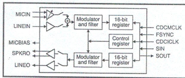
IBM3920 CODEC Block Diagram
