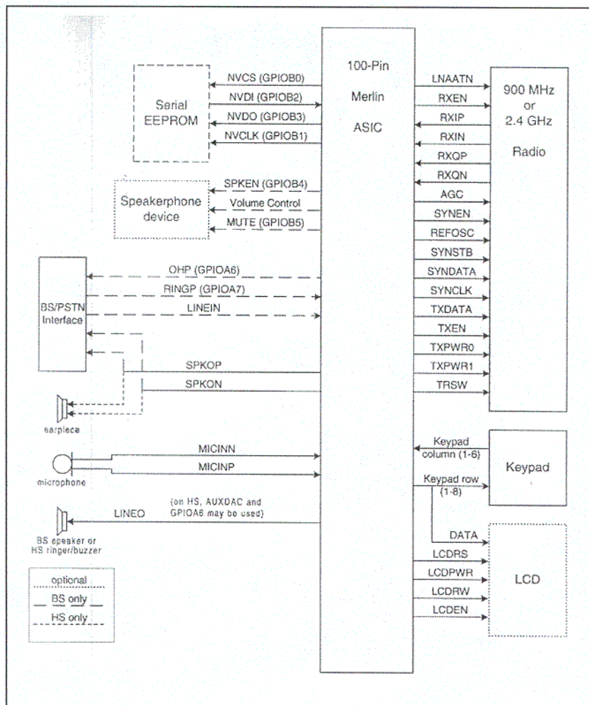
IBM3920 System Block Diagram
