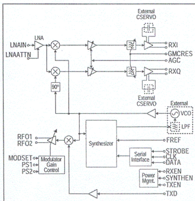
IBM3920 RF Block Diagram
