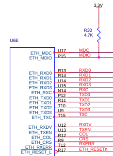
AR2315 MII Interface
