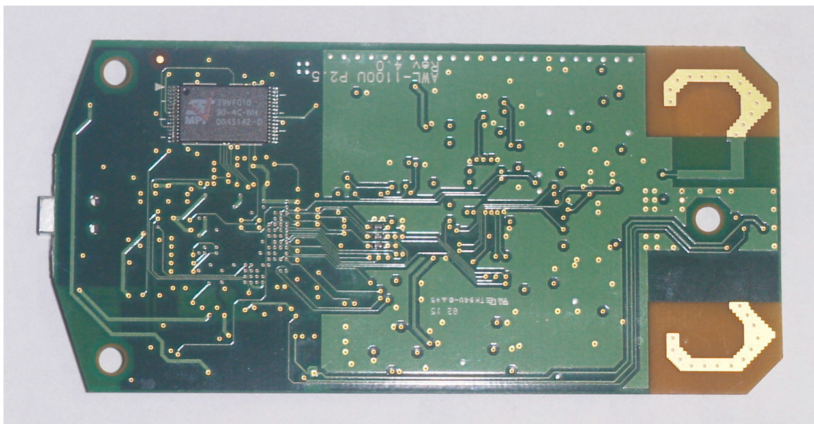
8.4 PBA Bottom View
