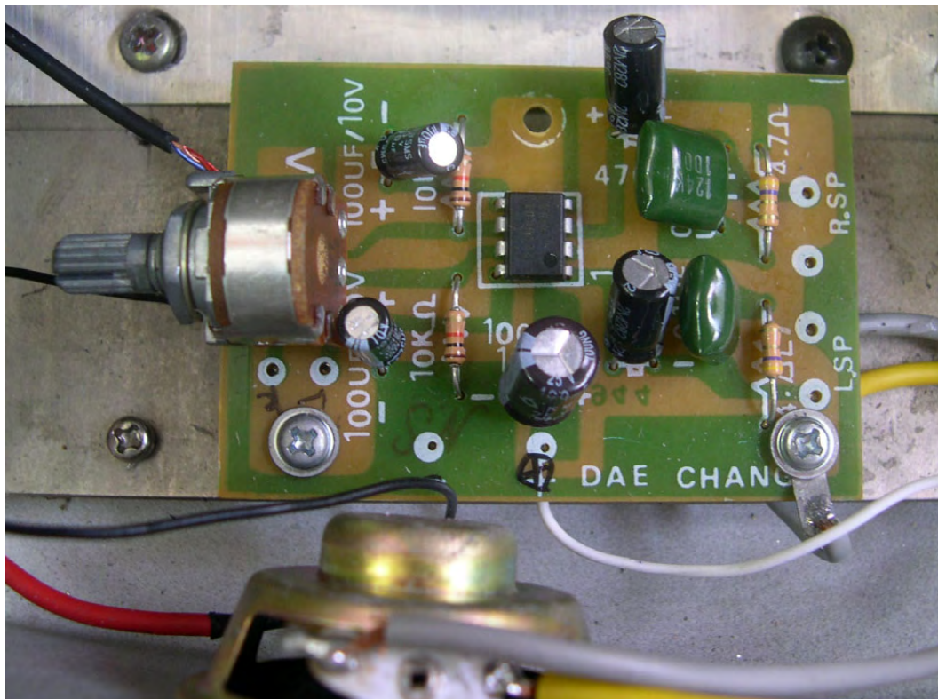
<Photograph 10: Audio board - Front View>
