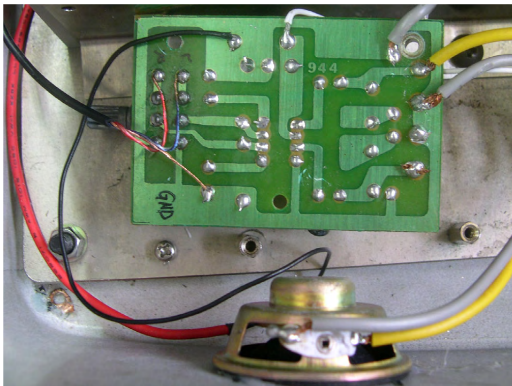
< Photograph 11: Audio board - Rear View >
