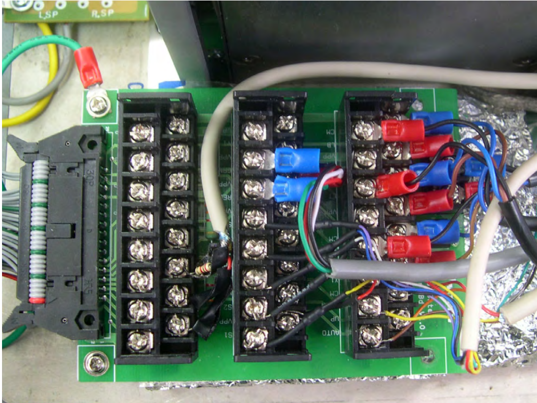
<Photograph 2: I/O board - Front View>
