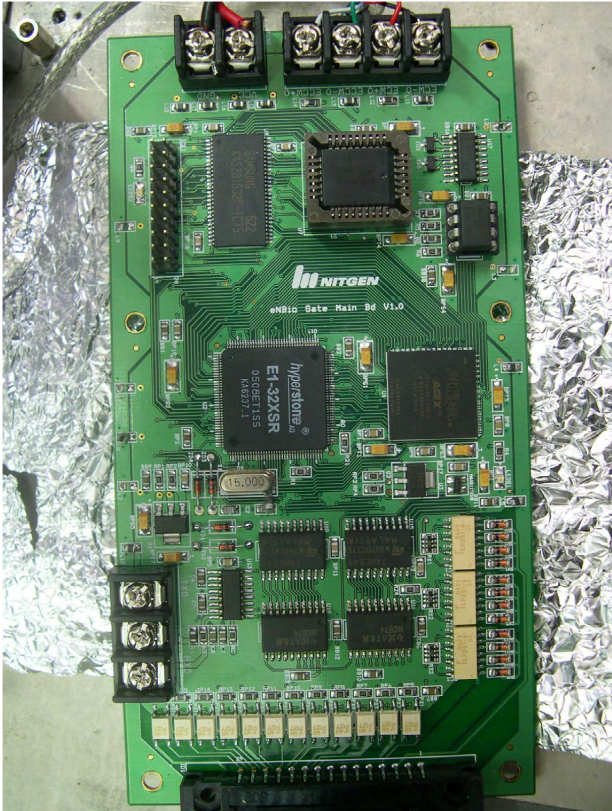
<Photograph 4: Main board - Front View>
