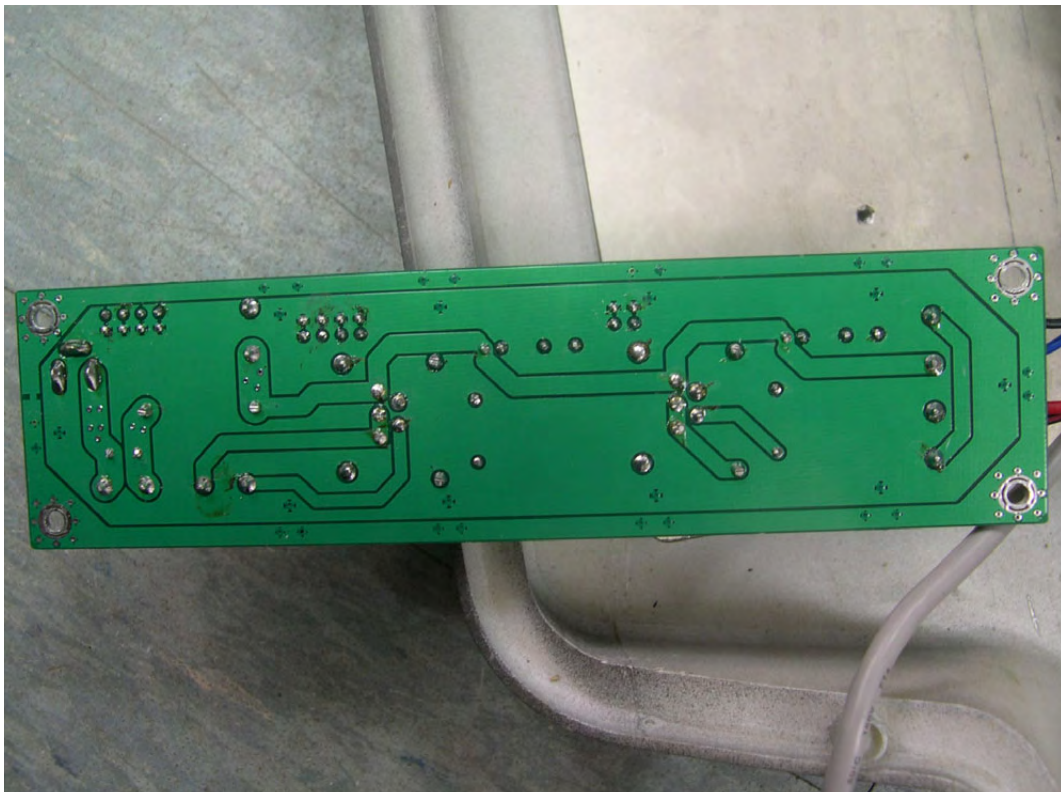
<Photograph 7: Power board - Rear View>
