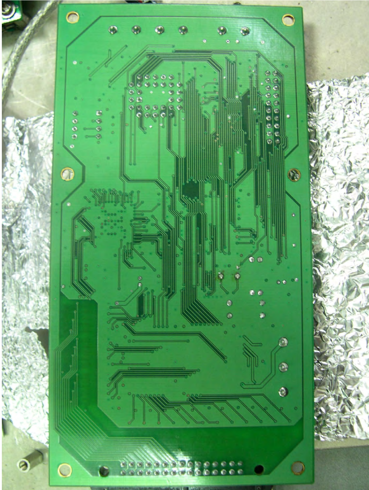
<Photograph 5: Main board - Rear View>
