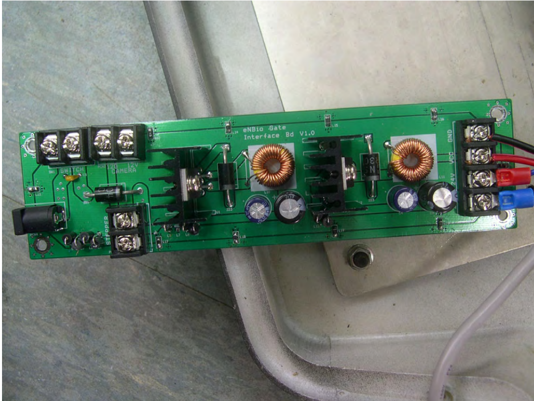
<Photograph 6: Power board - Front View>
