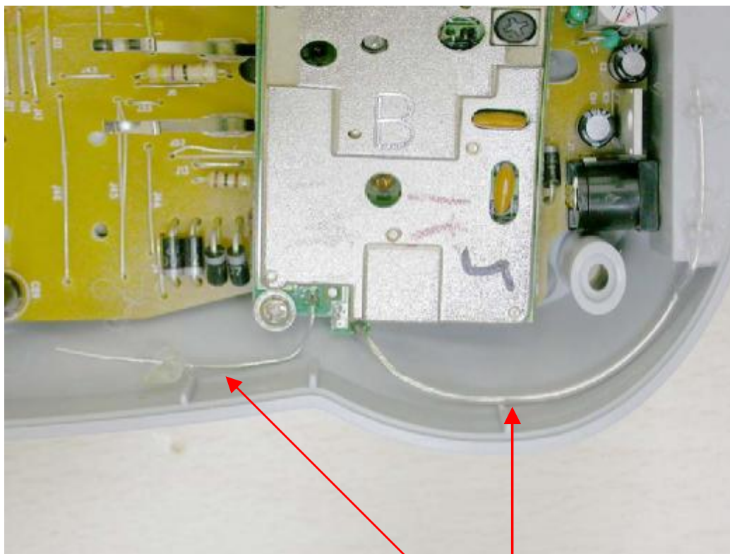
Photo 4: External photo of Antenna
